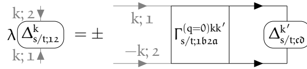
FIGURE 3.18 – Linearized Eliashberg equation for vanishing transfer frequency q = 0 , see Eq. (3.136).
