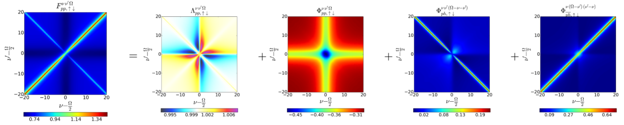
FIGURE 3.14 – Numerical SIAM results for all local vertices contained in the parquet equation Eq. (3.33) for vanishing transfer frequency \Omega = 0 , taken from Ref. [Wentzell2020]. In our convention, \Omega should be replaced by \omega .
