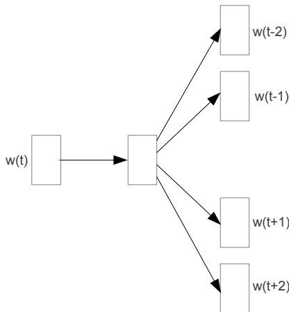
Skip-gram
