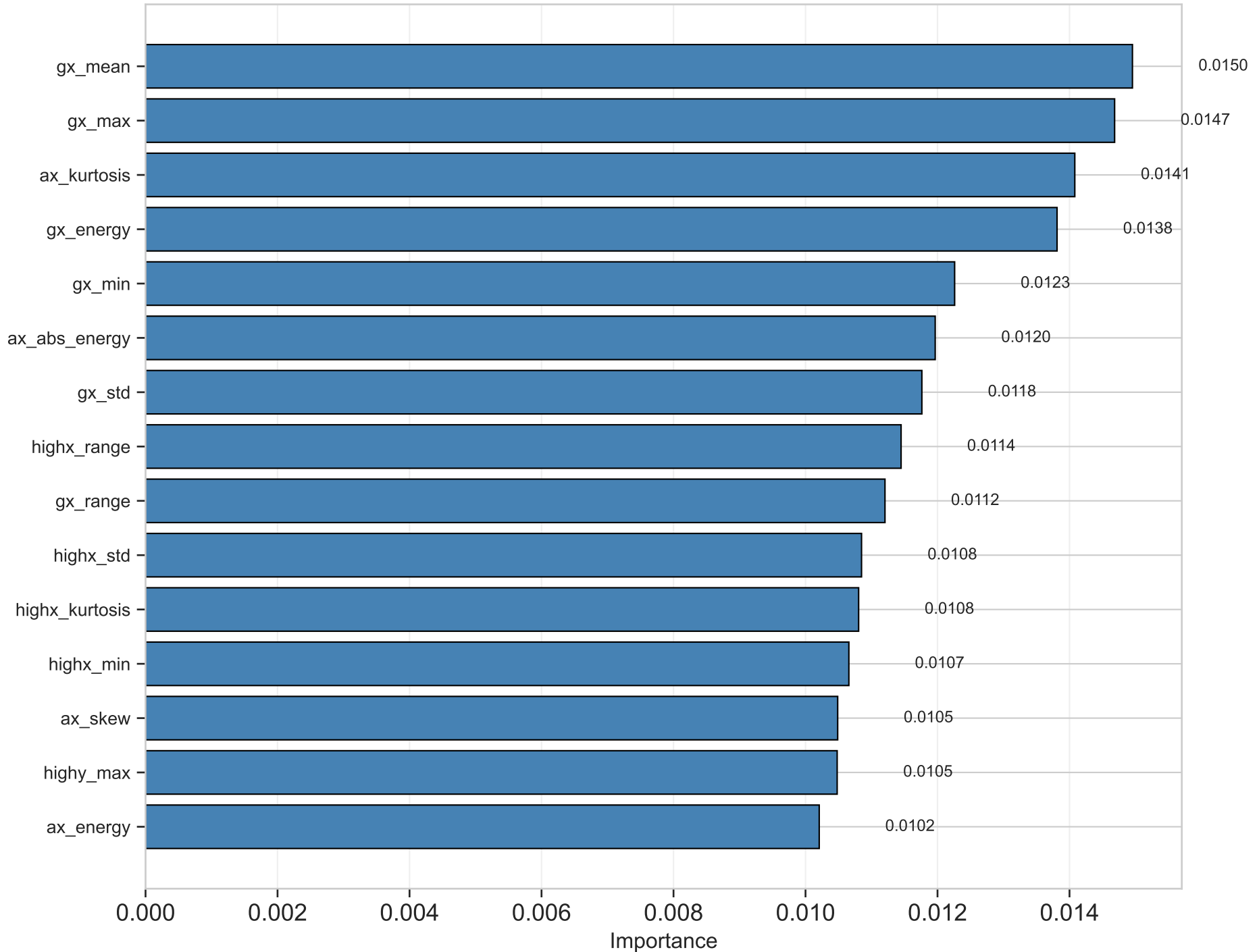
Top 15 Feature Importances (Random Forest)
