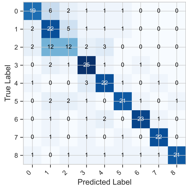
DTW + KNN
