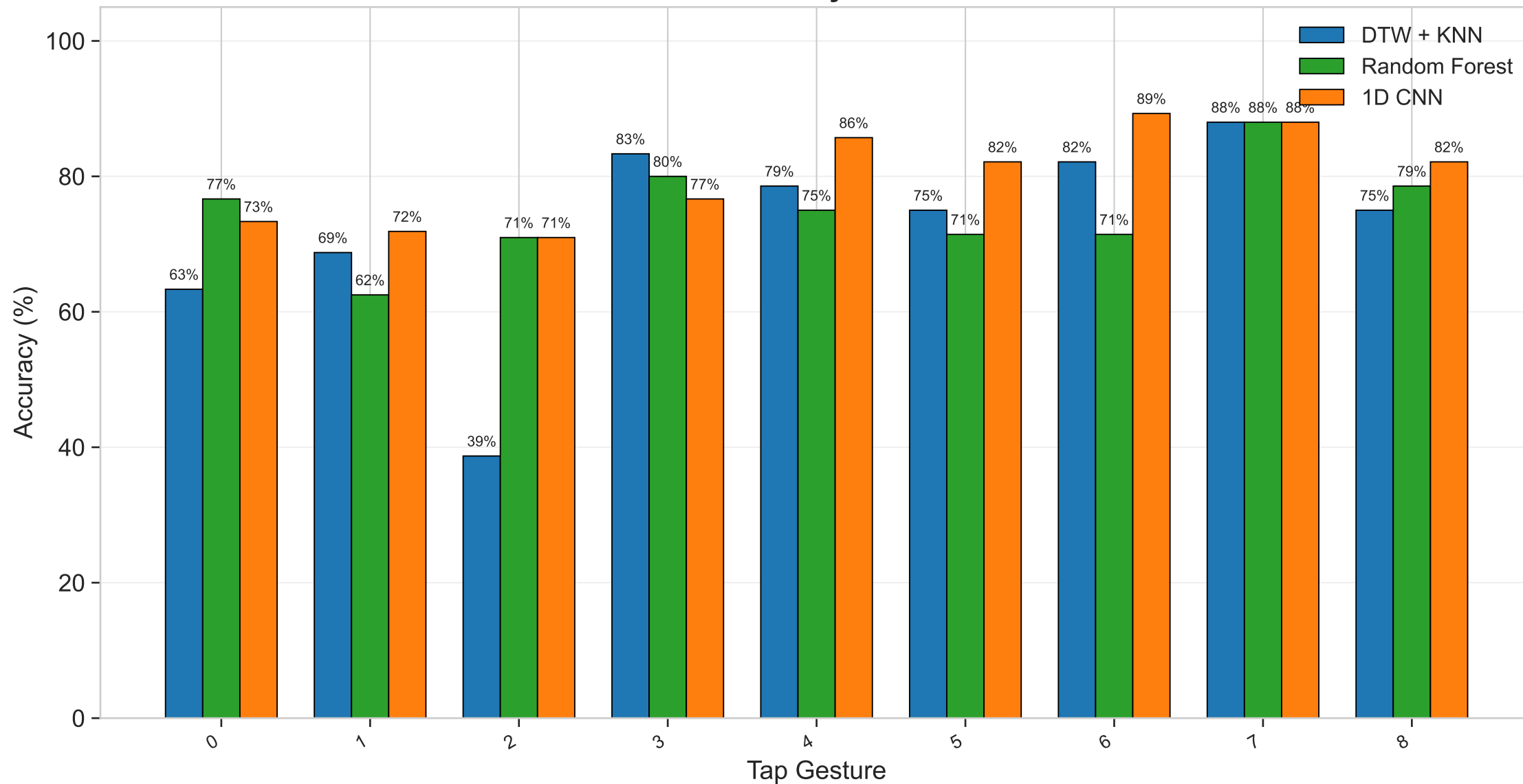
Per-Class Accuracy Across Models
