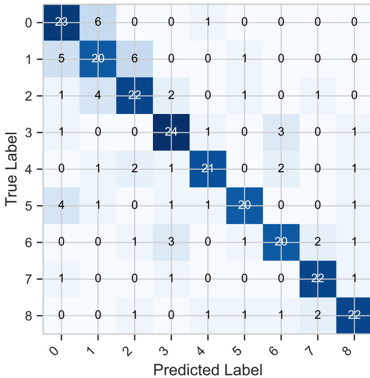
Random Forest
