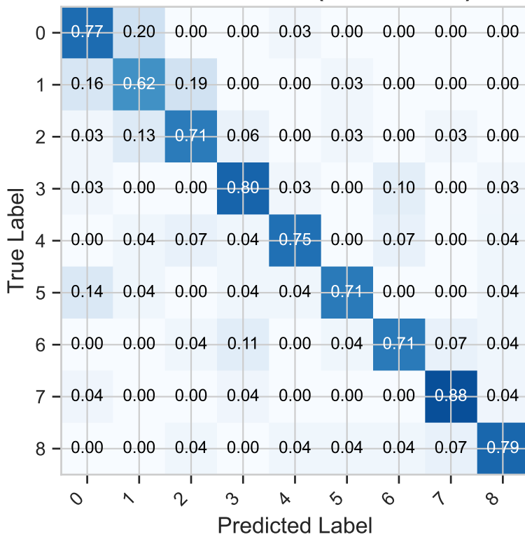
Random Forest (Normalized)
