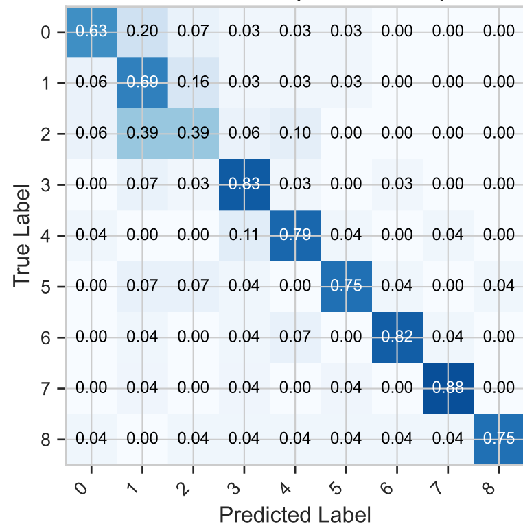
DTW + KNN (Normalized)
