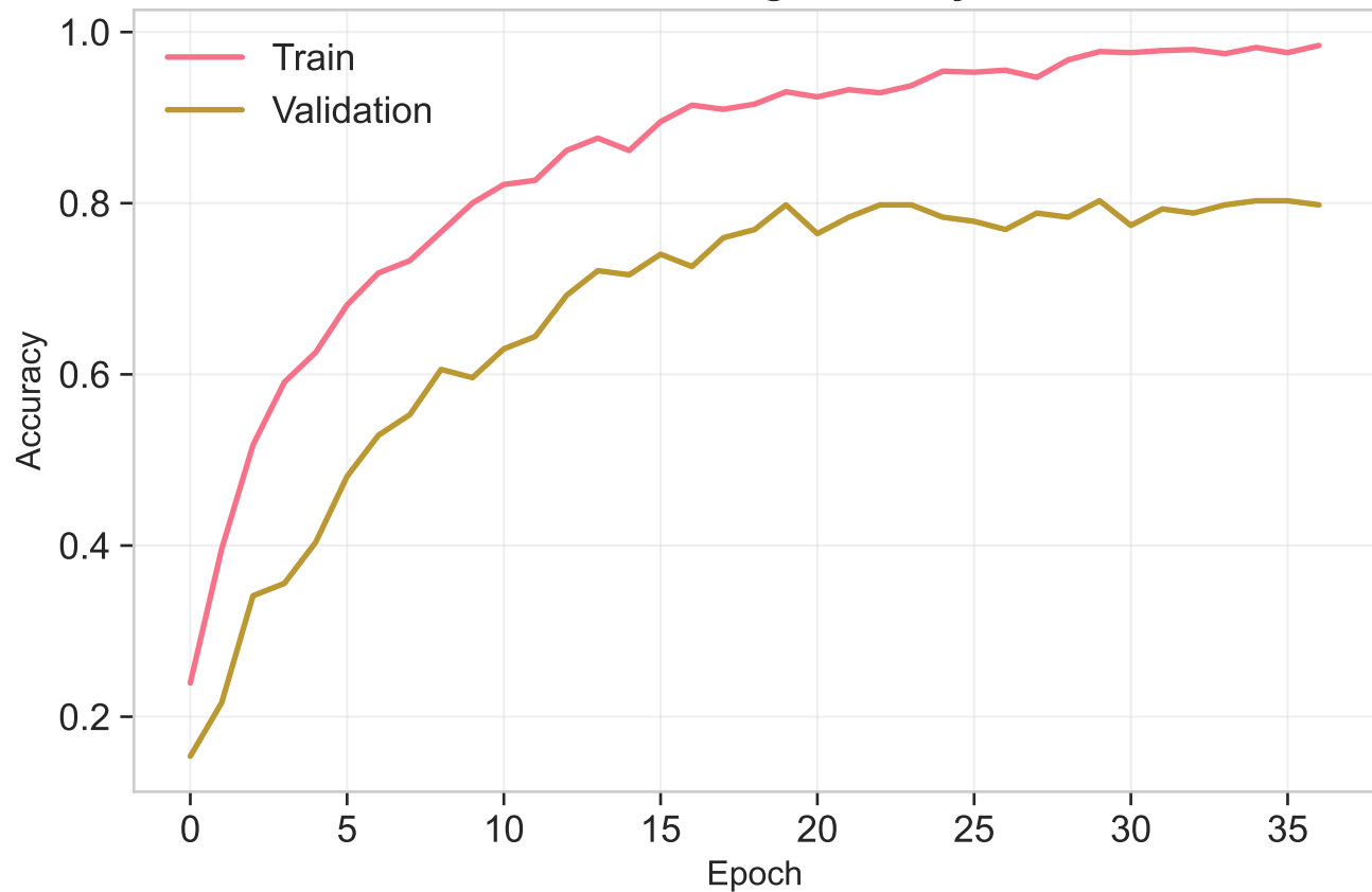
CNN Training Accuracy
