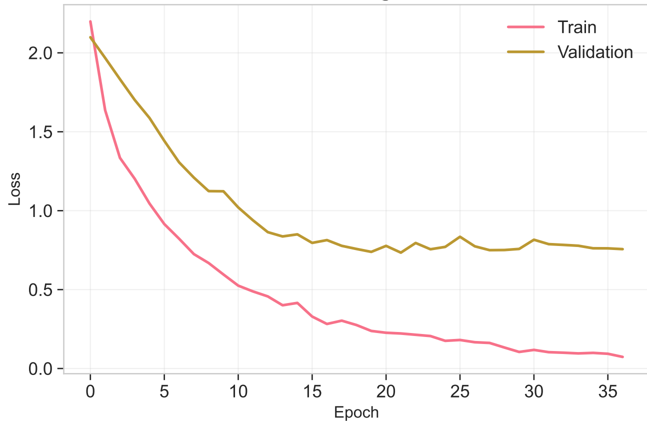
CNN Training Loss
