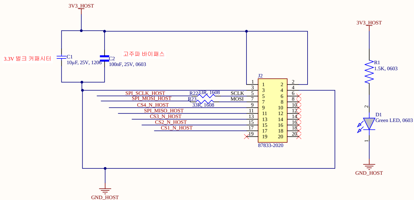
J2 – CARRIER BOARD INTERFACE
