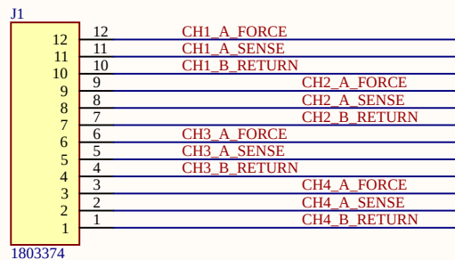
PT100 Sensor Input
