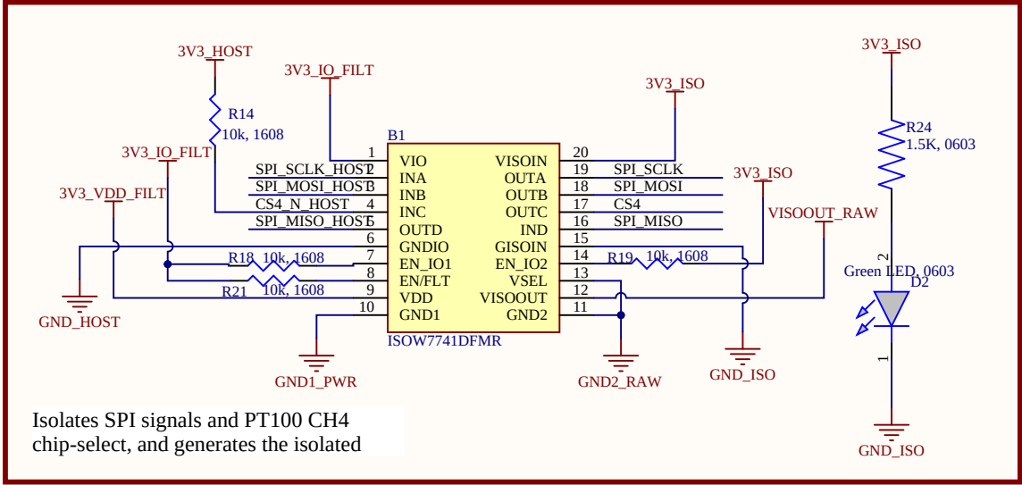
SPI BUS & CS4 ISOLATION / ISOLATED POWER
