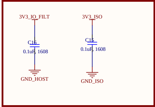
B2 SUPPLY DECOUPLING
