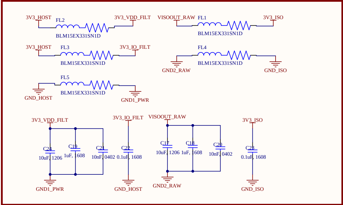
POWER/GROUND FILTERING & DECOUPLING
