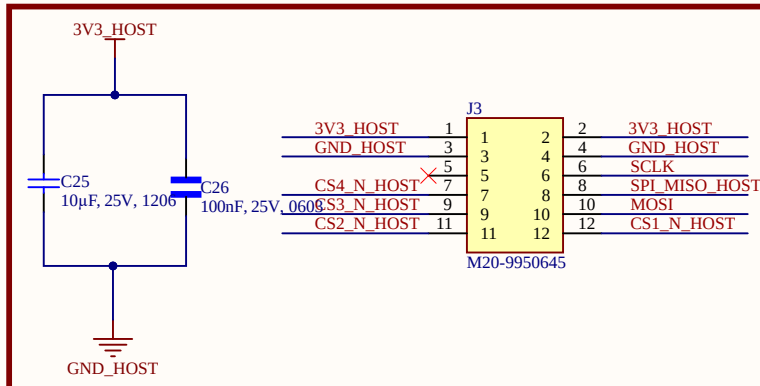
J3 – ZYBO PMOD INTERFACE
