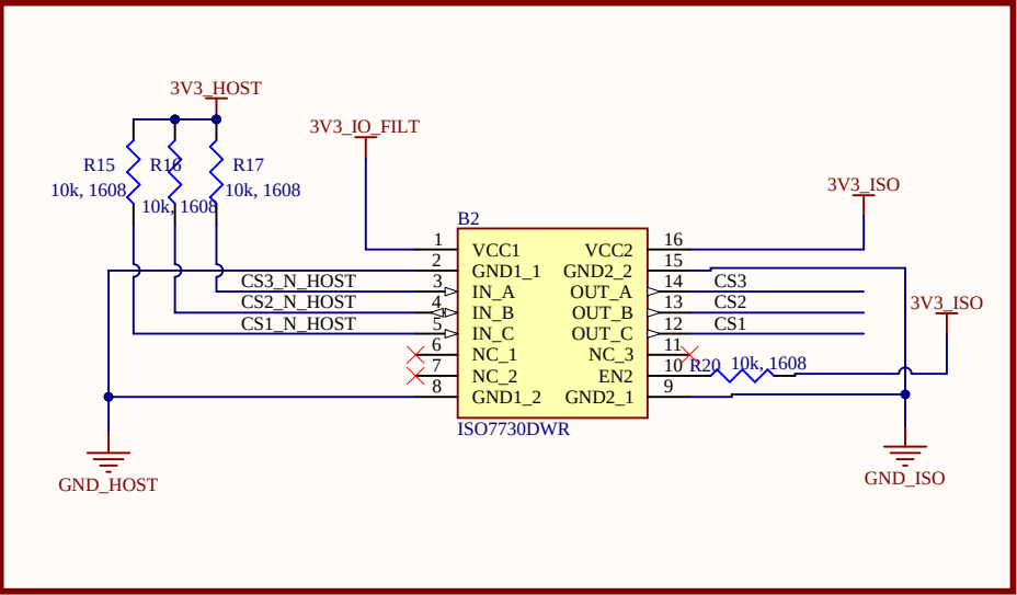
CH1-CH3 CHIP-SELECT ISOLATION
