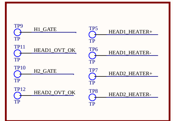
SIGNAL TEST POINTS
