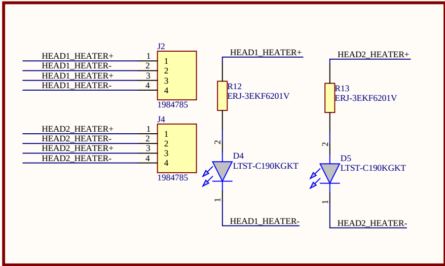
HEATER OUTPUT & STATUS LED
