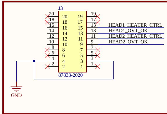
CONTROL SIGNAL INTERFACE
