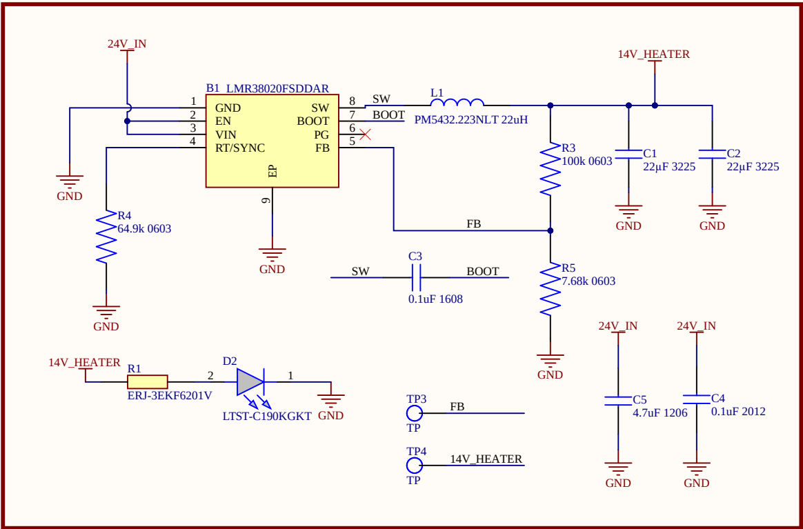
24V-to-14V Heater Buck Converter
