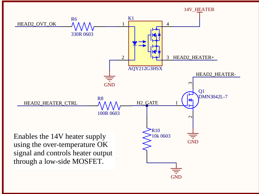
HEATER CH2 OUTPUT CONTROL
