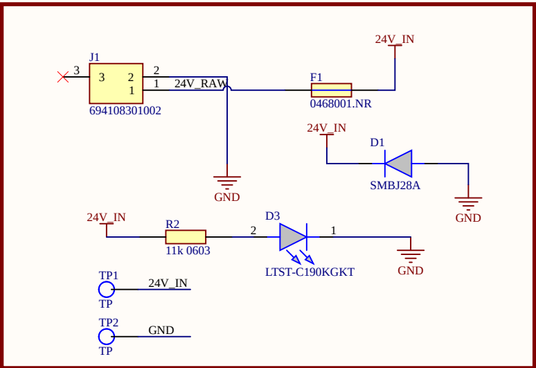
24V Power Input & Protection
