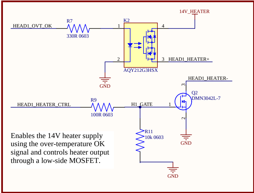
HEATER CH1 OUTPUT CONTROL
