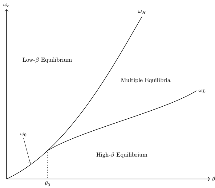
Figure 3: Equilibrium Characterization
