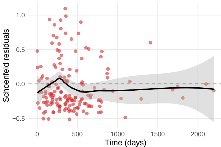
LEFTY1 (p = 0.5981)
