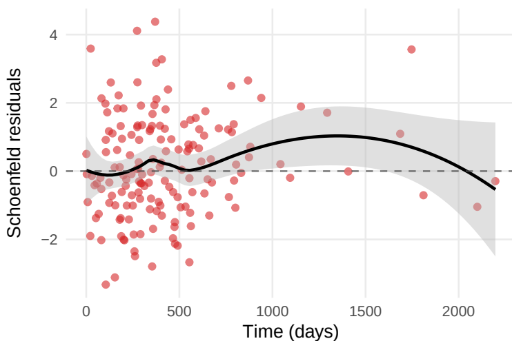
LEFTY1 (p = 0.5981)
