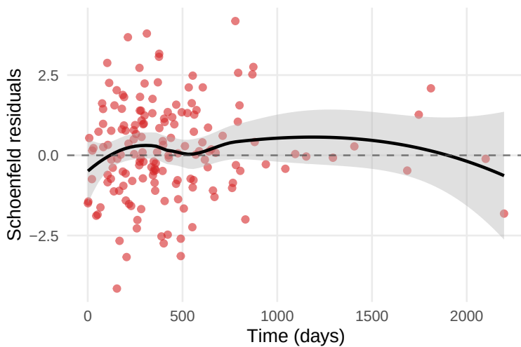
CPQ (p = 0.339)
