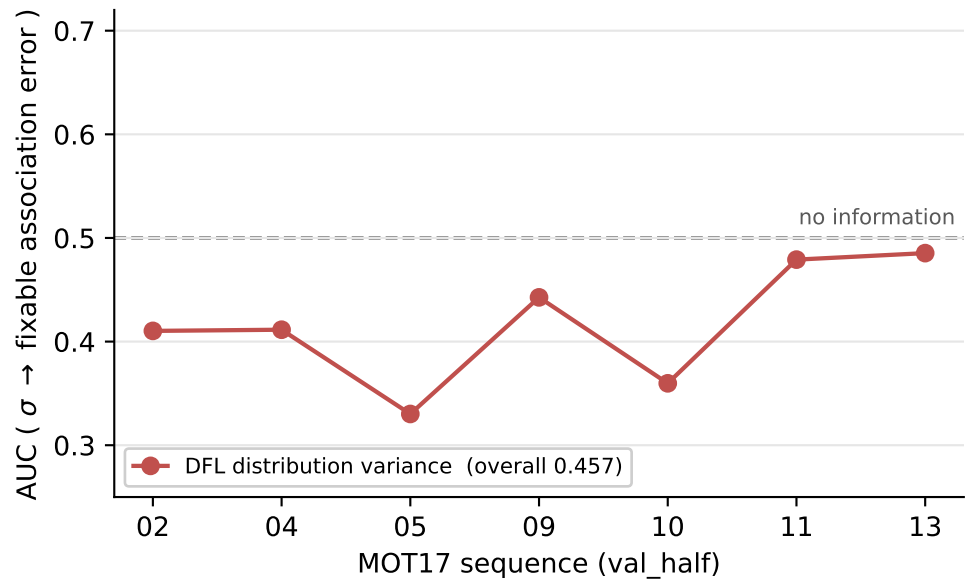
(b) Association error \sigma does not rank which match is wrong
