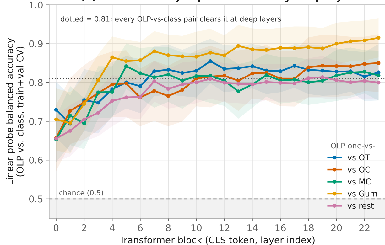
(a) OLP is linearly separable at every deep layer
