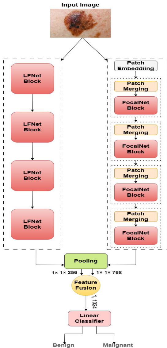
FIGURE 6. Detailed architecture of FoMoSkinNet.
