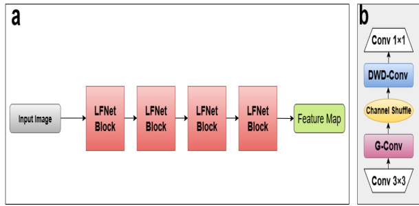
FIGURE 9. (a) Overview of LFNet pipeline, and (b) Structure of a LFNet block.
