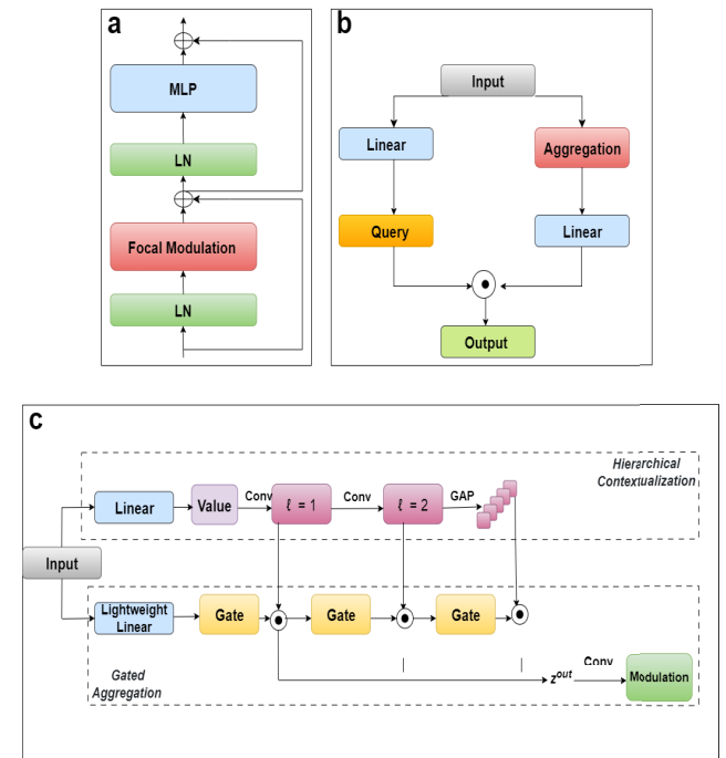
FIGURE 8. Structure of main FocalNetBlock and its parts: (a) FocalNetBlock, (b) Modulation unit and (c) Context aggregation.
