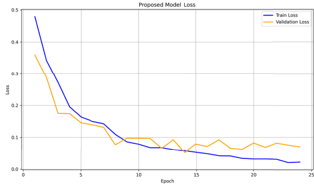
FIGURE 15. Training and validation loss of FoMoSkinNet.
