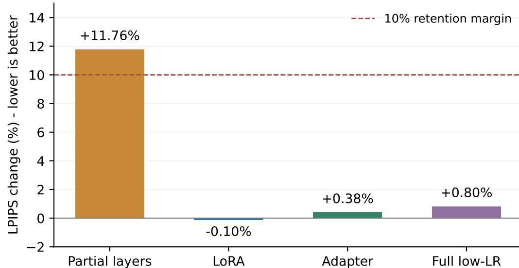
Future-video error change from Stage1
