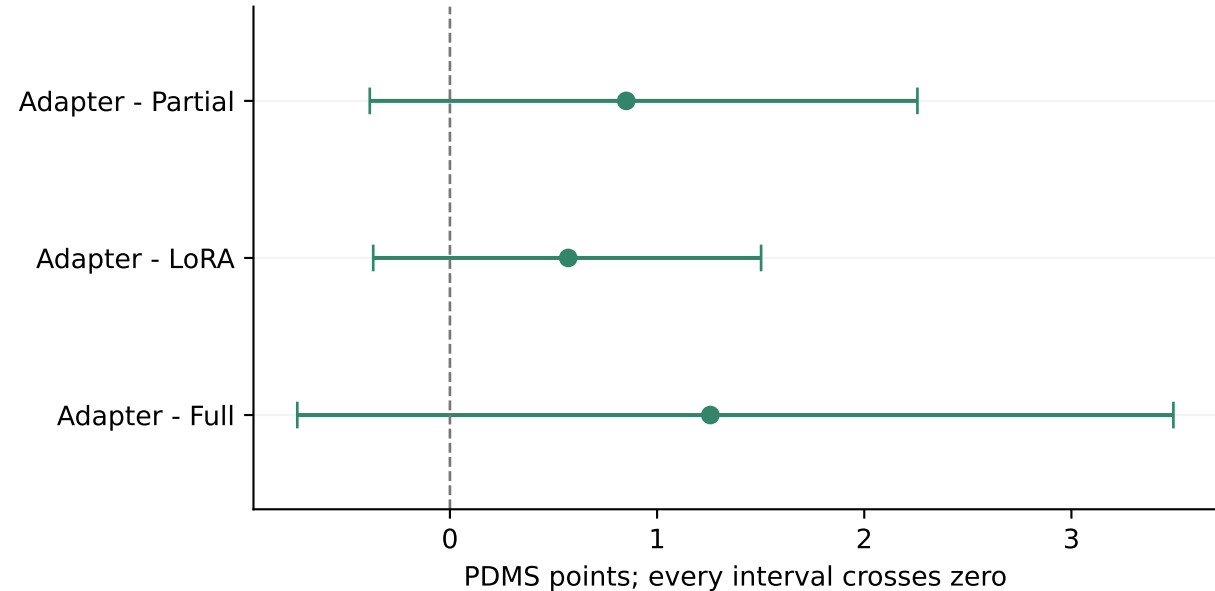
PDMS differences: paired 95% intervals
