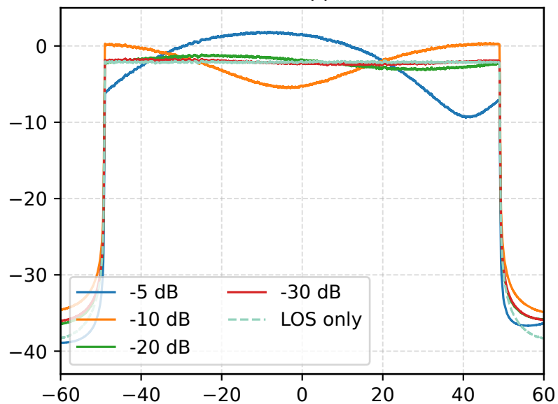
(b) Received ripple at 10 ns
