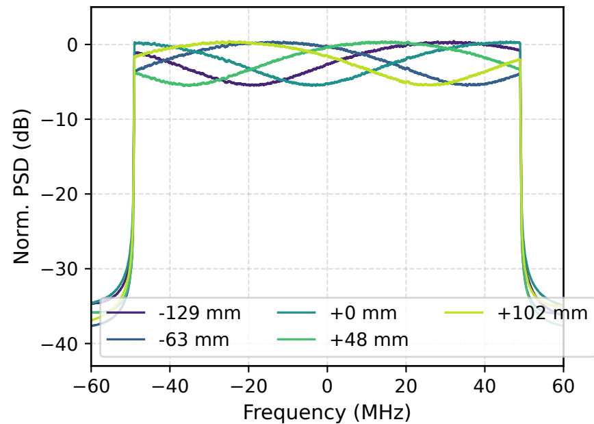
(c) Multi-point spectra, est. -10.00 dB / 10.00 ns
