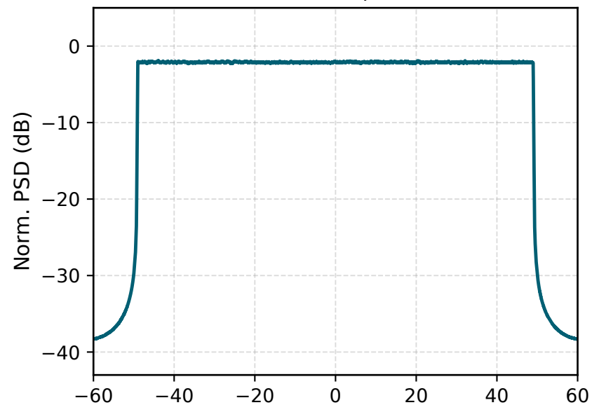
(a) Transmit spectrum
