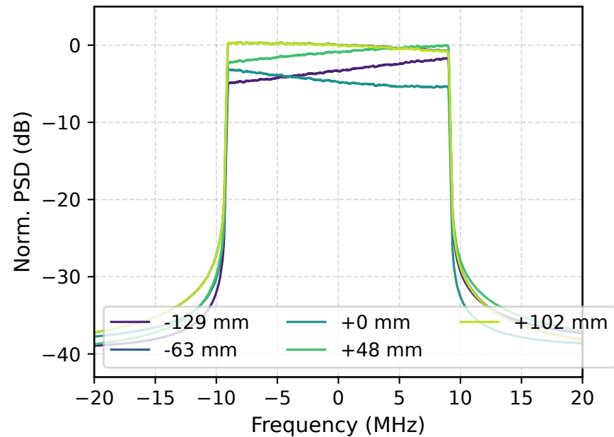
(c) Multi-point spectra, est. -9.93 dB / 9.81 ns
