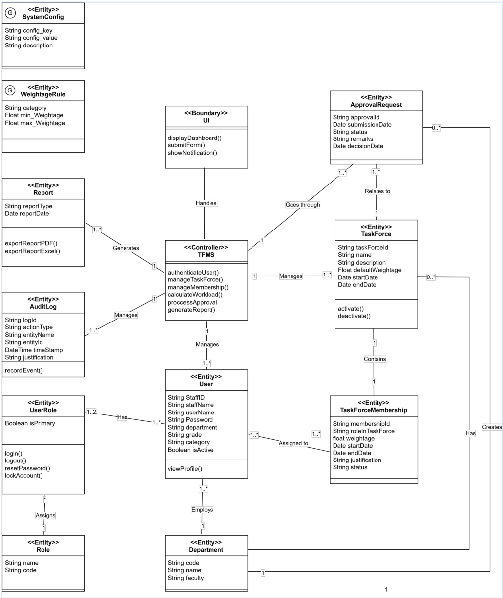
Figure 9: Class Diagram of TFMS
