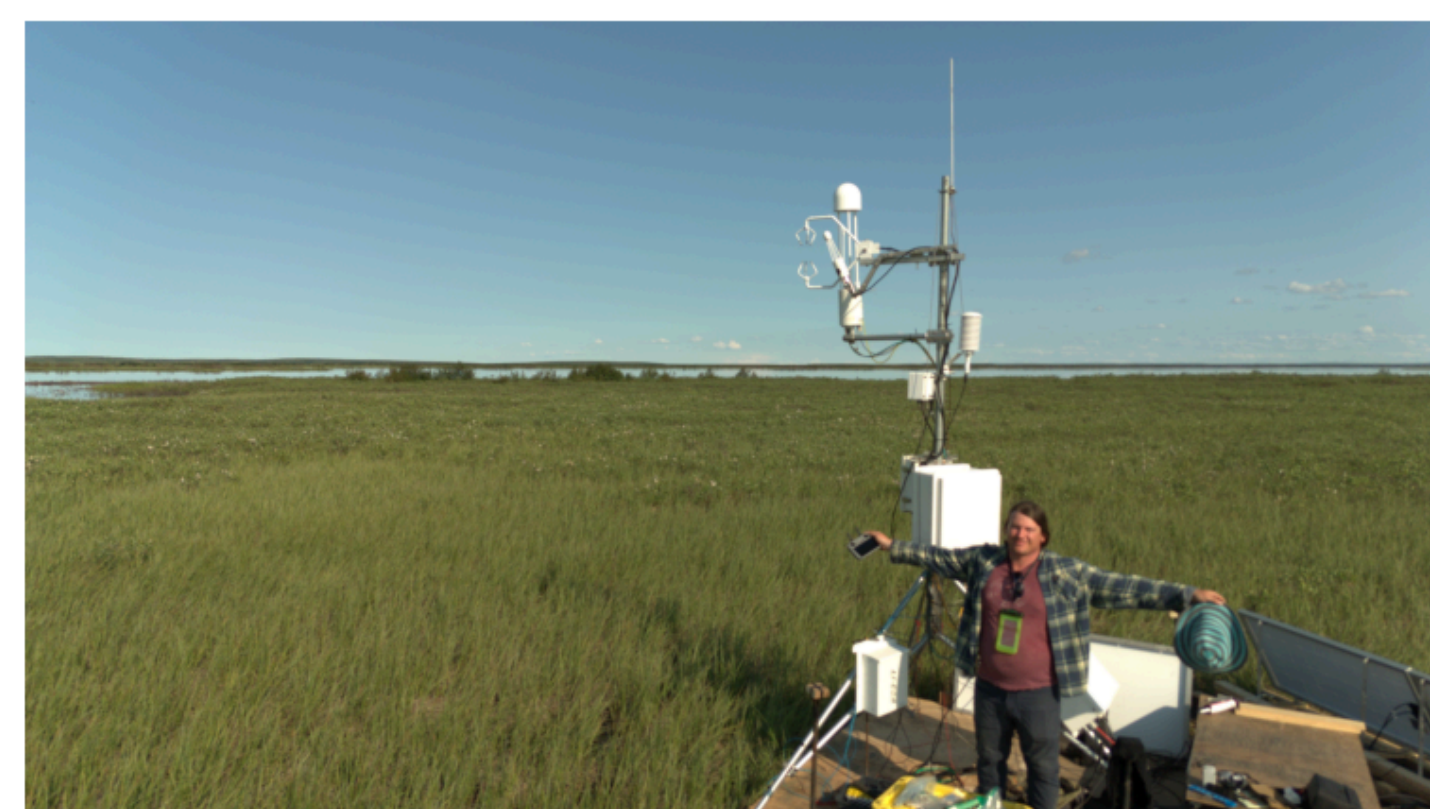
Figure 2: Eddy covariance system with open path CO 2 and CH 4 sensors.
