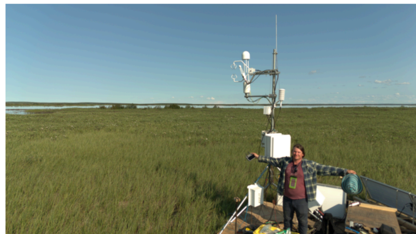
Figure 2: Eddy covariance system with open path CO 2 and CH 4 sensors.
