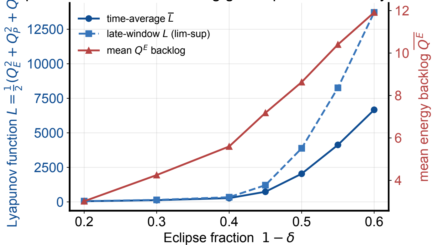
Eclipse-fraction stress: backlog grows past the stability boundary
