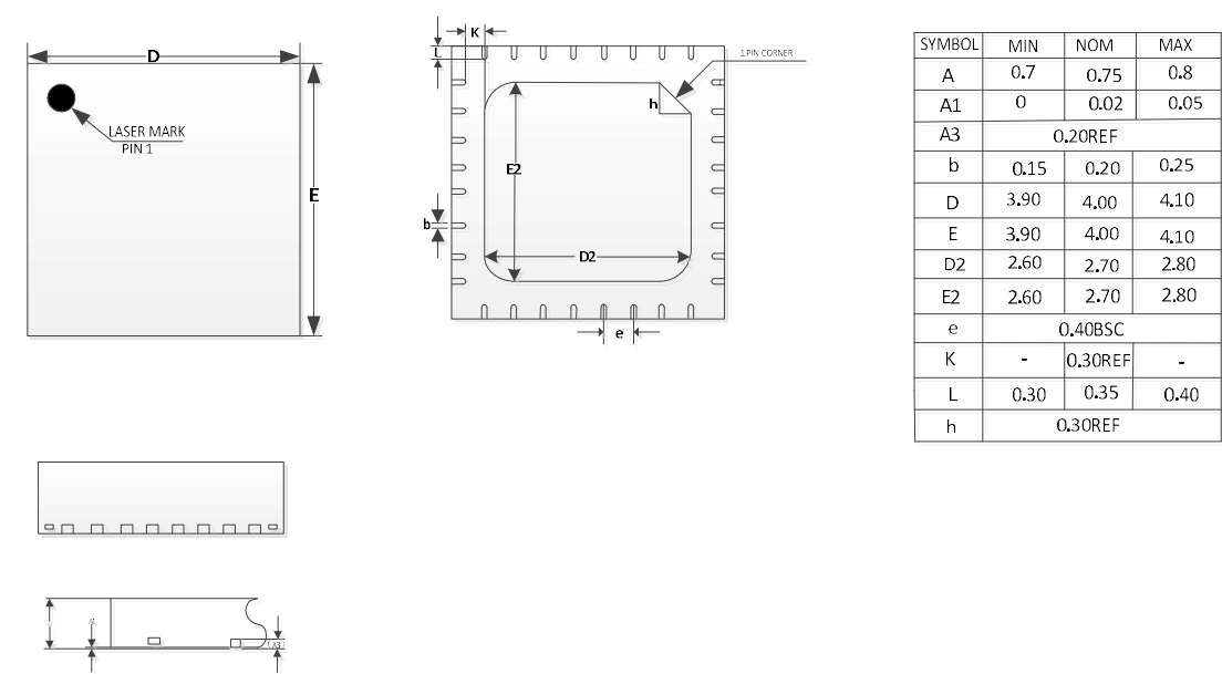
qfn32(4x4x0.75) package outline
