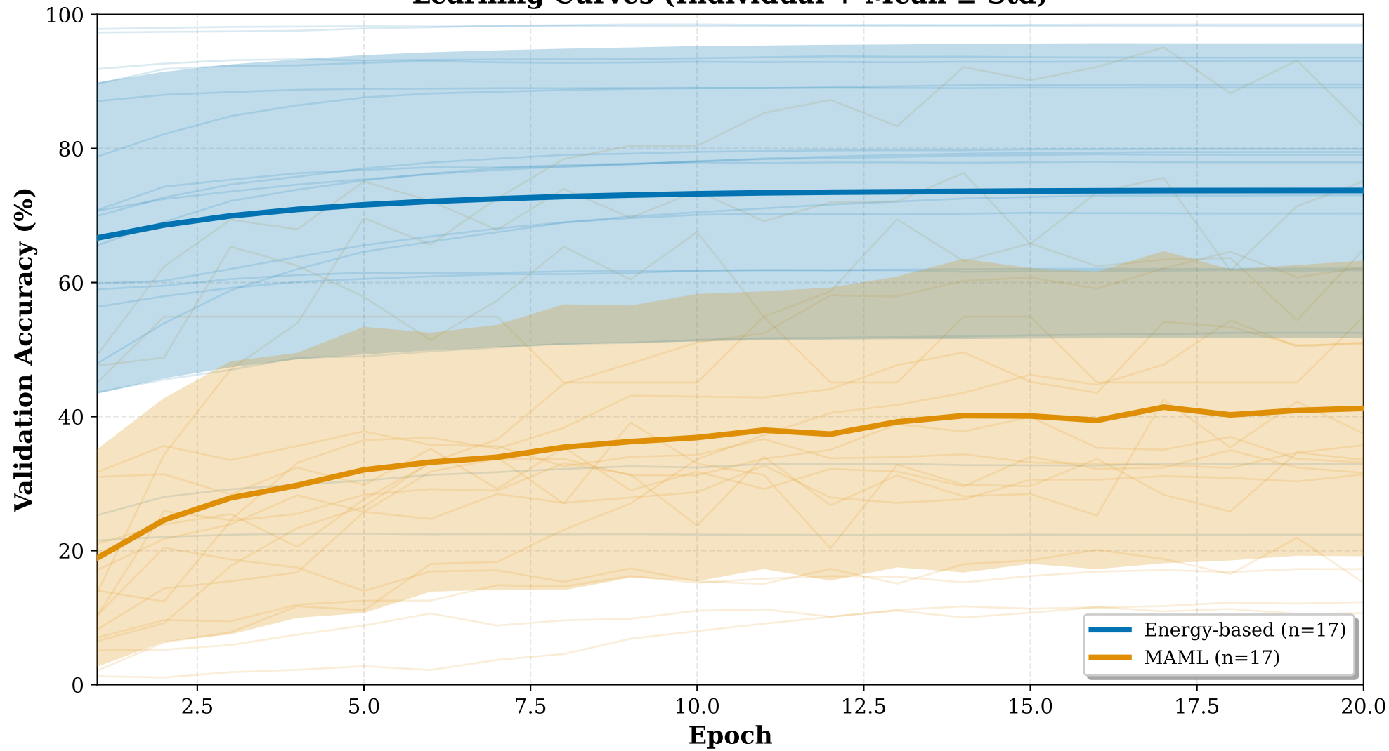
Learning Curves (Individual + Mean \pm Std)
