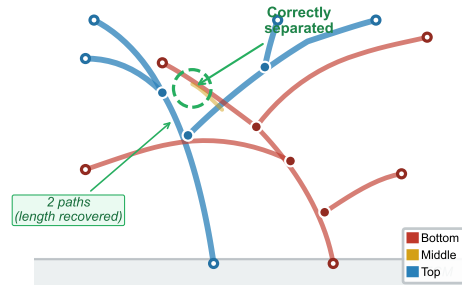
Depth-separated Skeleton
