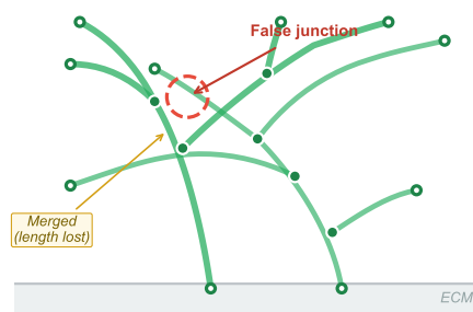
Single-color Skeleton
