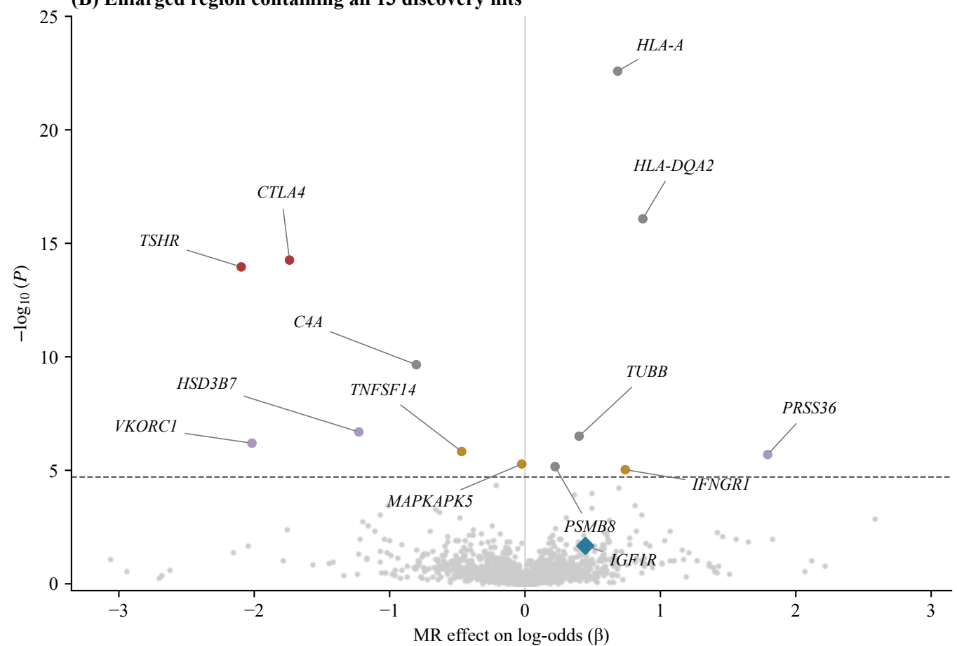
(B) Enlarged region containing all 13 discovery hits
