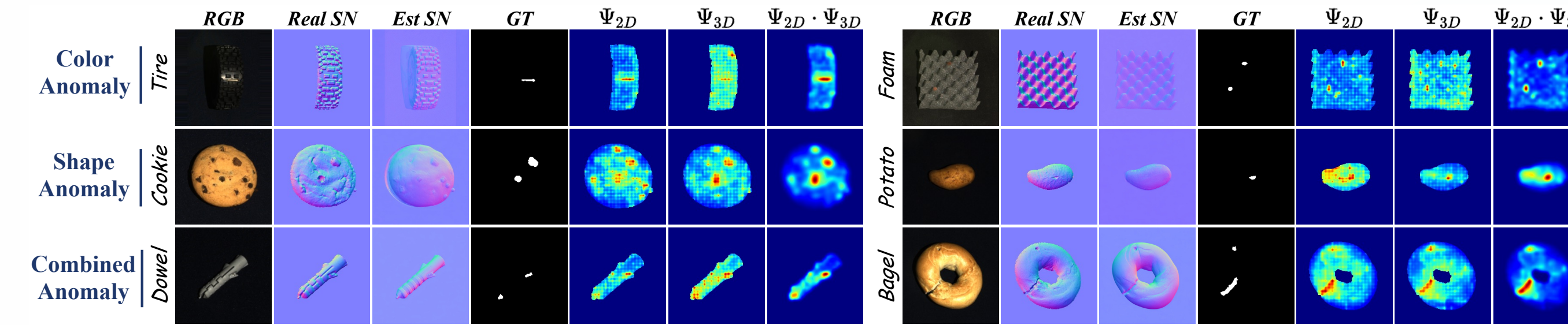
Color-only, shape-only, and combined defects are covered by complementary modality responses; the fused map suppresses unsupported background activation.
