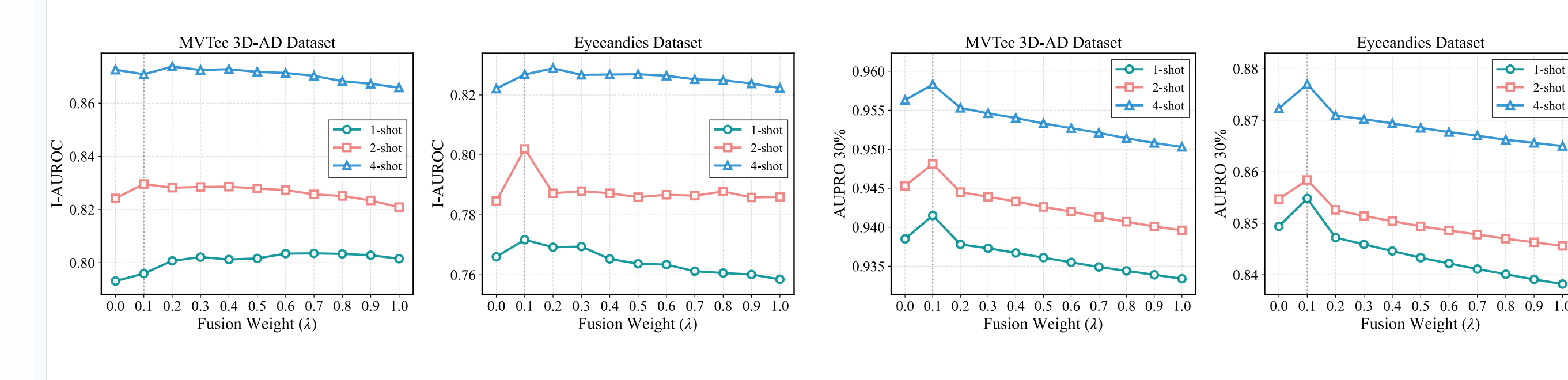
Performance remains stable around the selected balancing weights, with only small changes across the tested \lambda_1, \lambda_2 settings.
