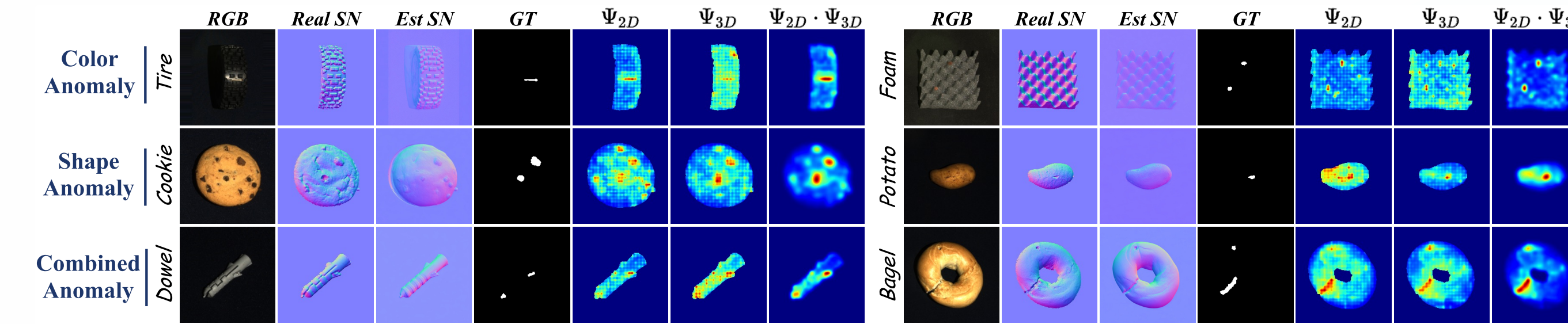
Color-only, shape-only, and combined defects are covered by complementary modality responses; the fused map suppresses unsupported background activation.
