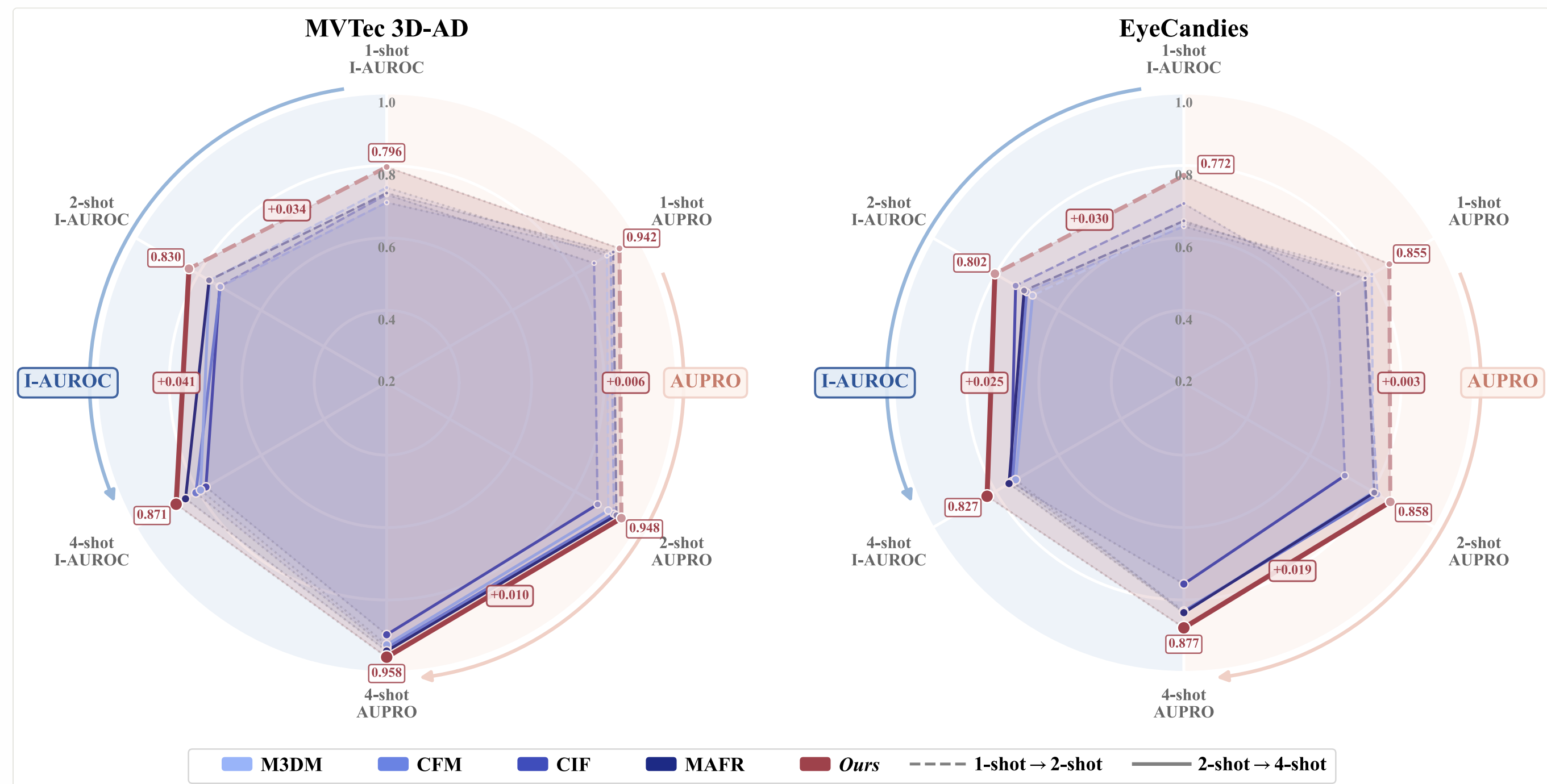
CMDs-AD (red) scales from 1 to 4 normal samples on both benchmarks.
