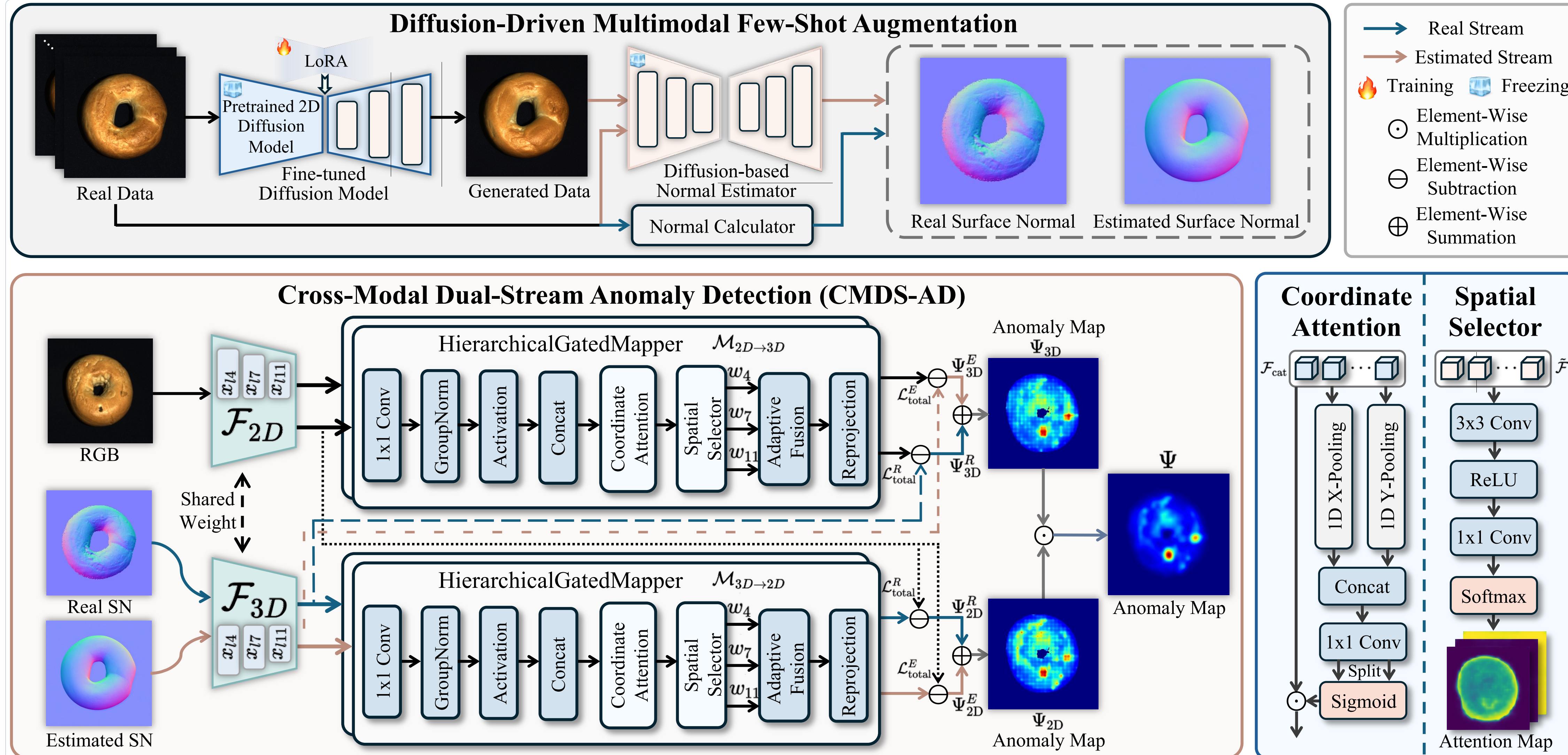
Paired diffusion augmentation creates real and estimated streams; bidirectional 2D↔3D mapping then fuses their dense anomaly evidence.
