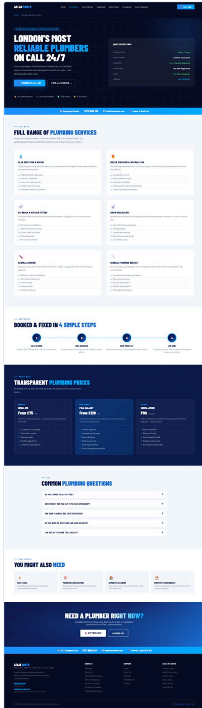
plumbing.html 1440 × 5,076px
