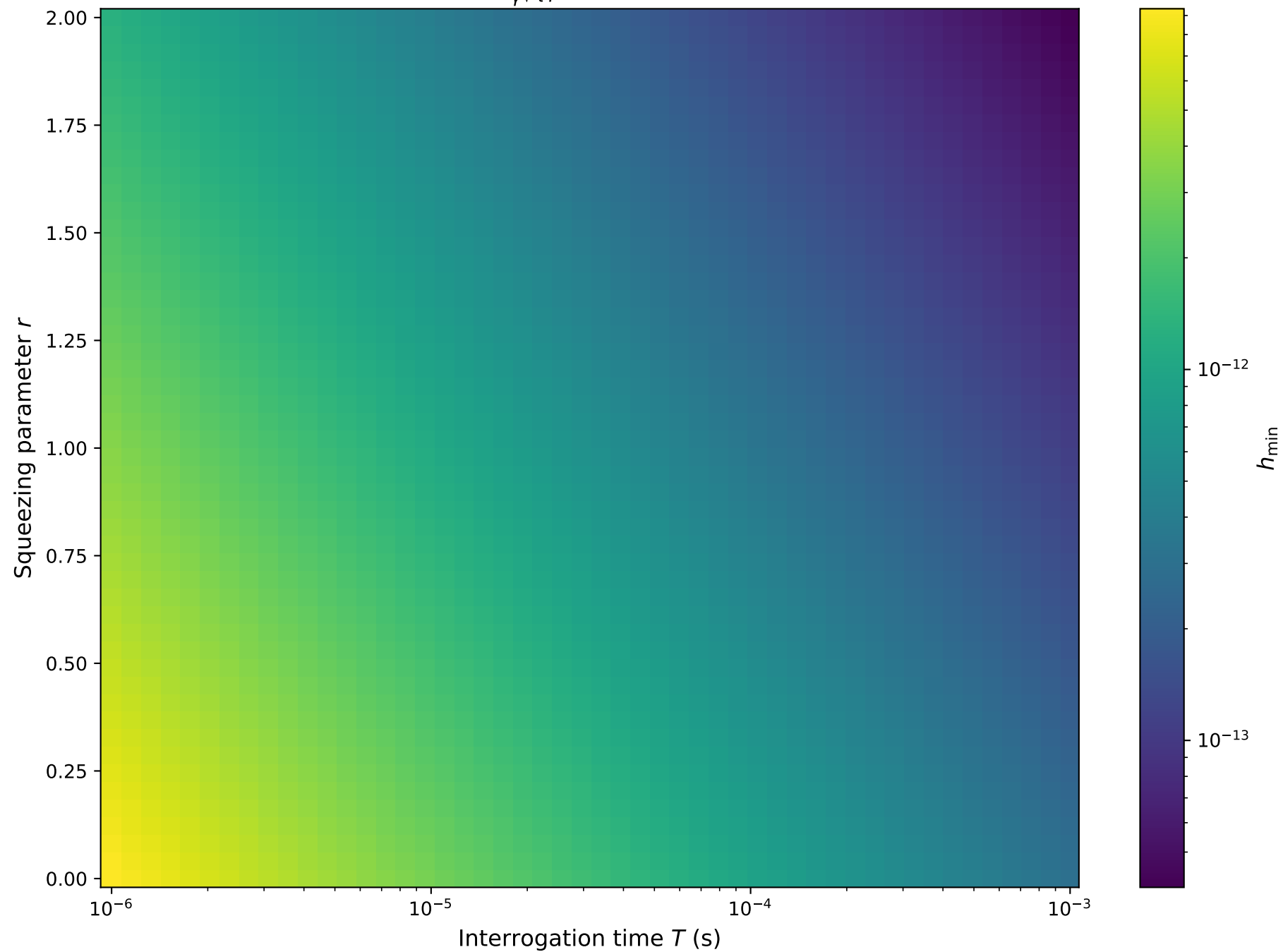
Minimum detectable strain h_{\min} as function of T and r
