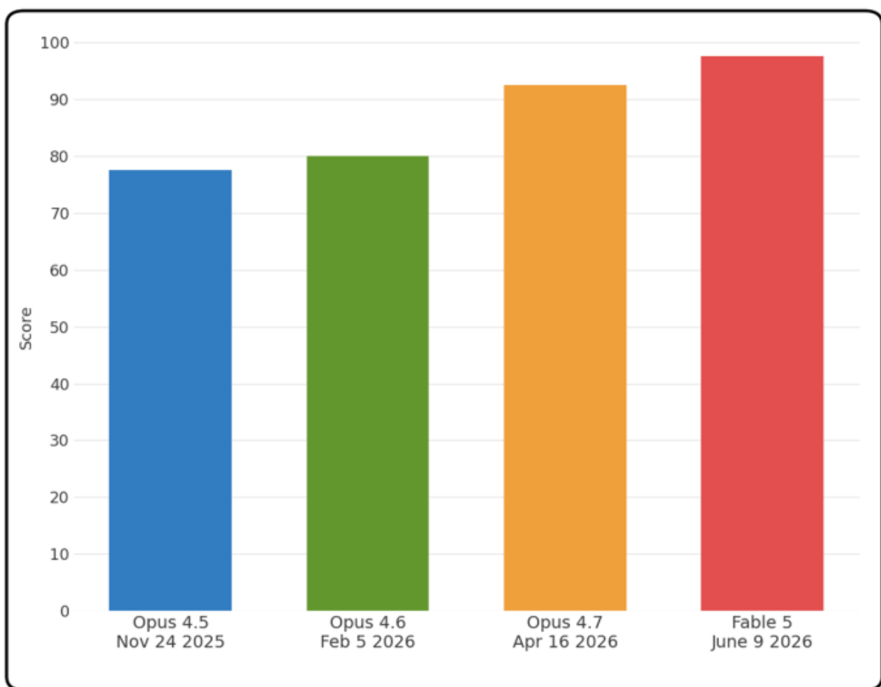
Figure 2: LLM Scores
