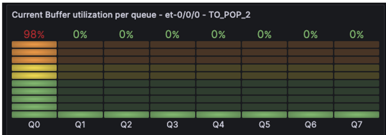
Figure 7: uRPF impact
