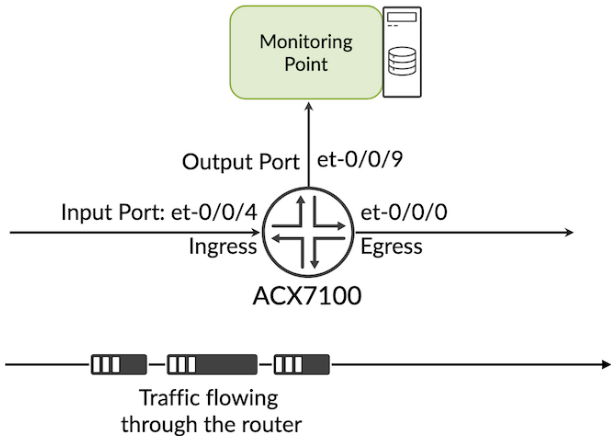
Figure 1: Topology Port Mirroring
