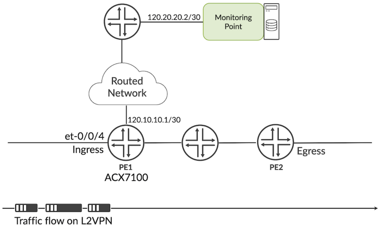
Figure 3: Topology ERSPAN
