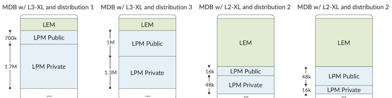
Figure 6: Examples of lpm-distribution
