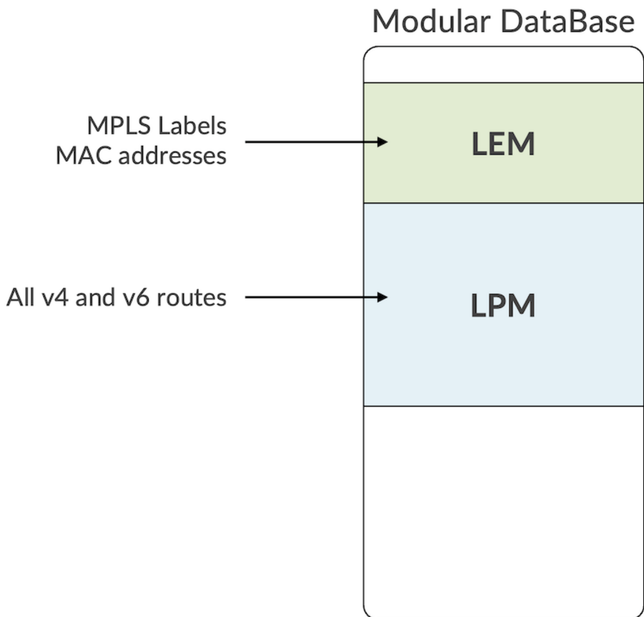
Figure 5: LEM and LPM roles starting from Junos 23.2R1
