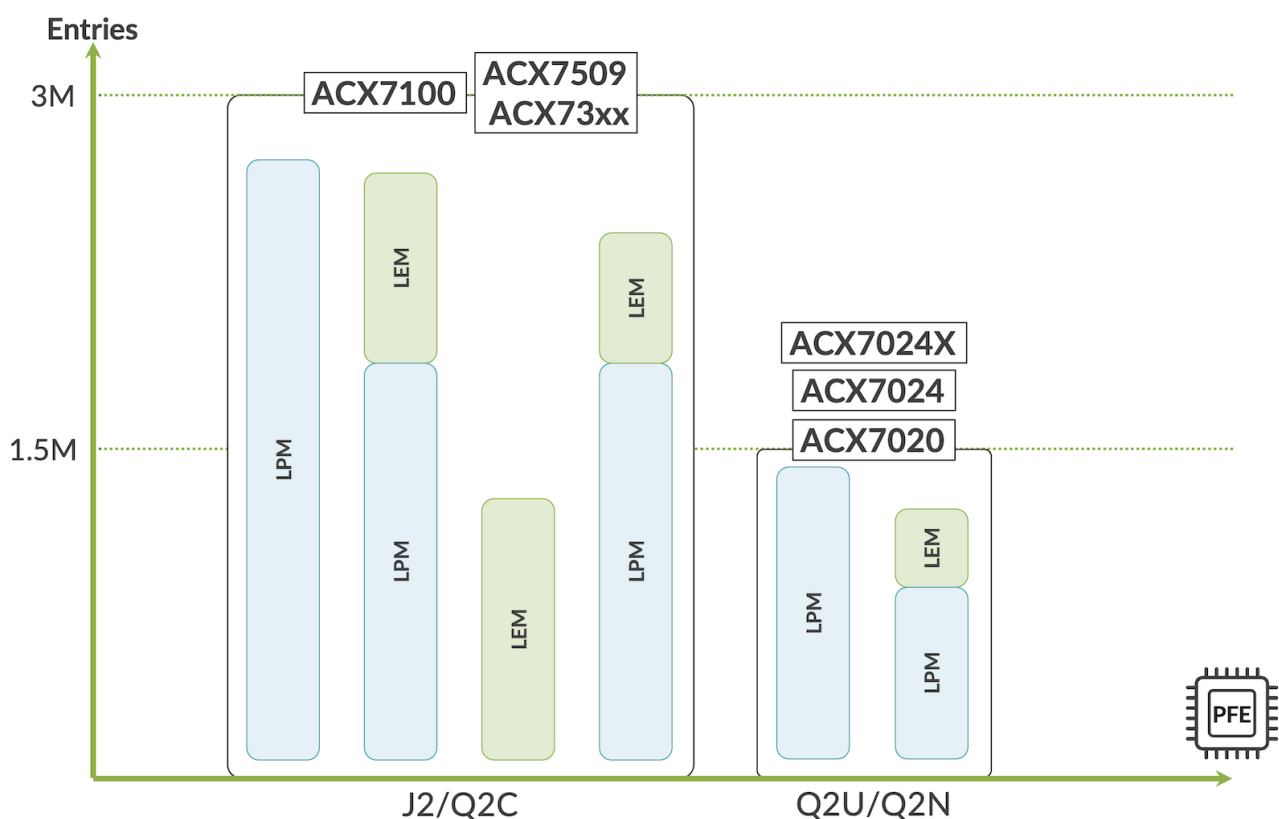
Figure 2: DNX Jericho2 PFE and Associated MDB Sizes
