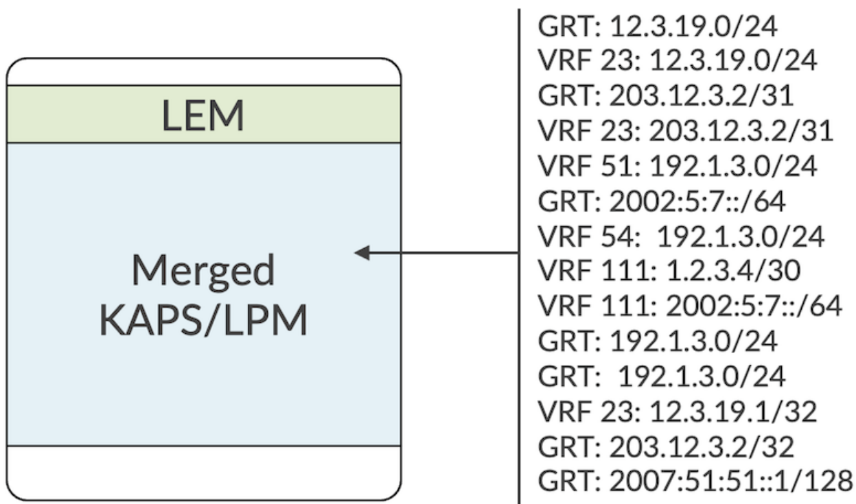
Figure 10: Simplification of the route-storing logic
