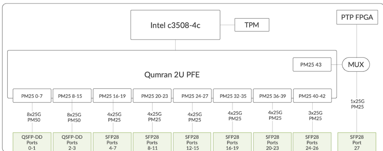
Figure 2: ACX7024 Block Diagram
