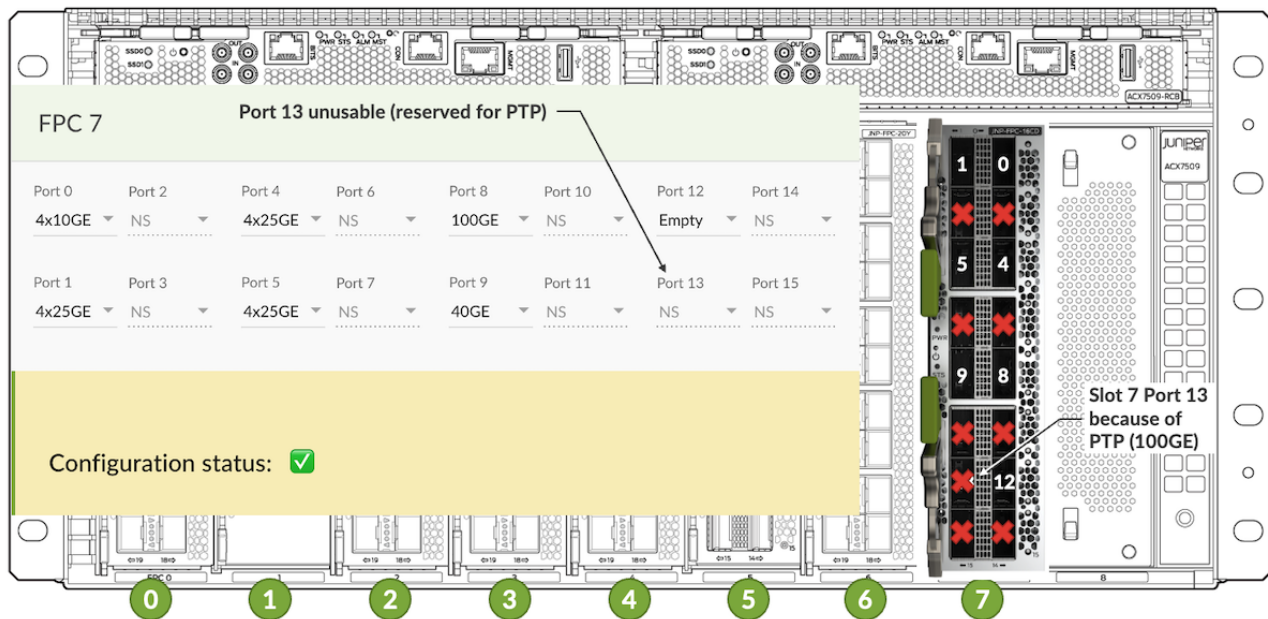
Figure 27: Port 13 disabled in slot 7 for PTP
