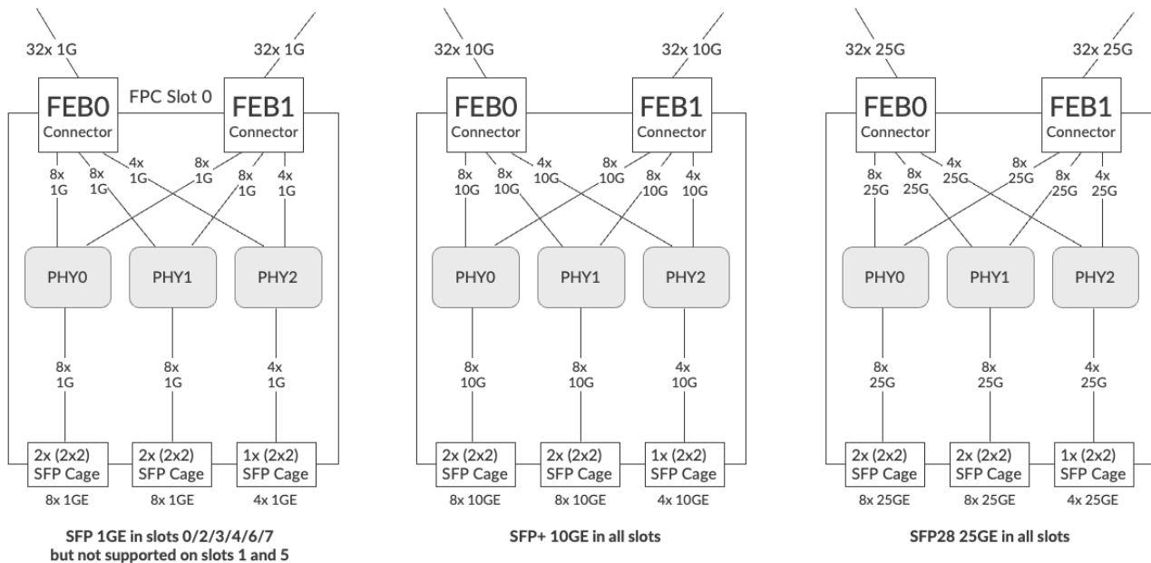
Figure 18: ACX7509-FPC-20Y capability in different chassis slots
