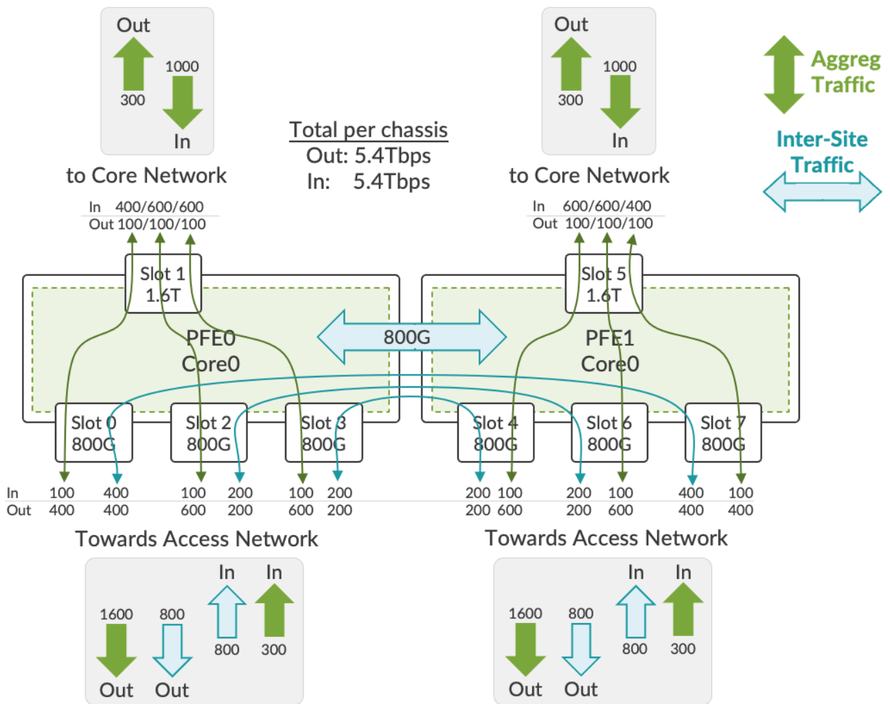
Figure 33: Example of optimization in Aggregation use-case
