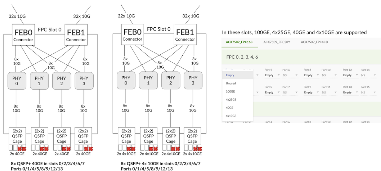
Figure 25: ACX7509-FPC-16C and 40GE/4x10GE in PM25 slots
