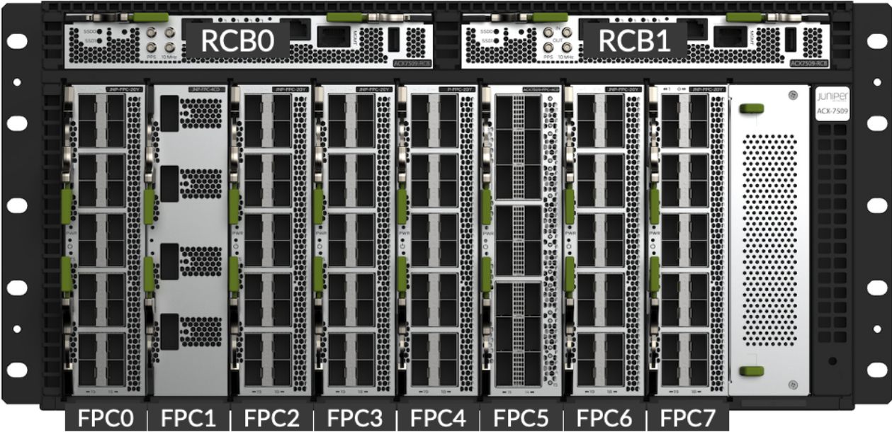
Figure 15: ACX7509 FPC slots numbering
