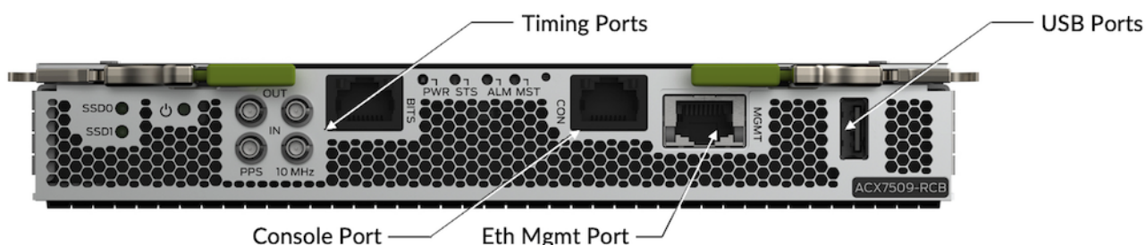
Figure 11: ACX7509 Routing and Control Board
