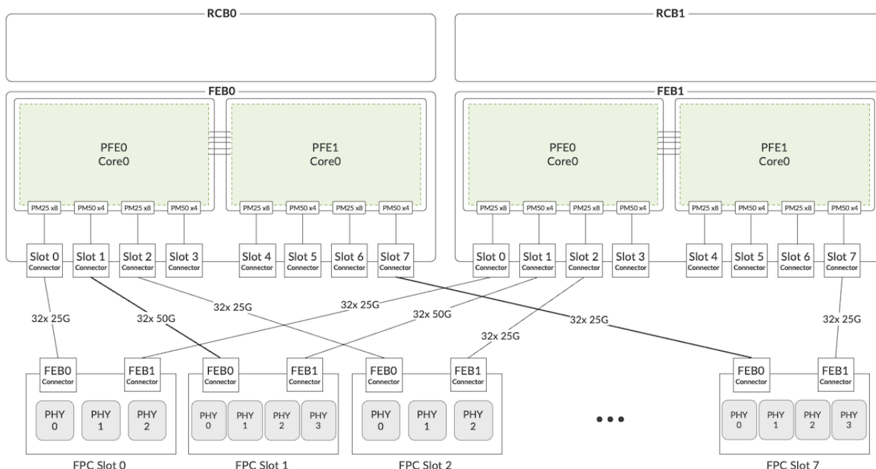
Figure 30: ACX7509 High Level block diagram
