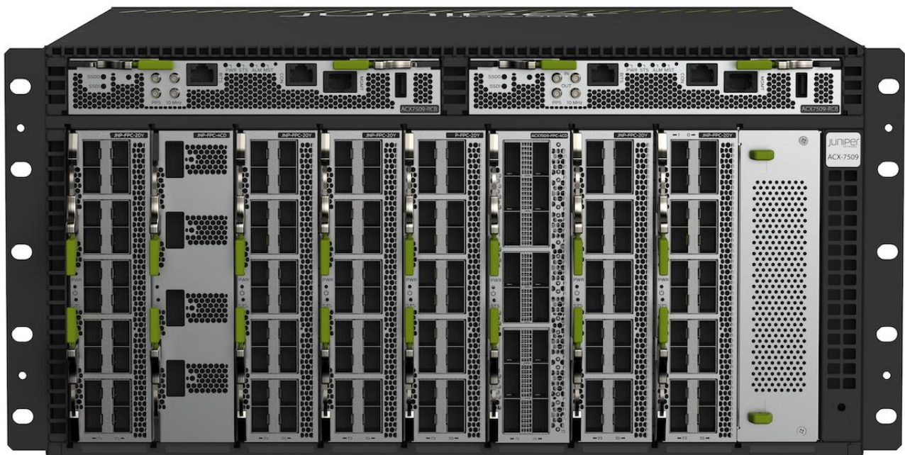
Figure 1: Front view of the ACX7509
