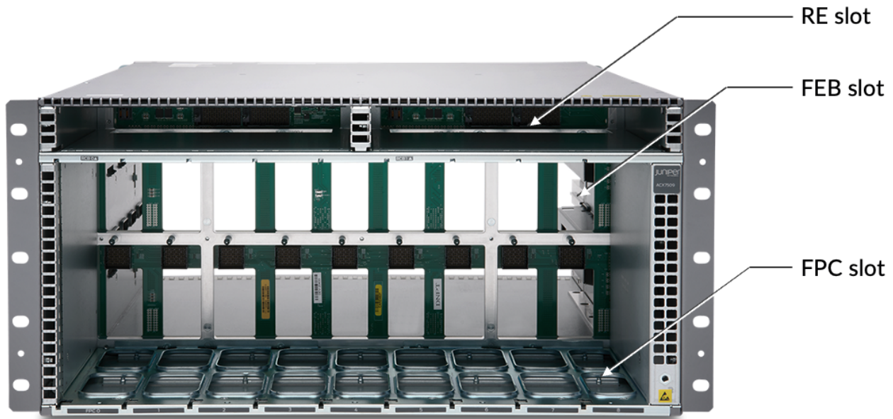
Figure 5: Front view of an empty ACX7509 chassis
