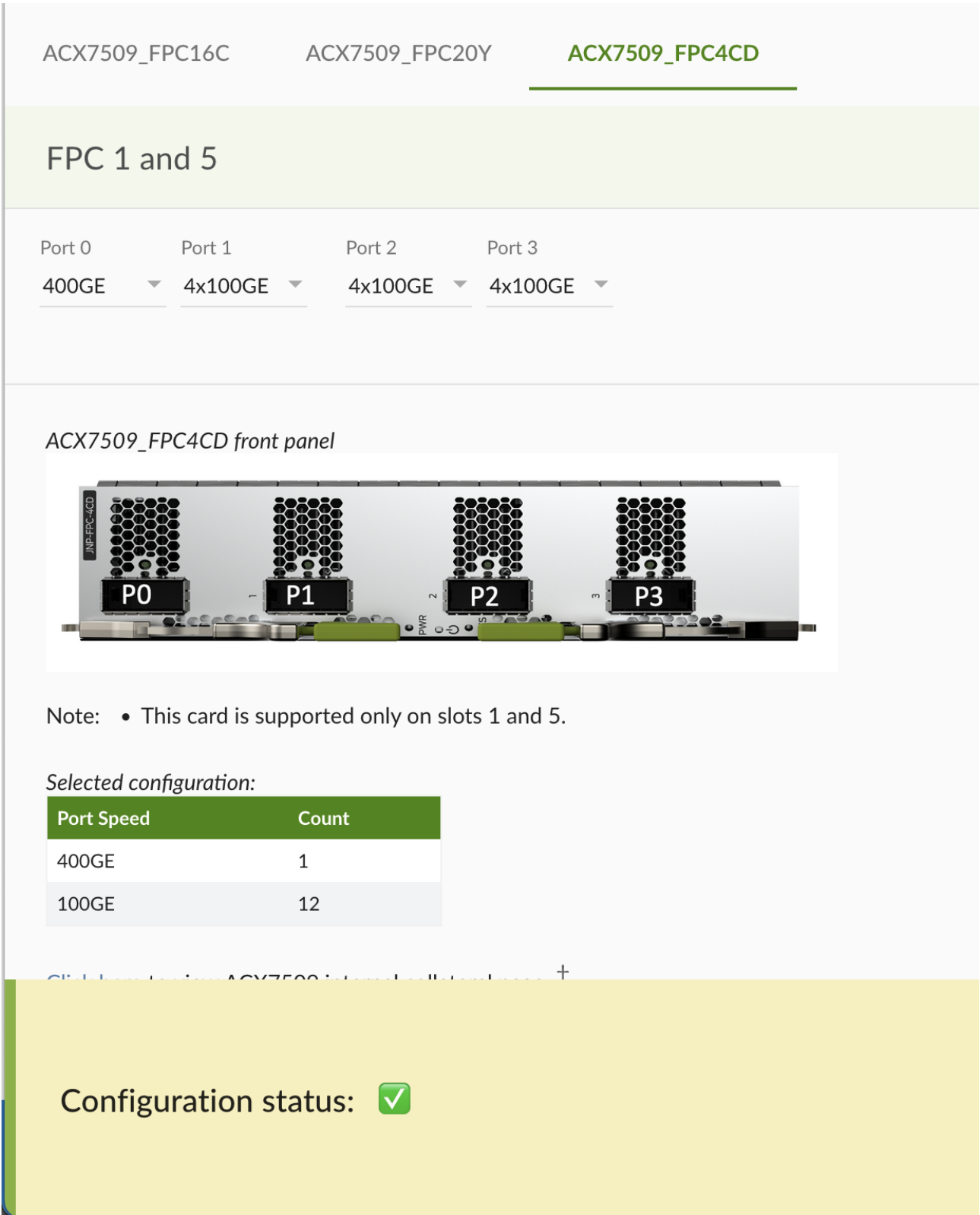
Figure 29: ACX7509-FPC-4CD Different options in the port checker
