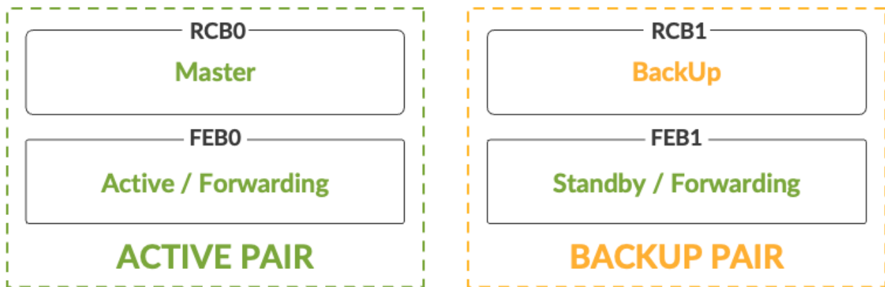
Figure 35: Nominal redundant state
