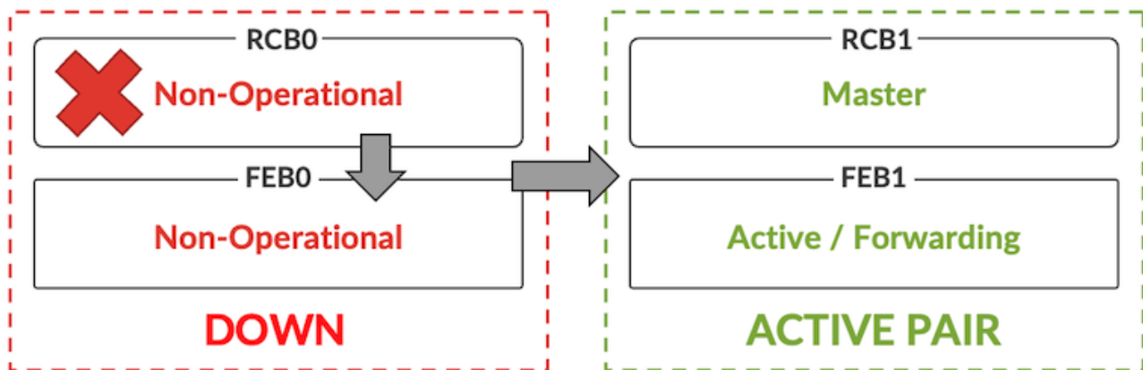
Figure 36: RCB0 failure scenario
