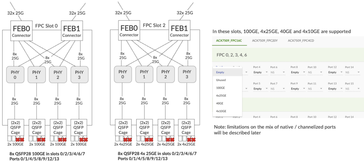
Figure 24: ACX7509-FPC-16C and 100GE/4x25GE in PM25 slots
