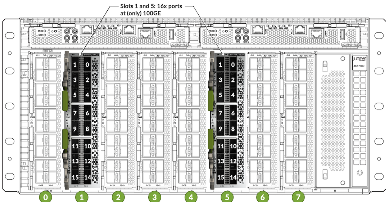
Figure 22: ACX7509-FPC-16C and Port Checker options in PM50 slots (1 and 5)
