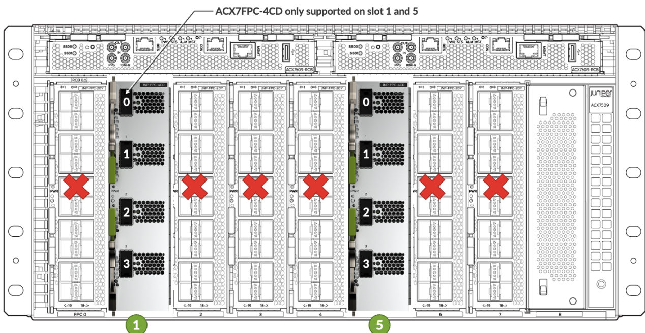
Figure 28: ACX7509-FPC-4CD in Slots 1 and 5
