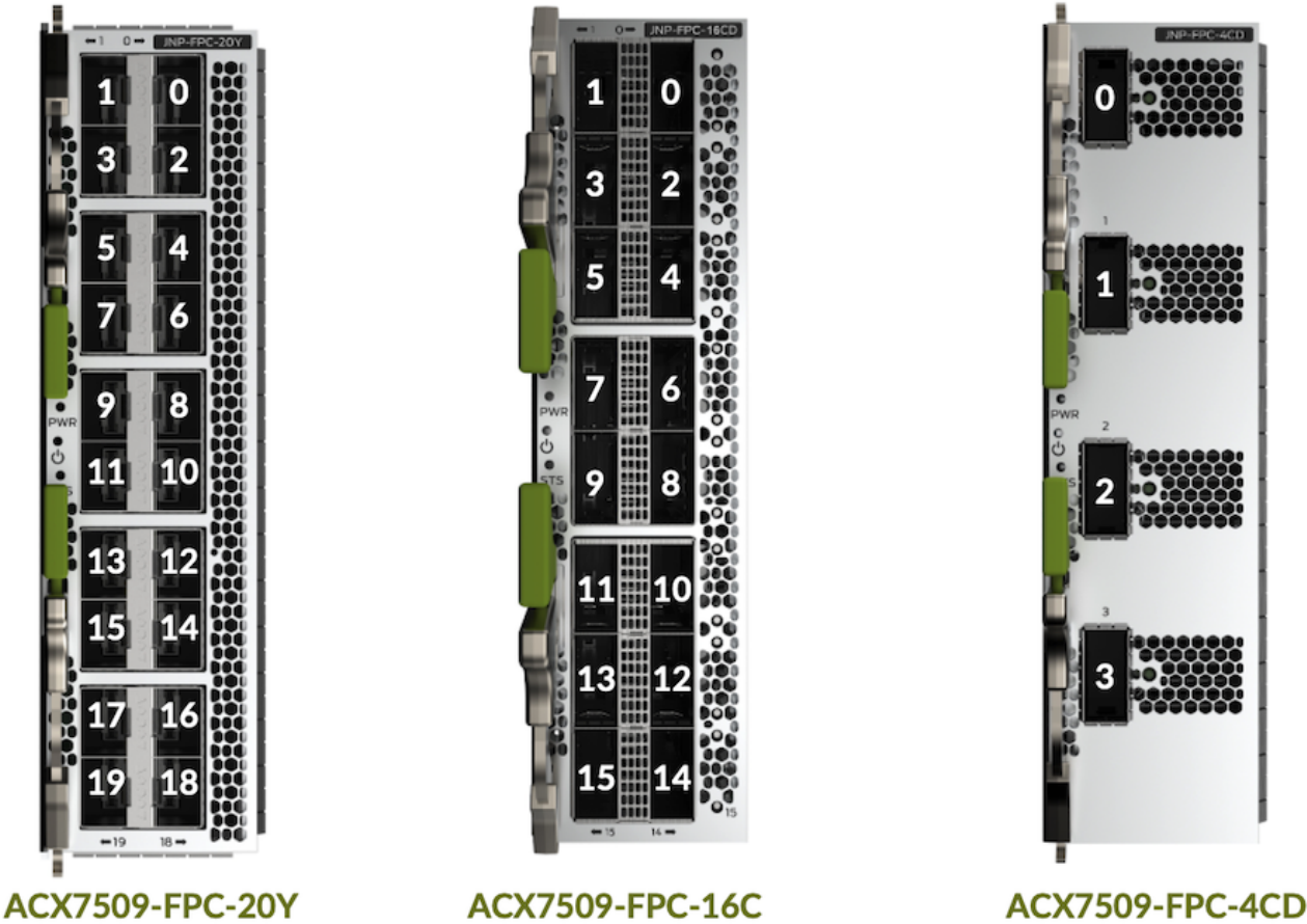
Figure 16: FPC ports numbering
