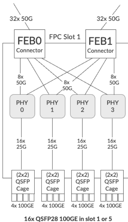
Figure 21: ACX7509-FPC-16C in slots 1 and 5
