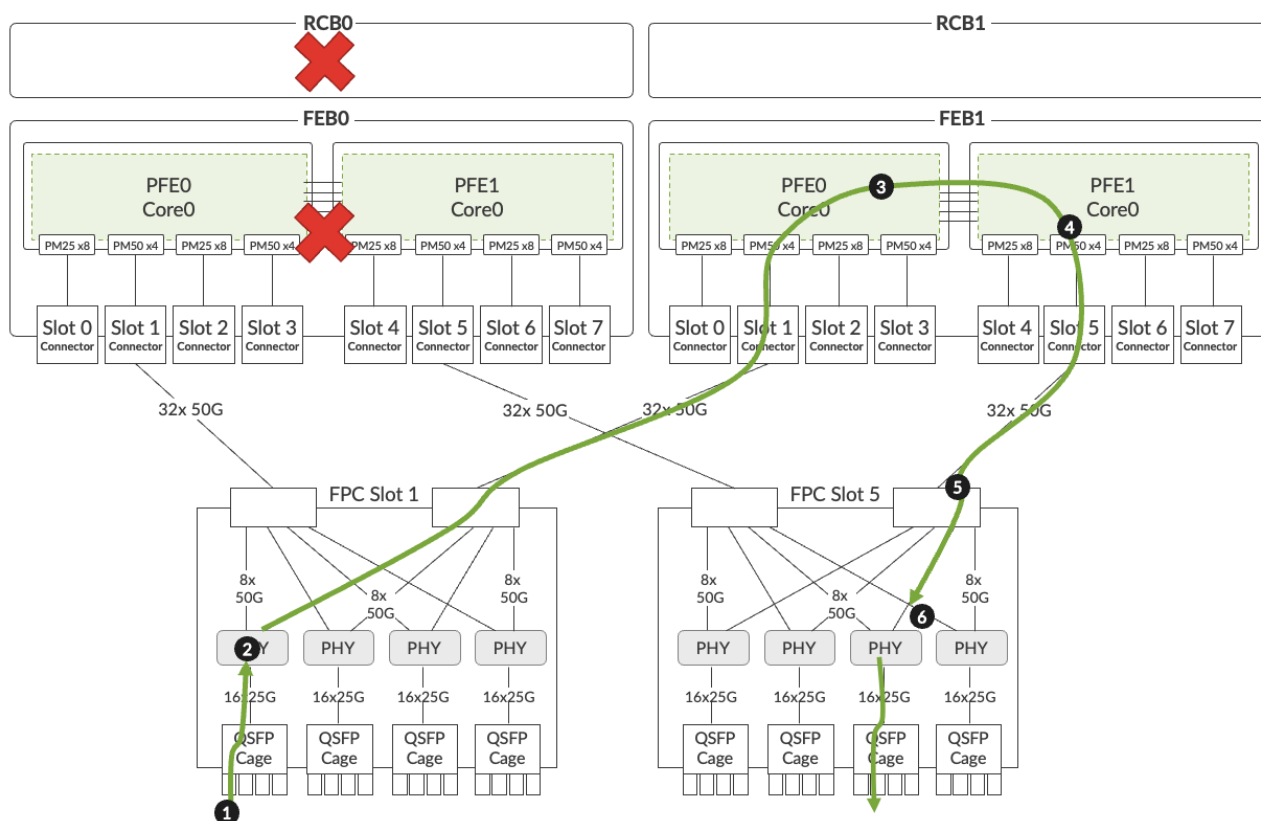
Figure 39: FEB0 failure scenario
