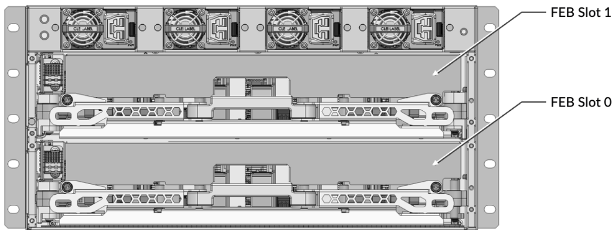
Figure 13: Position of the FEBs in the back of the ACX7509 chassis
