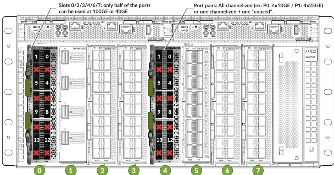
Figure 23: ACX7509-FPC-16C examples in PM25 slots
