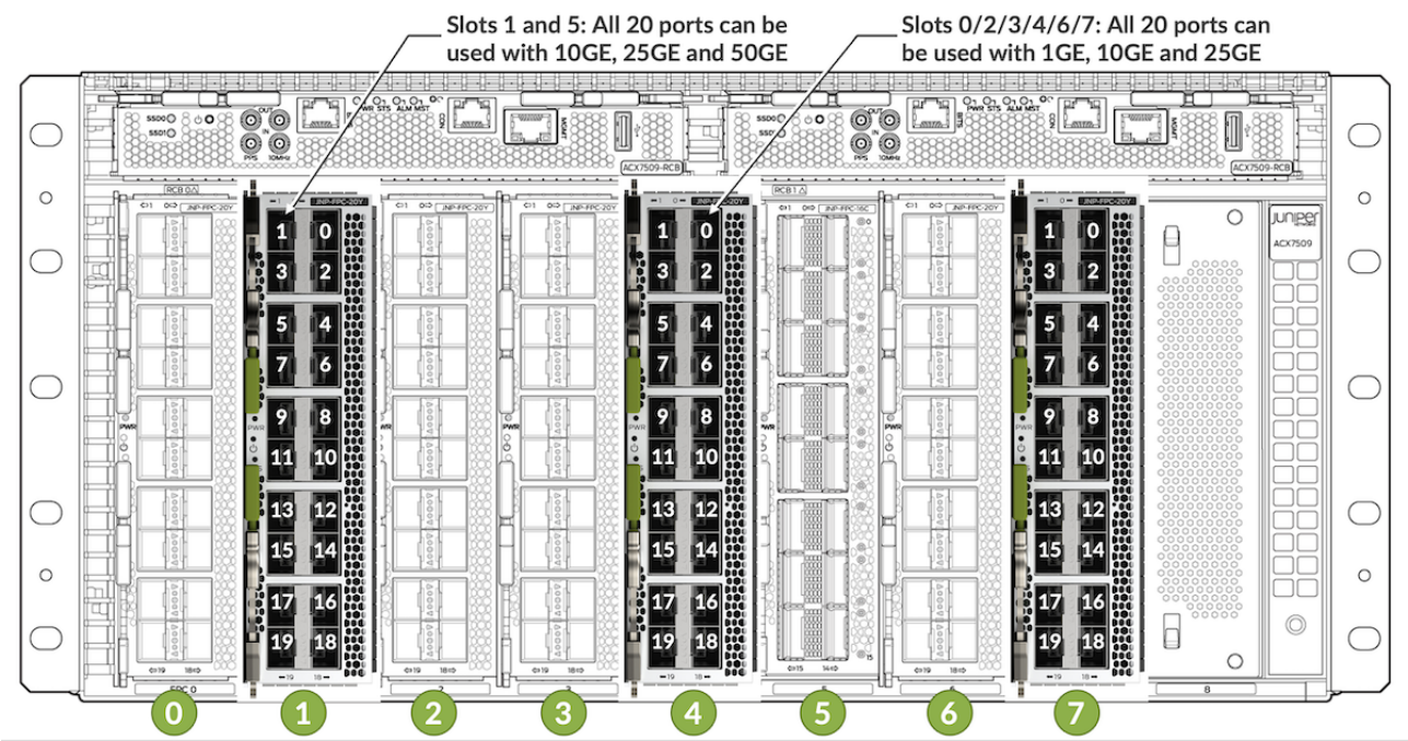
Figure 19: Using ACX7509-FPC-20Y for 1GE, 10GE and 25GE
