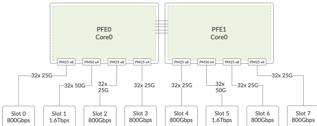
Figure 17: FPC slots connections to the PFEs of a FEB
