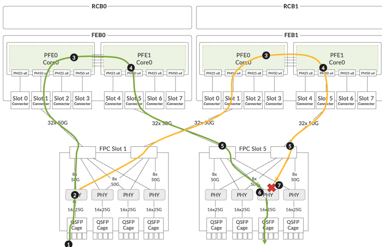
Figure 38: Redundant mode data path
