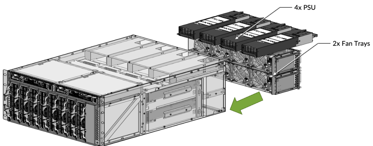
Figure 14: PSU and Fan Trays inserted in the rear side of a ACX7509 chassis
