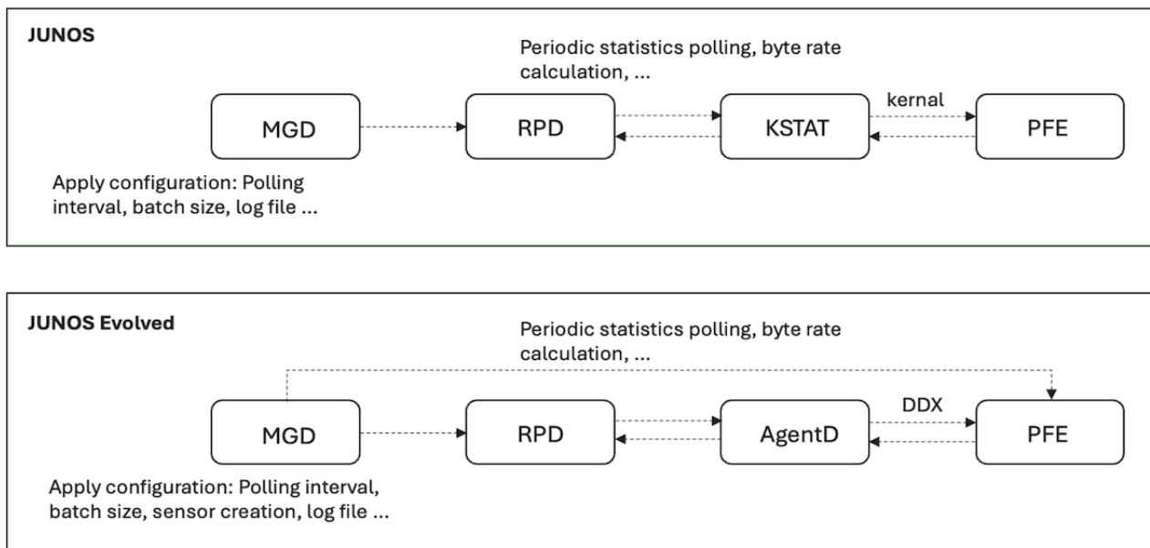
Figure 1: Statistics Collection in Junos OS and Junos OS Evolved
