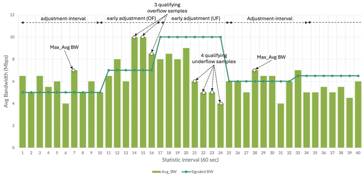
Figure 3: Overflow/underflow illustration
