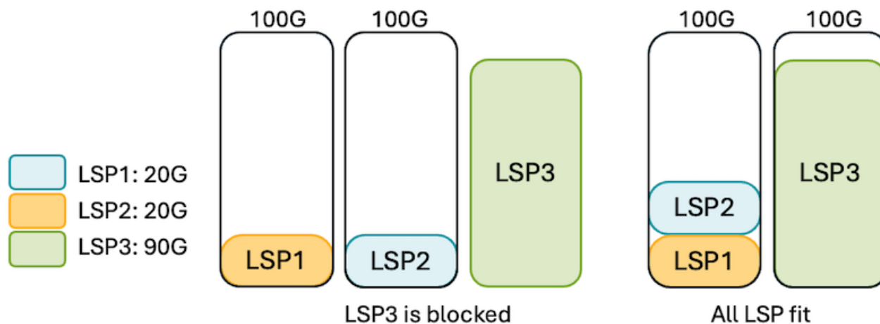
Figure 2: LSP blocking
