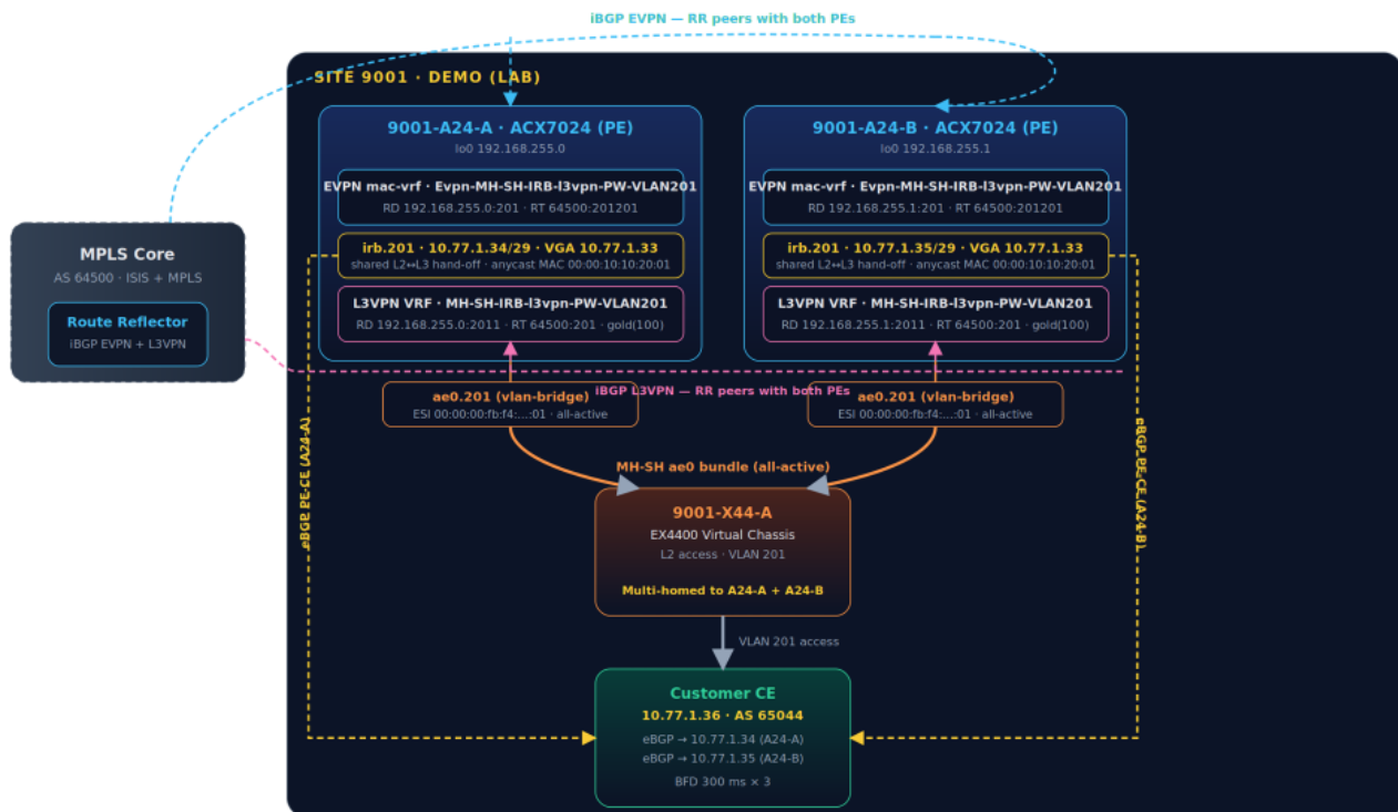
Figure 2: Paired L3VPN/EVPN over VLAN201 Topology
