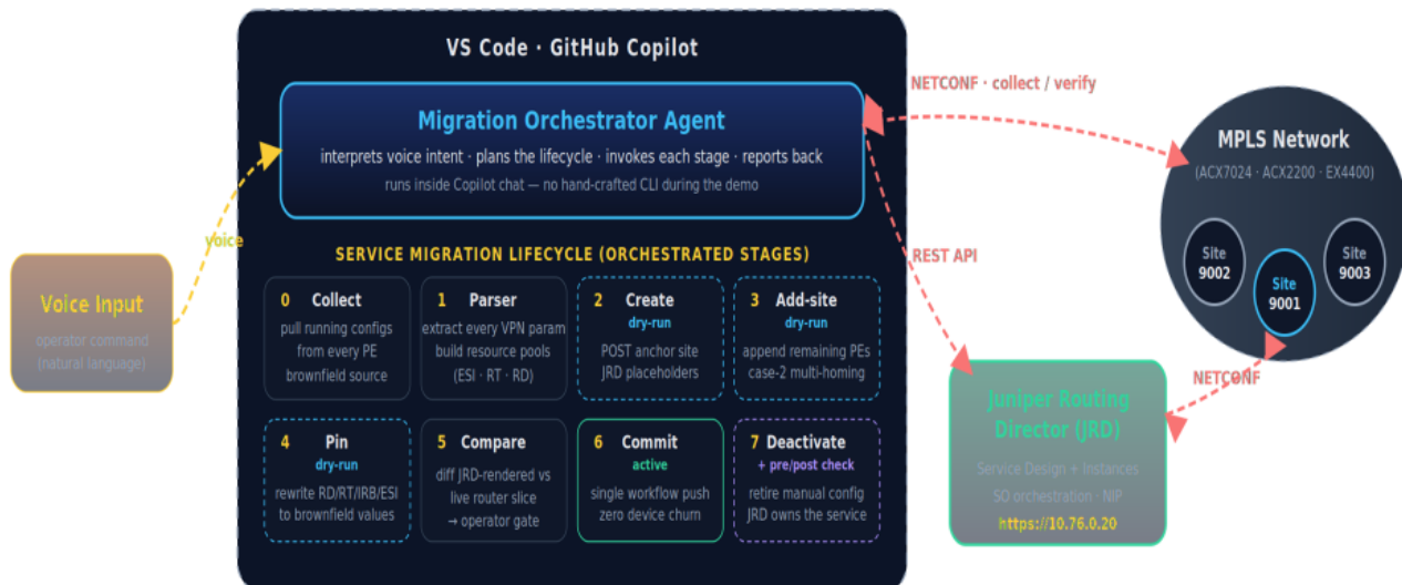
Figure 1: Brownfield Migration Pipeline Framework
