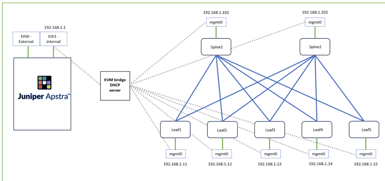
Figure 3: Juniper Apstra to virtual fabric integration
