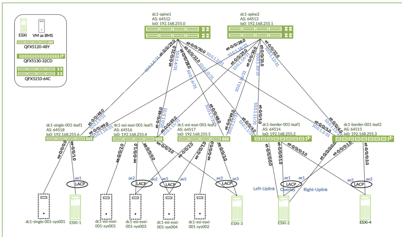
Figure 2: 3 Stage (ERB) Datacenter Topology
