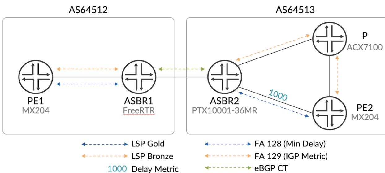
Figure 1: BGP CT Test topology
