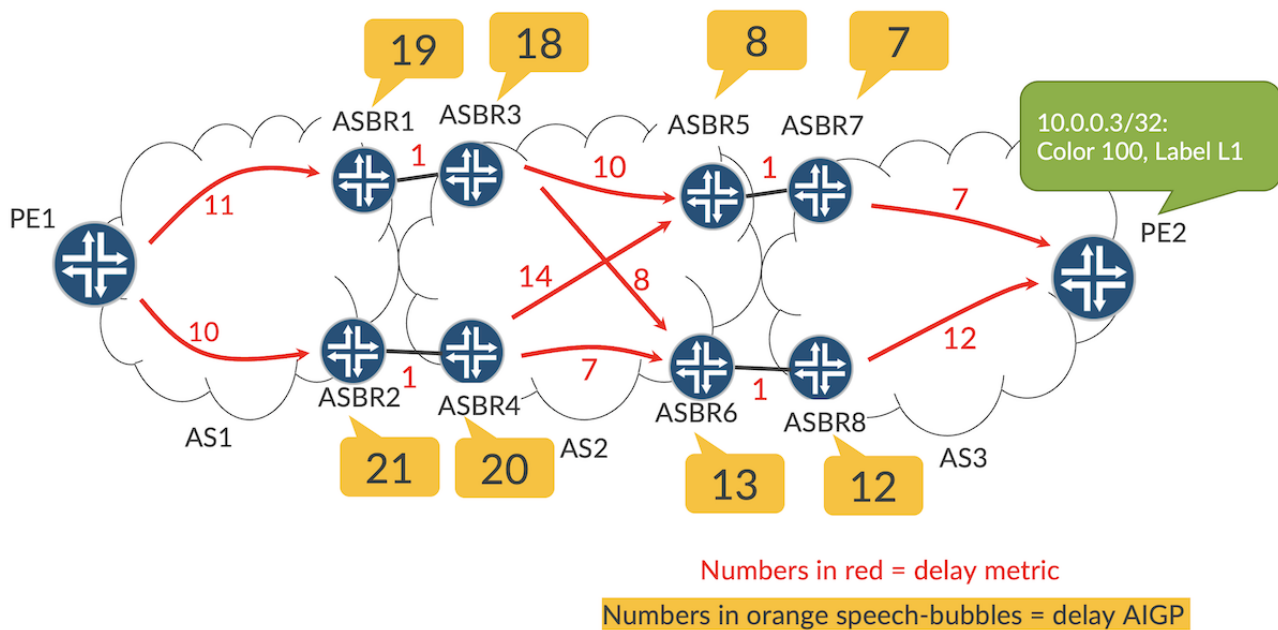
Figure 6: using Generalized AIGP with BGP-CT to achieve optimum end-to-end path
