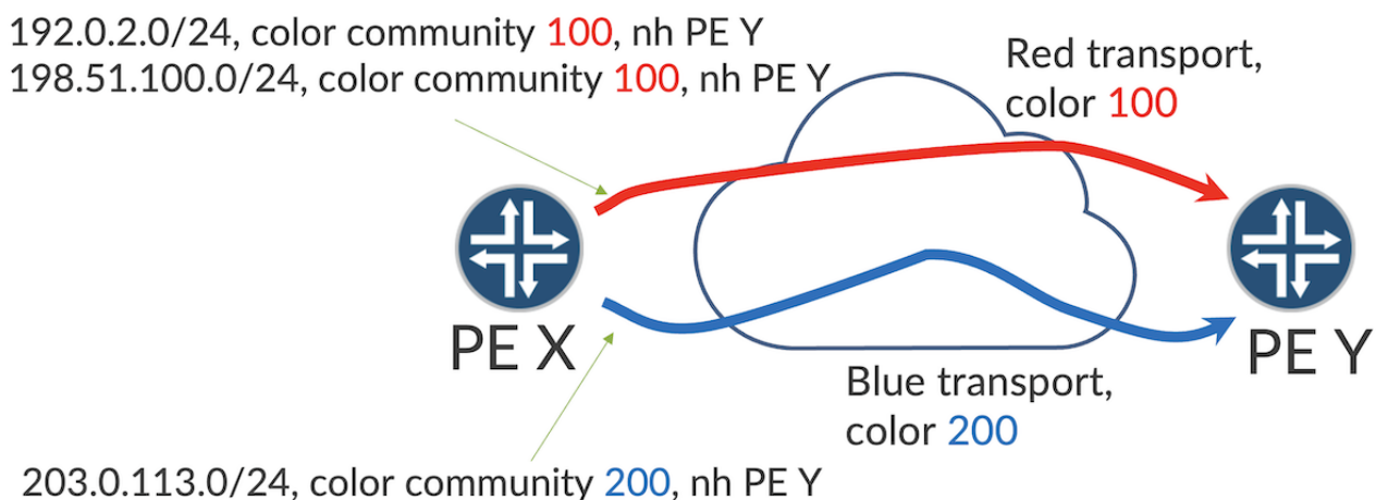
Figure 1: Color-based transport within a single AS
