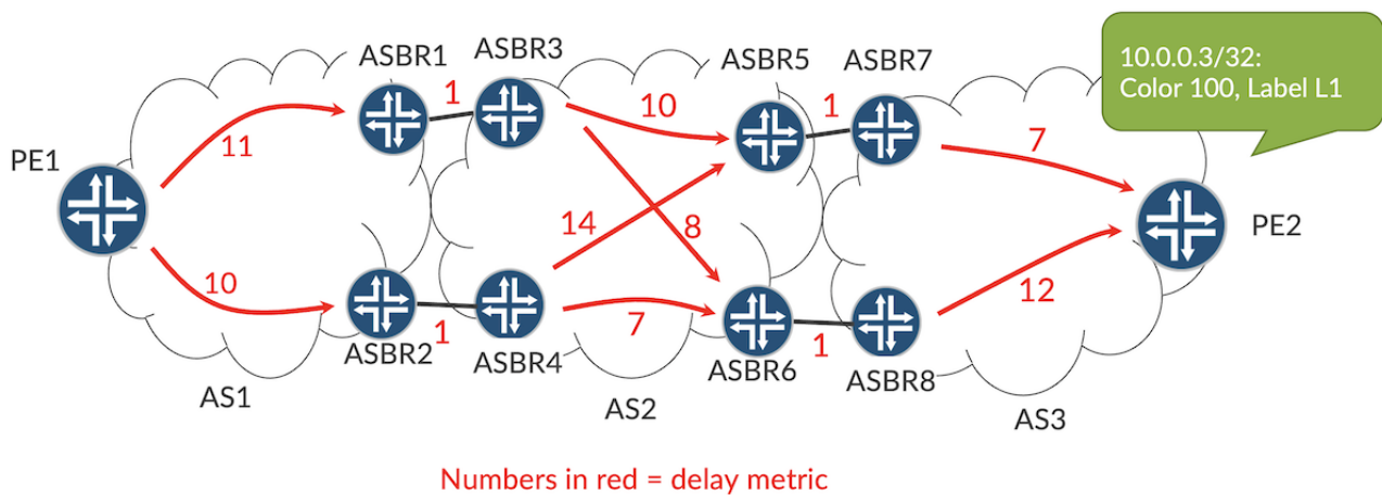
Figure 5: Delay metrics in a multi-AS scenario
