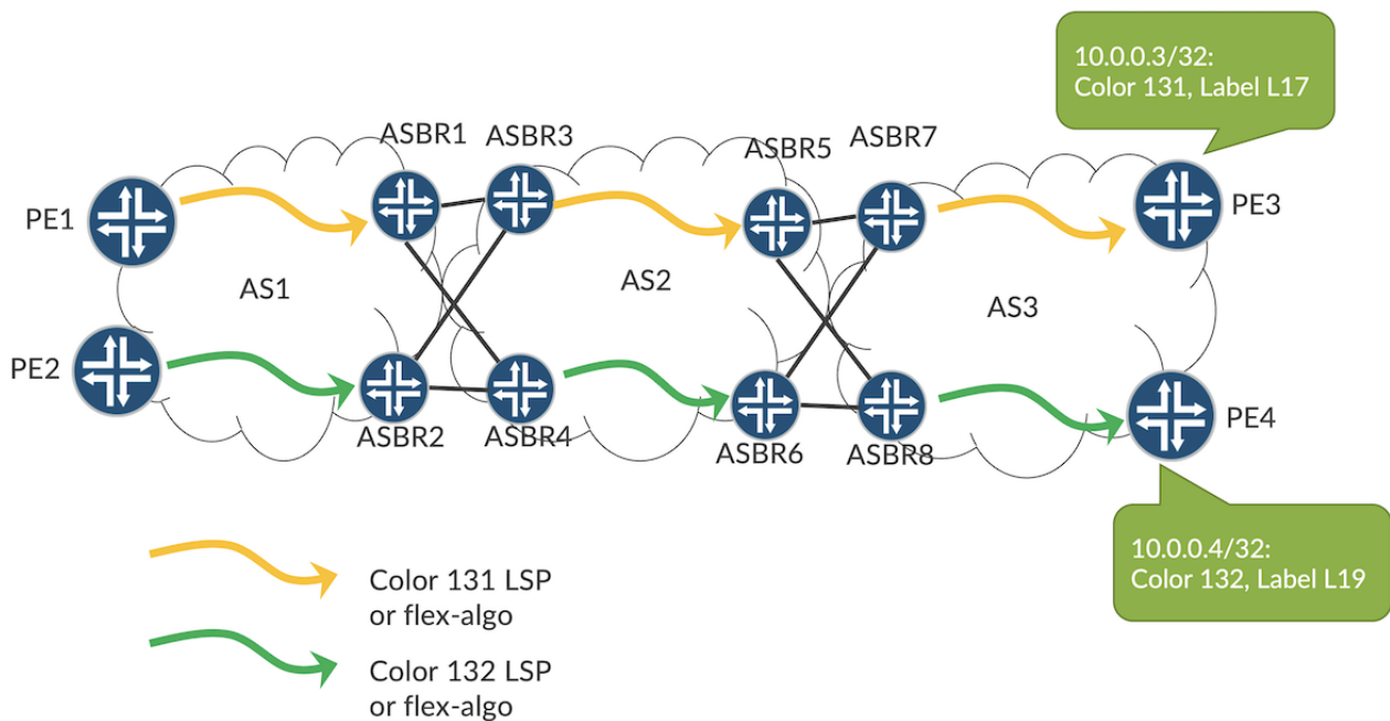
Figure 3: Path diversity across multiple ASes with BGP-CT
