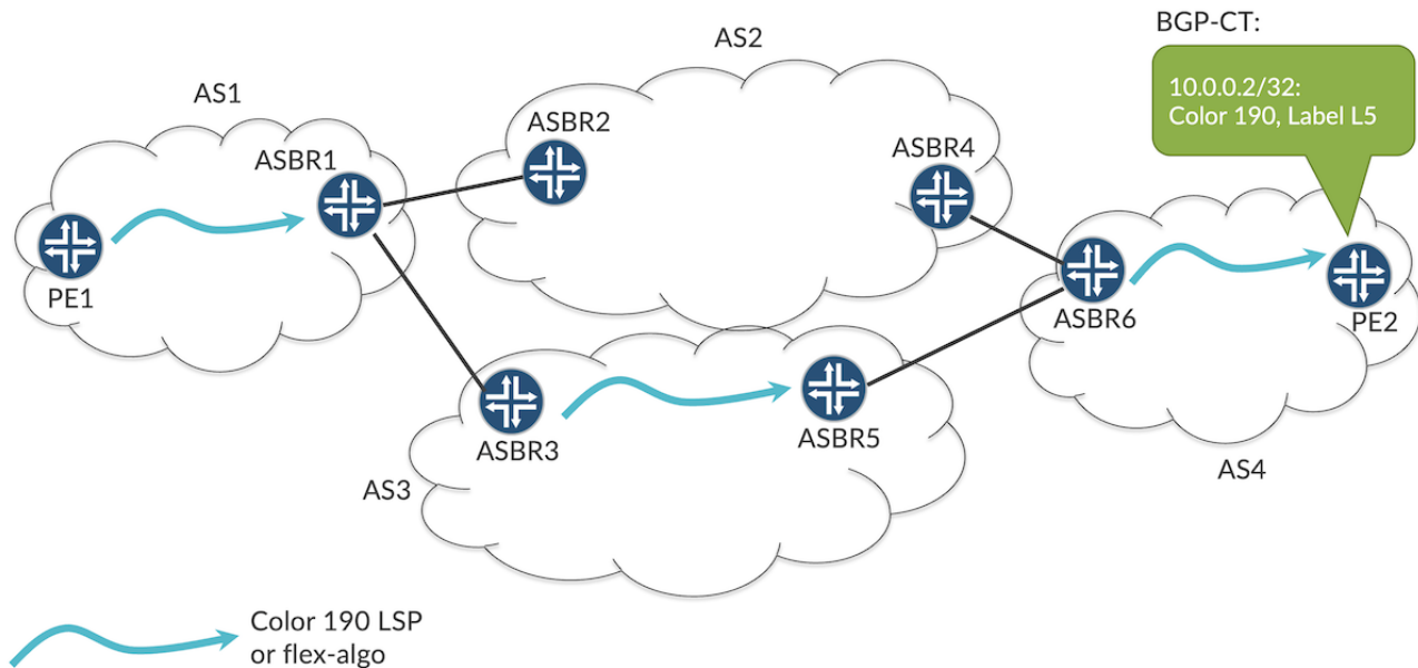
Figure 4: Geo-routing with BGP-CT
