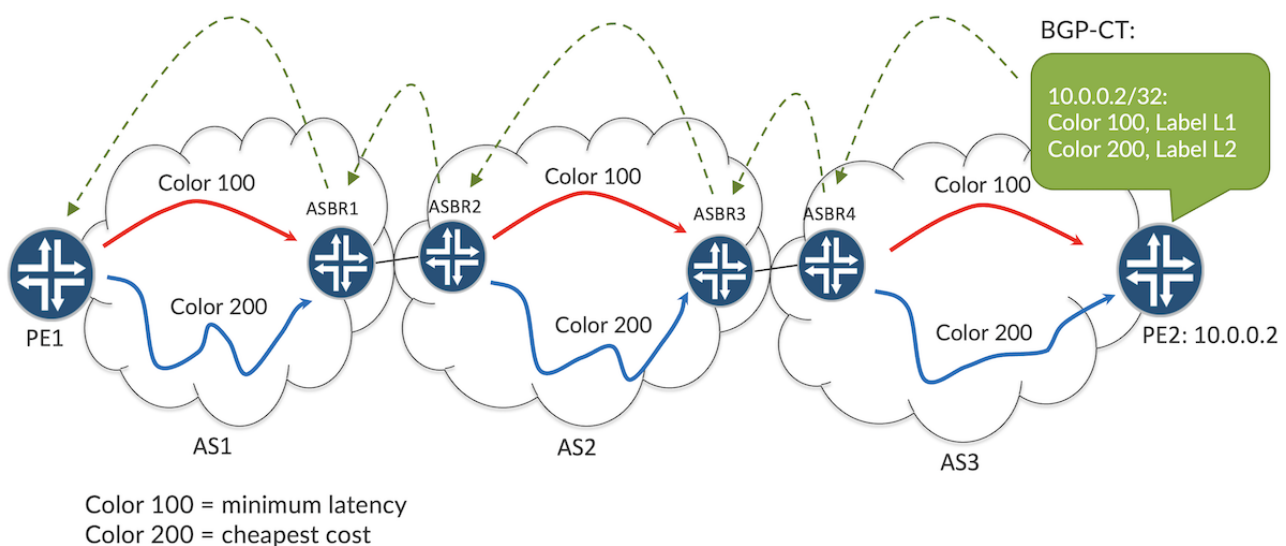
Figure 2: Extending color-based transport across multiple ASes with BGP-CT
