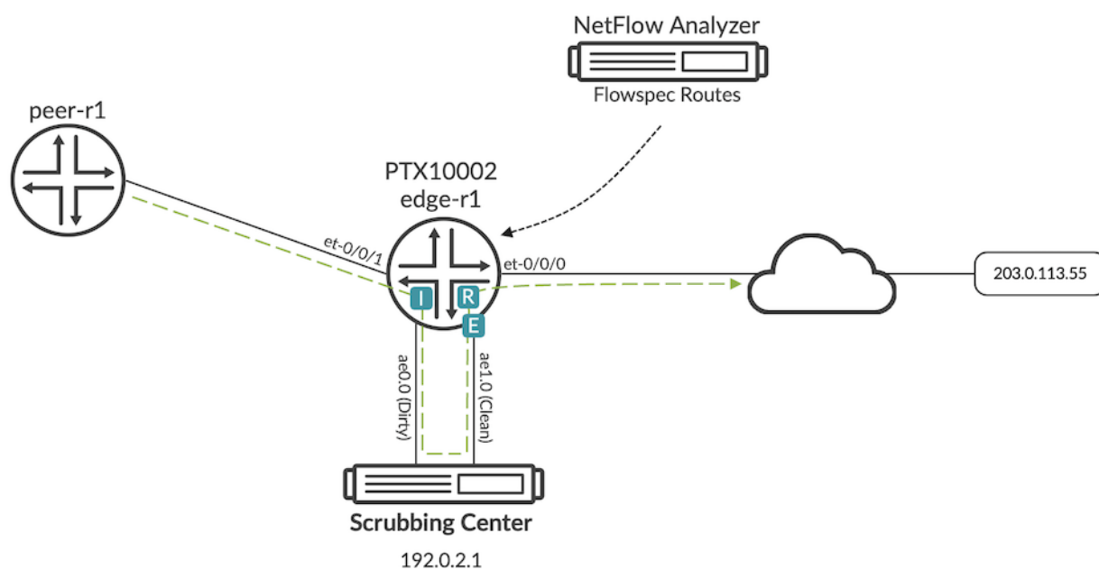
Figure 2: BGP FlowSpec Loop Free Traffic (Explicit Interface Filters)
