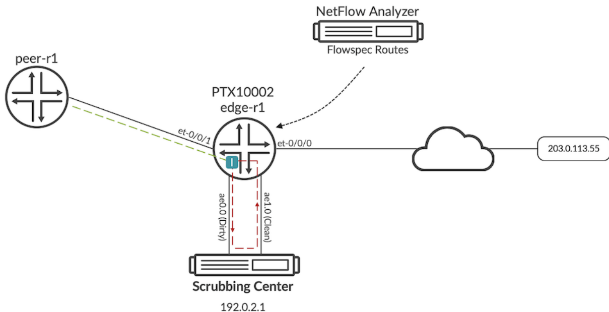
Figure 1: BGP FlowSpec Looped Traffic (Implicit Forwarding-Table Filter)
