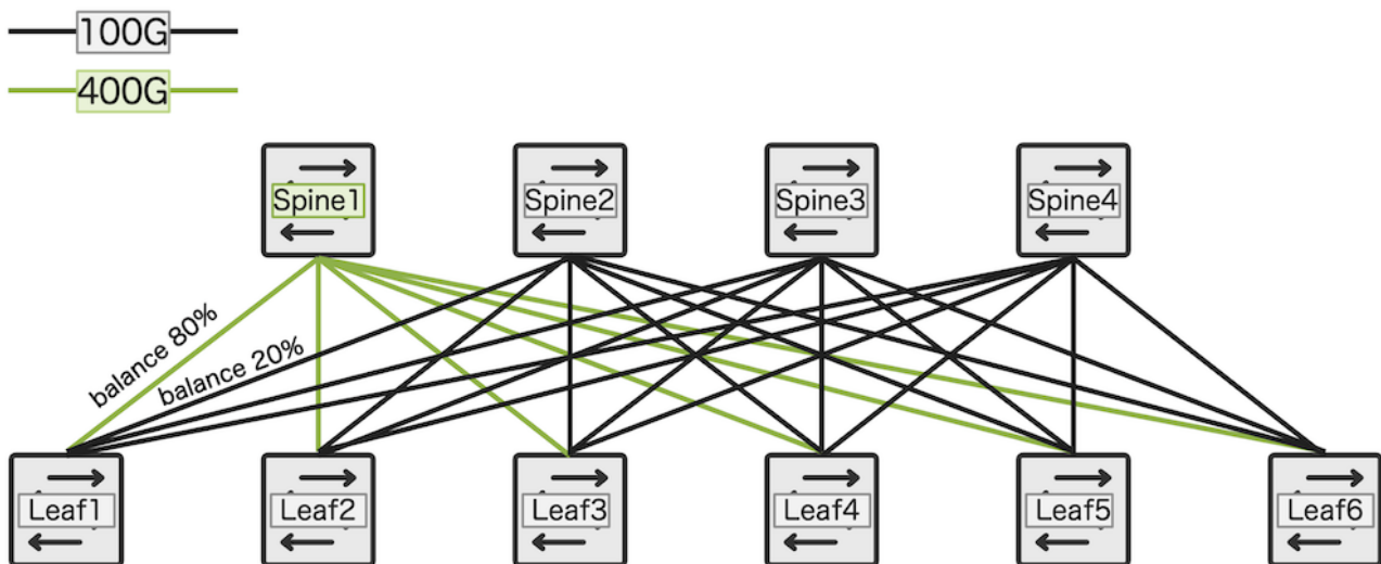
Figure 2: Leaf-Spine
