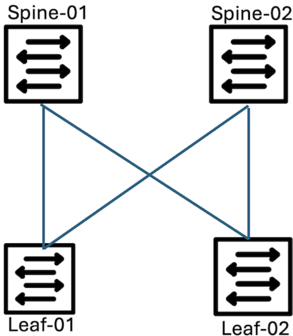
Figure 1: 3-CLOS Topology with a single link between leaf and spine
