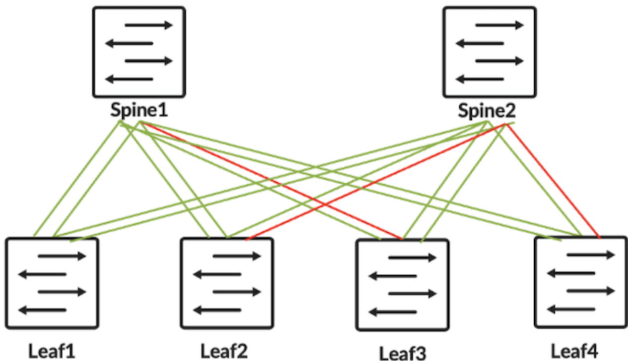
Figure 6: Multiple failures between different spine and leaf combinations
