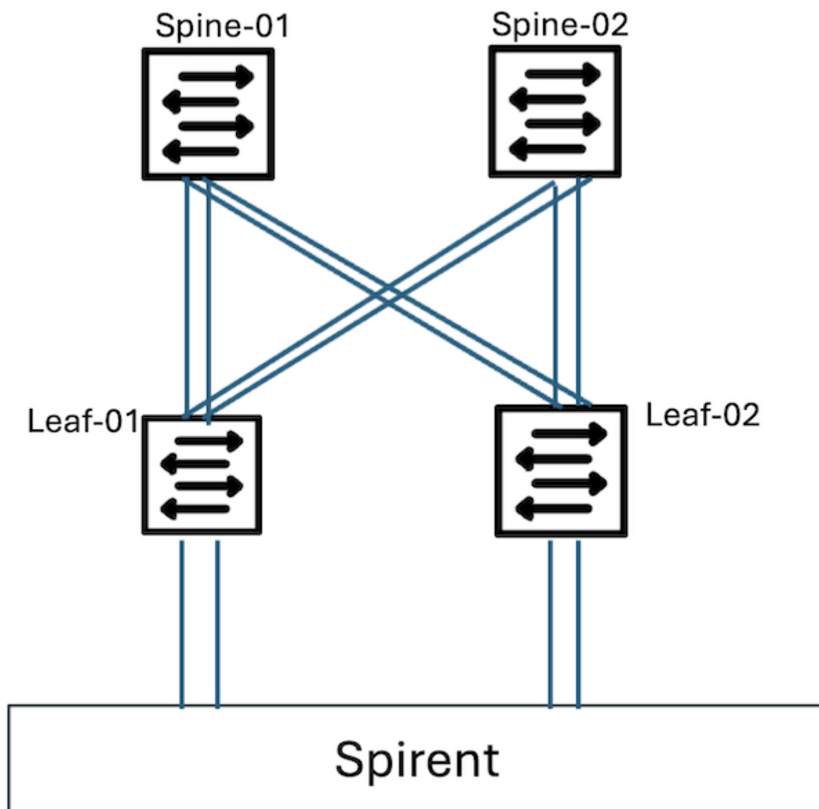
Figure 3: Lab Topology
