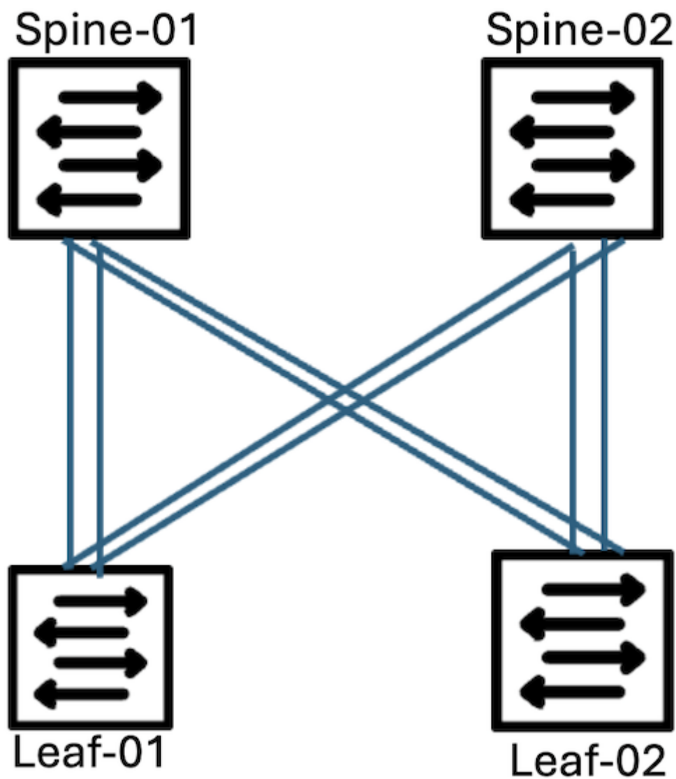
Figure 2: 3-CLOS Topology with multiple links between leaf and spine
