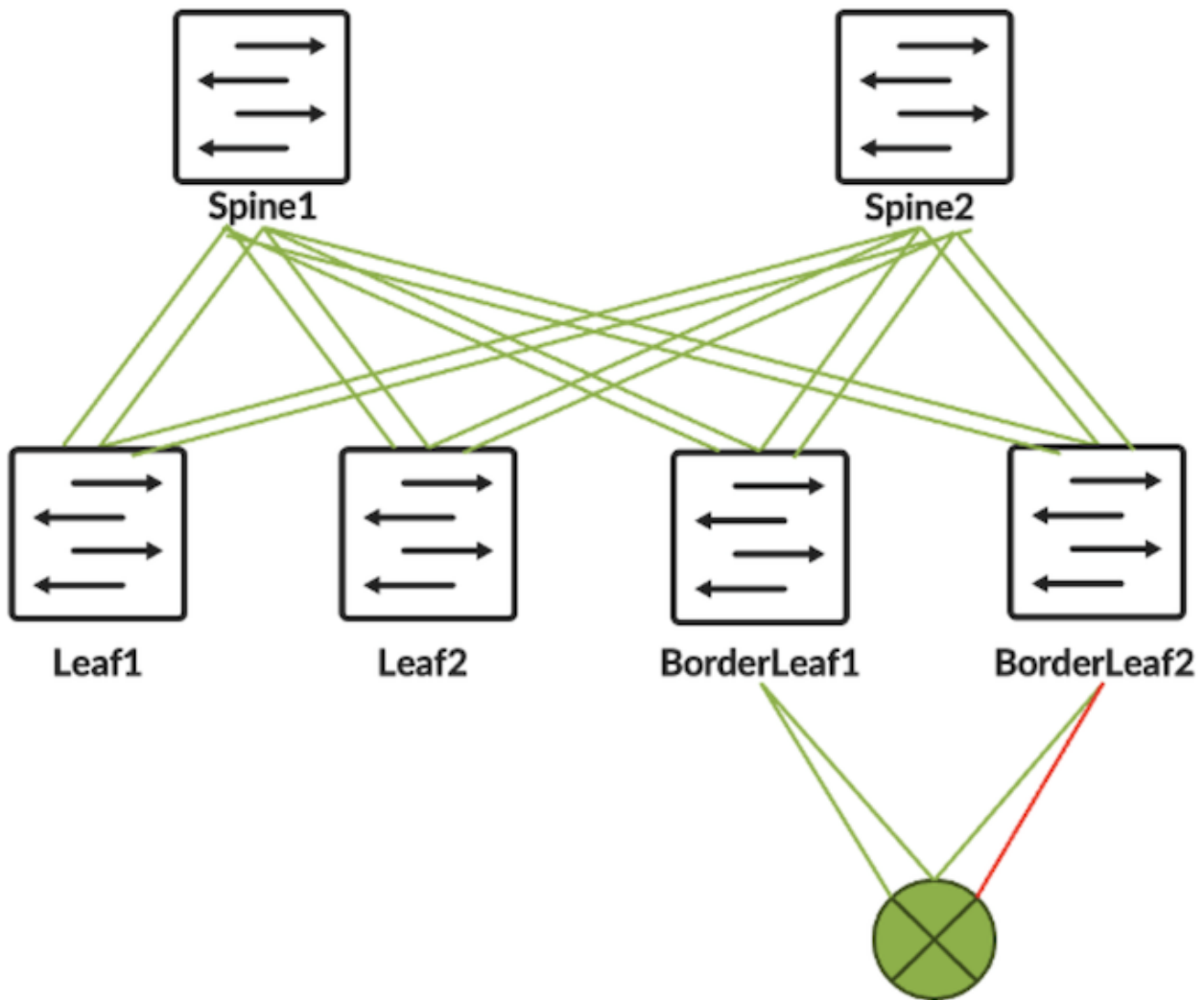
Figure 7: Topology with link failure between a border leaf and gateway
