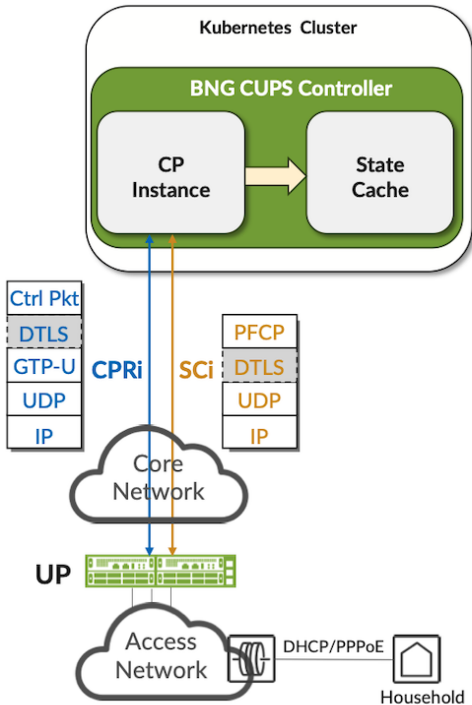
Figure 2: Juniper BNG CUPS Controller
