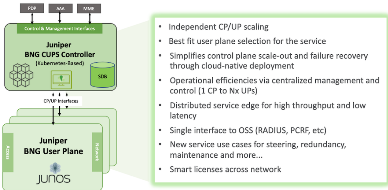
Figure 1: Juniper BNG CUPS Overview Architecture
