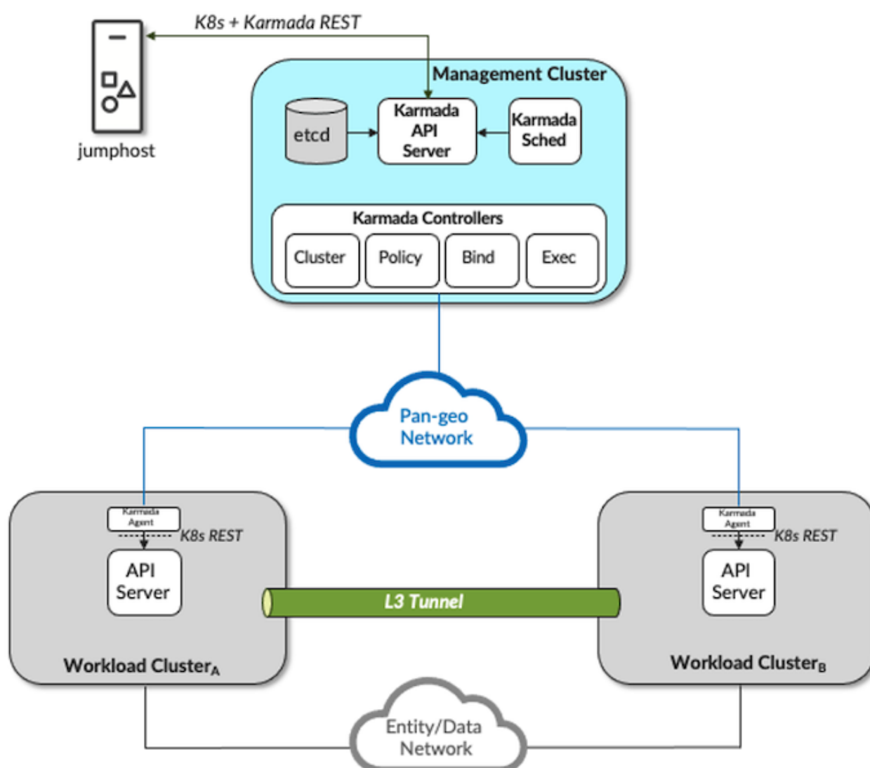
Figure 4: Karmada Multi-Cluster Logical Architecture
