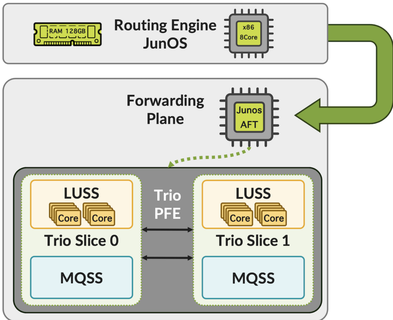
Figure 1: MX RE sends routes to the forwarding plane.
