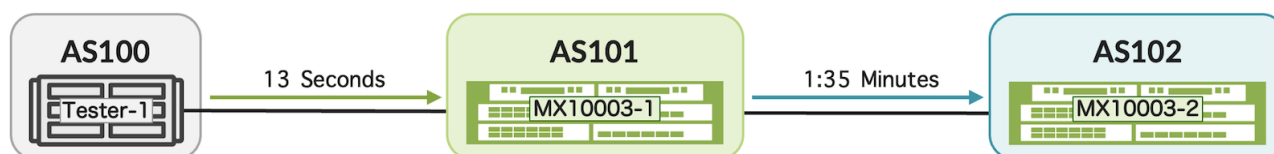
Figure 8: MX10003 with RIB sharding
