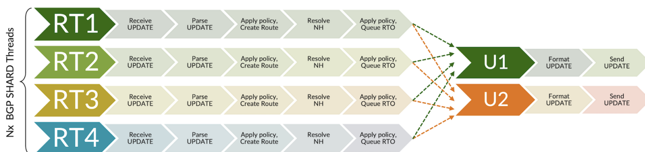
Figure 2: BGP RIB Sharding leverage multiprocessing
