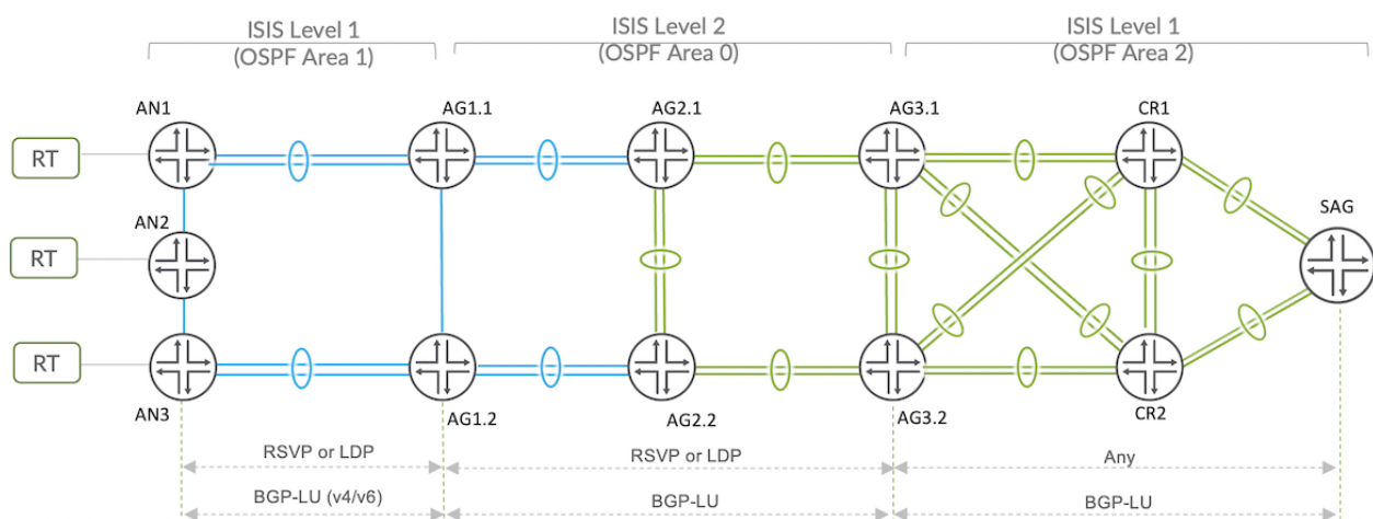
Figure 4: JVD Mobile Backhaul Transport
