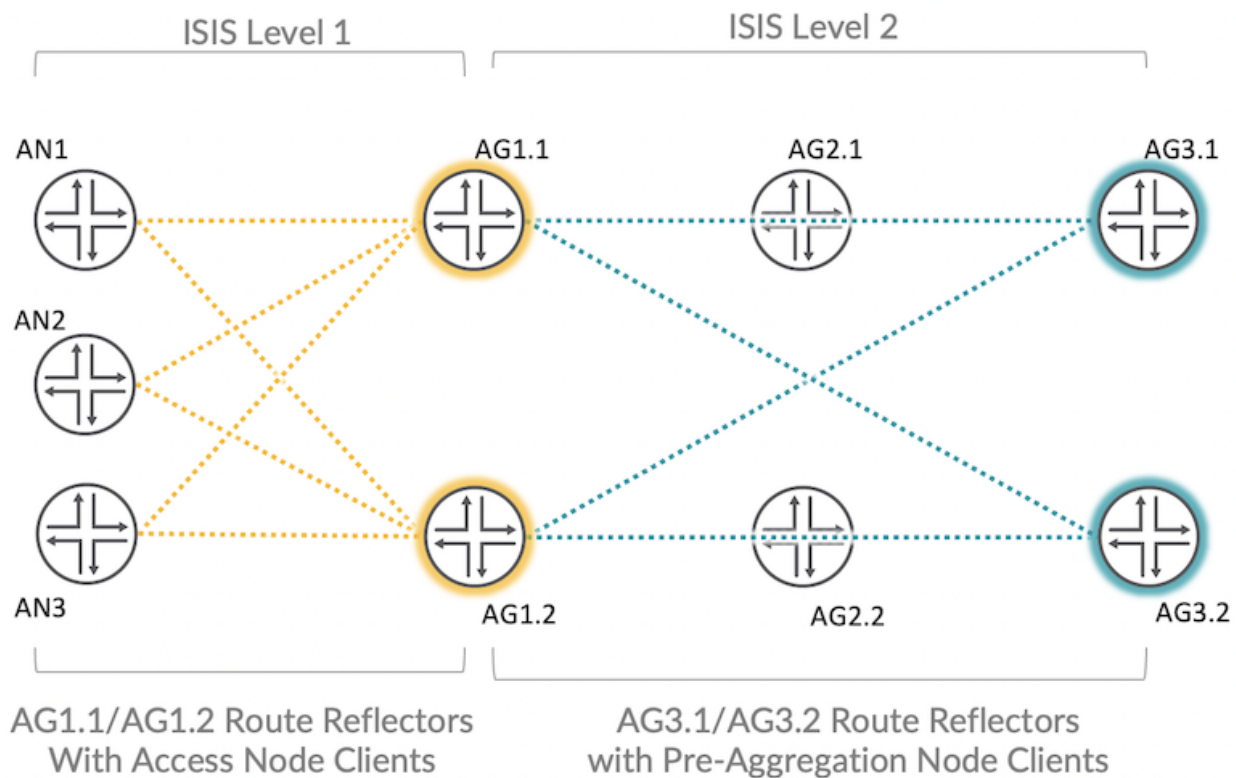
Figure 6: Redundant Route Reflector Design
