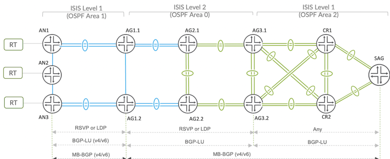
Figure 7: JVD Seamless MPLS Topology
