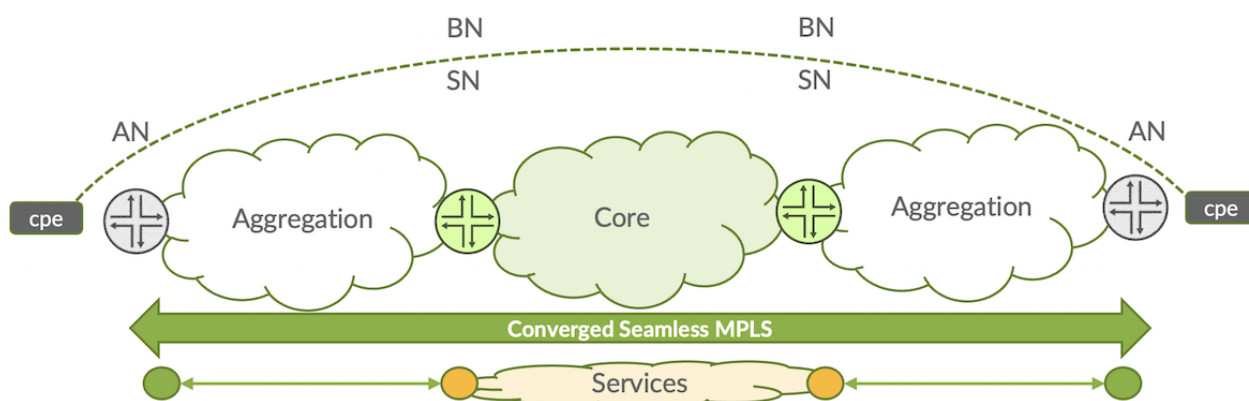
Figure 2: Seamless MPLS Domain
