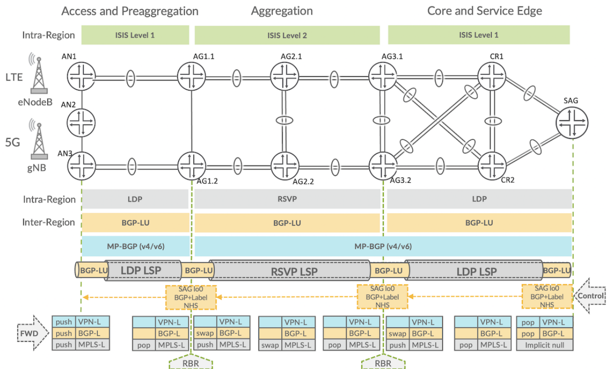
Figure 5: Multi-Region Seamless MPLS with BGP-LU
