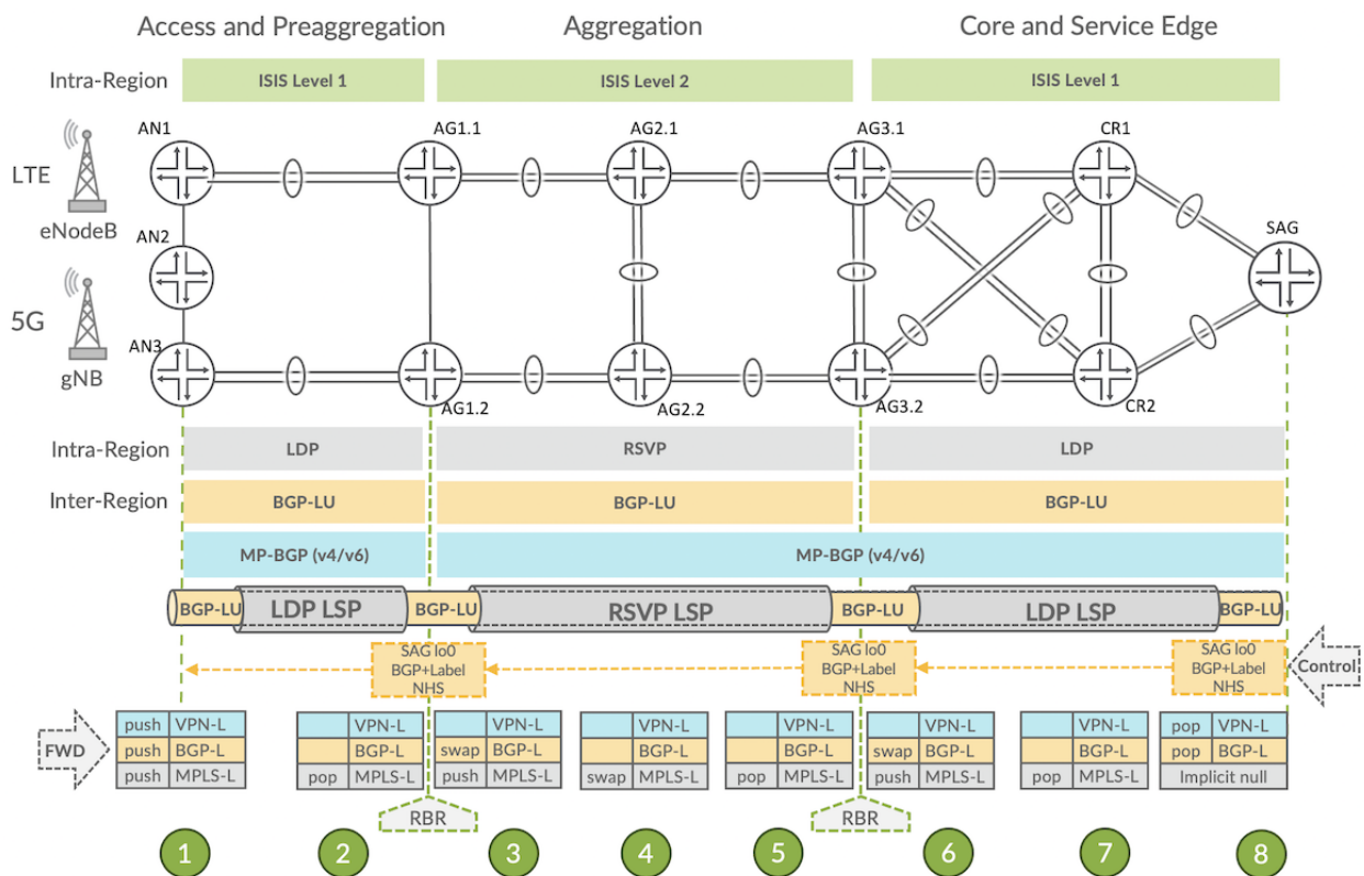
Figure 3: Seamless MPLS Label Operations
