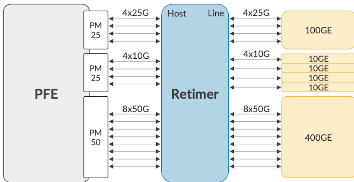
Figure 9: Retimer Example
