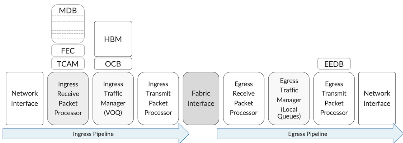
Figure 2: DNX ASICs Pipeline
