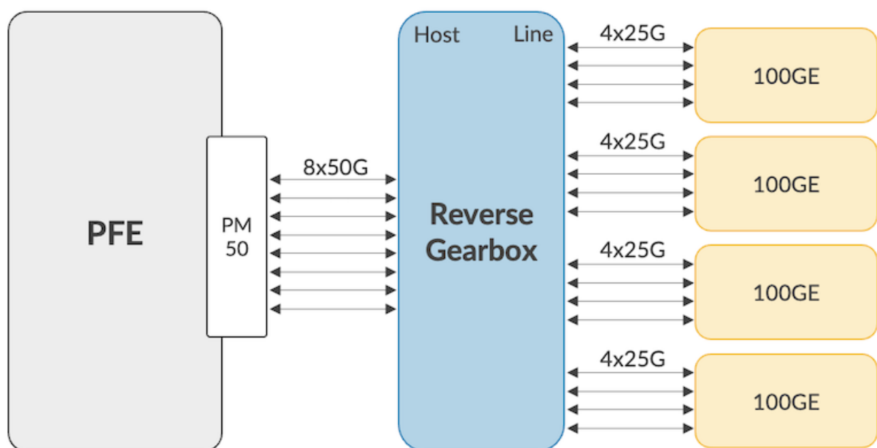
Figure 8: Reverse Gearbox Example
