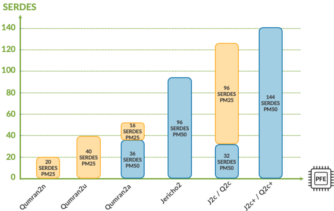
Figure 5: Port Macros association with NPUs
