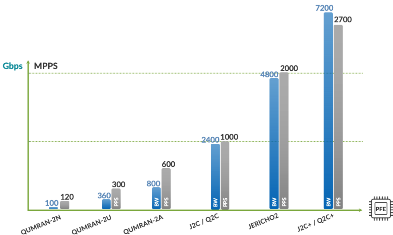
Figure 4: Jericho2's Generation NPUs
