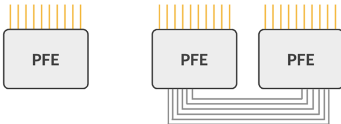
Figure 3: Standalone and Back-to-Back Modes
