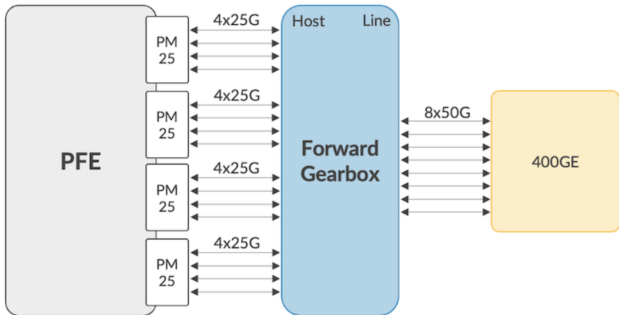
Figure 7: (Forward) Gearbox Example
