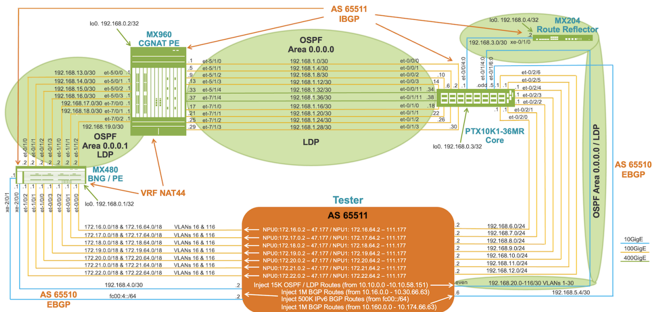
Figure 5: Scalability Topology
