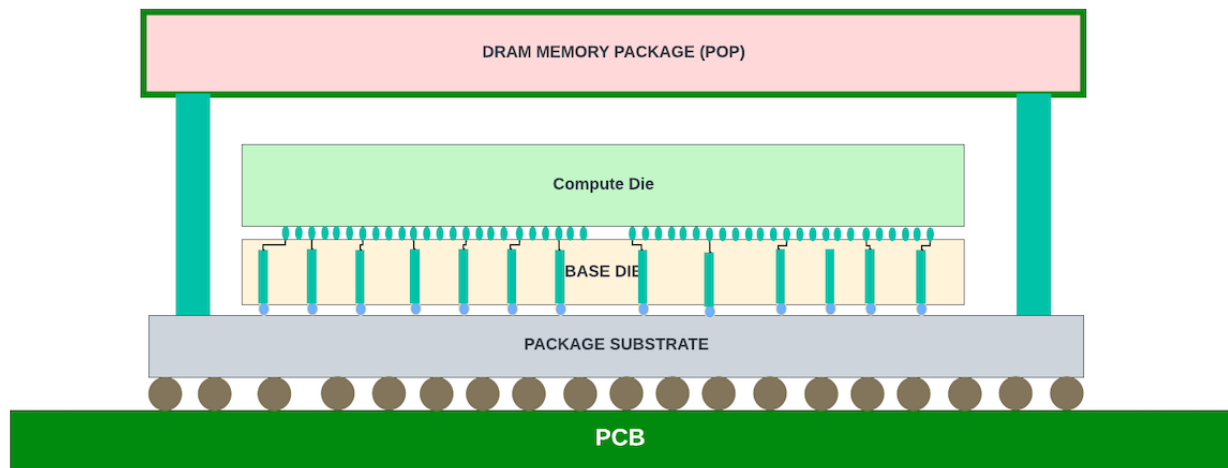
Figure 8: 3D Stacking between Base and Compute Dies and Package on Package (POP) DRAM
