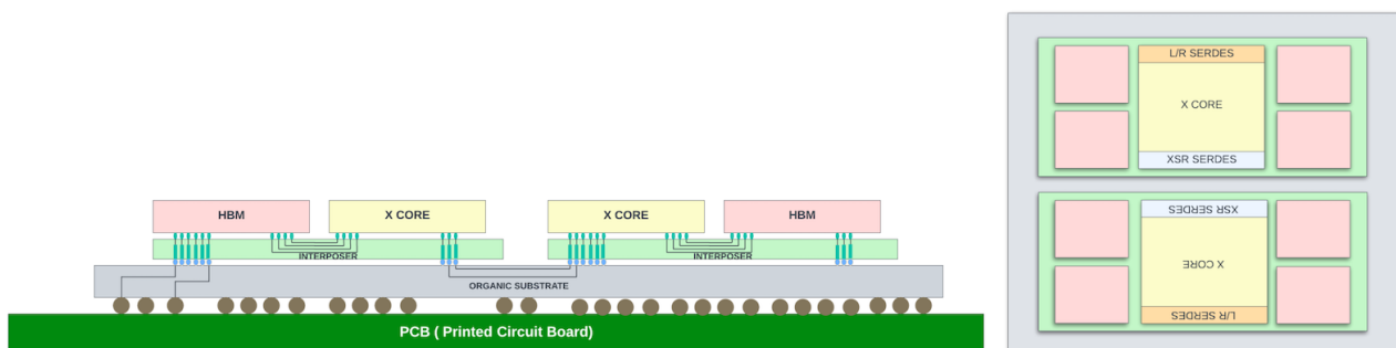
Figure 13: CoWoS with Silicon Interposer (S) Package used in Express 5 Silicon. The 28.8Tbps standalone switch ASIC
