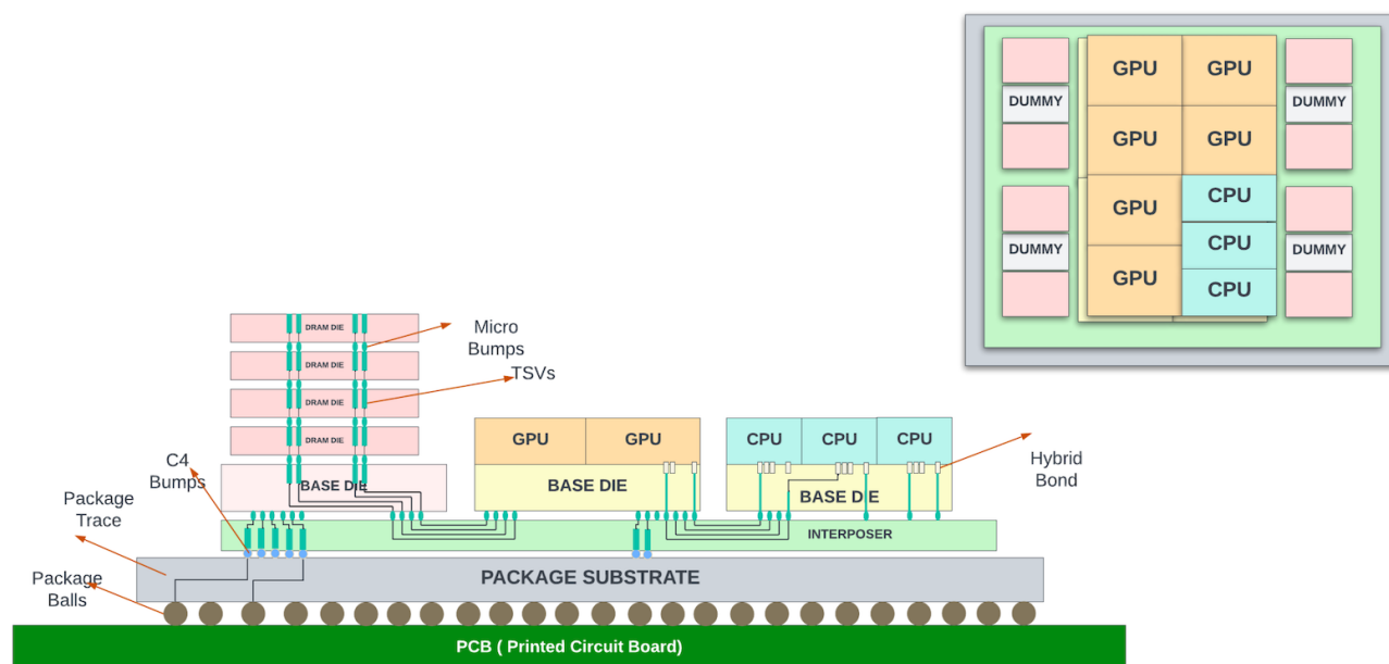
Figure 11: Advanced packaging with HBMs and 3D stacking of chiplets.
