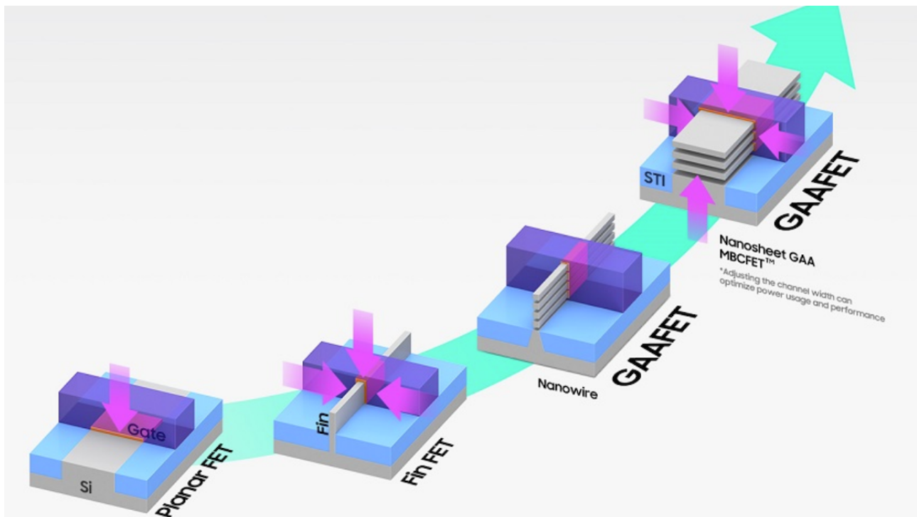
Figure 2: Various transistor technologies. Courtesy - Samsung Microelectronics.
