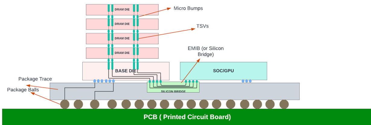
Figure 7: EMIB for HBM and Core Connectivity
