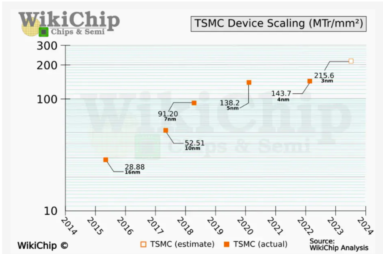
Figure 3: Transistor densities continue to increase with each process node.
