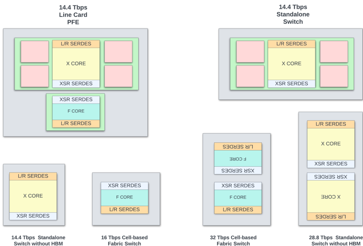
Figure 14: Two chiplets and the many packages.
