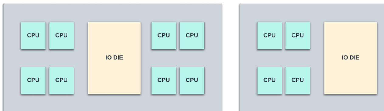
Figure 6: Illustration of Zen2 MCMs with IO dies
