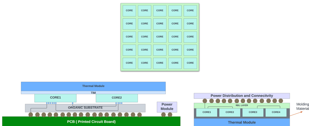
Figure 12: Integrated Fan-Out (INFO) System on a Wafer (SOW) Technology
