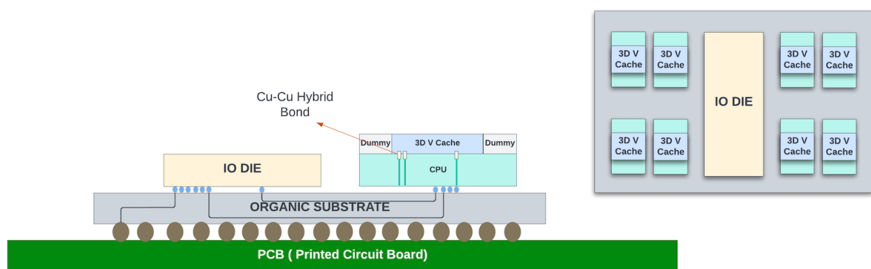
Figure 10: Cu-Cu Hybrid Bonding between the chiplets stacked in the vertical Direction
