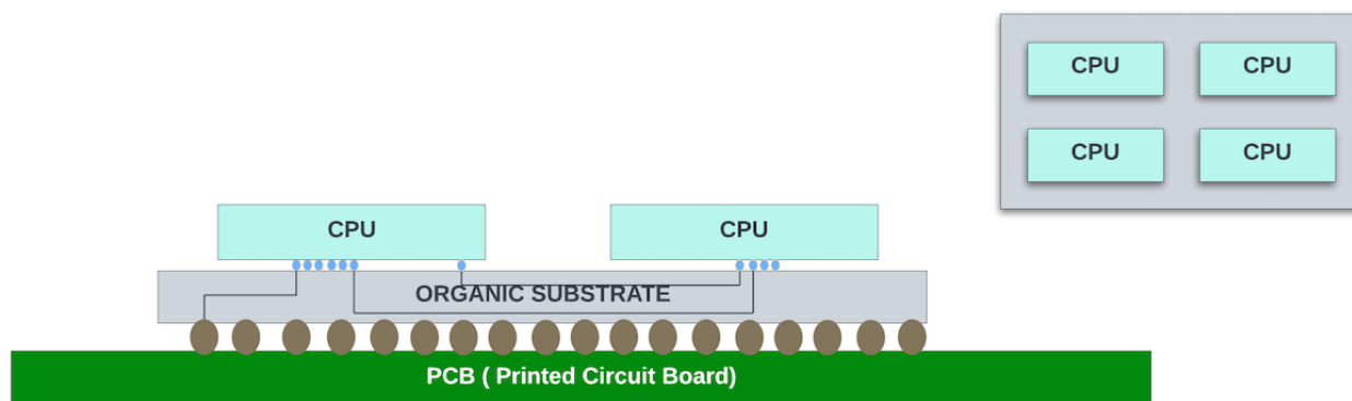
Figure 5: Multi-Chip Module (MCM) with four CPU dies.
