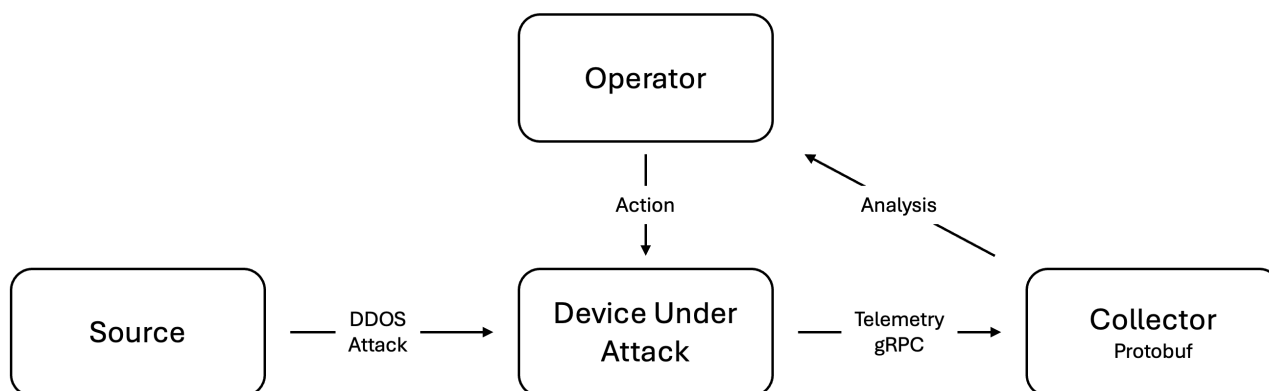
Figure 2: DDOS-Attack-Triggered-Packet-Capture
