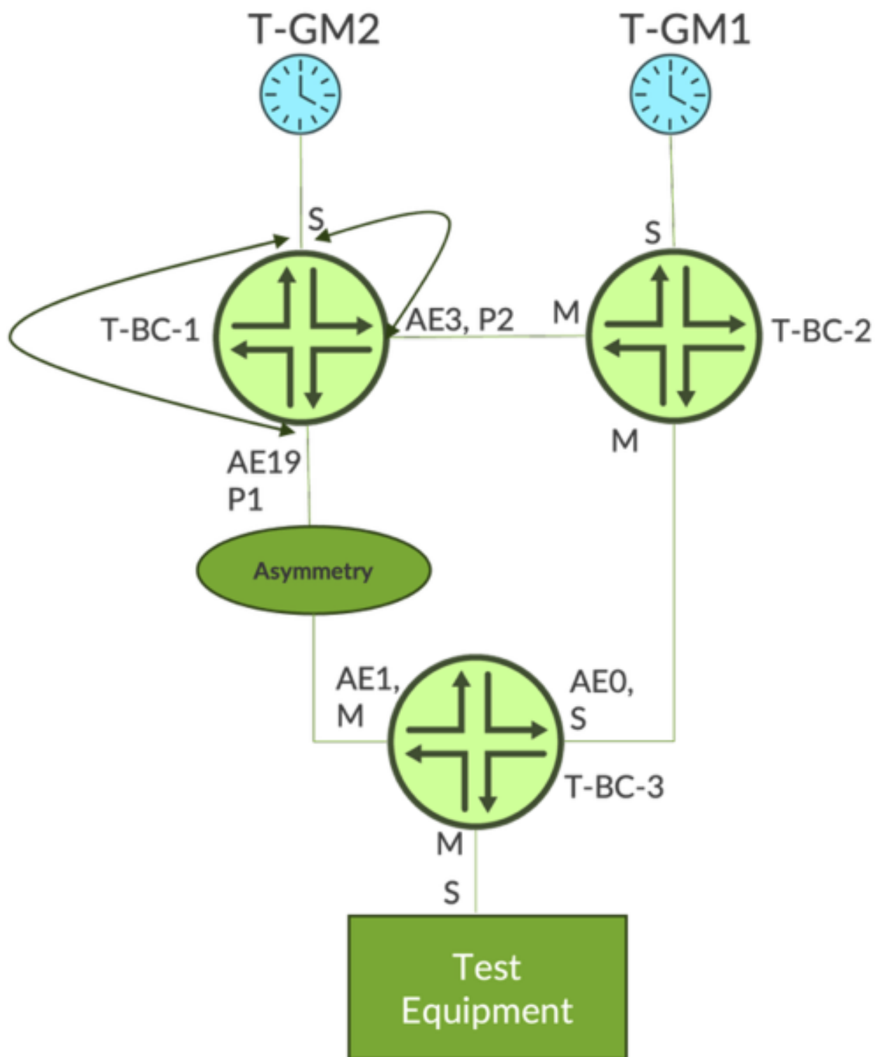
Figure 3: The topology model used by the EMEA Service Provider for the PPM feature
