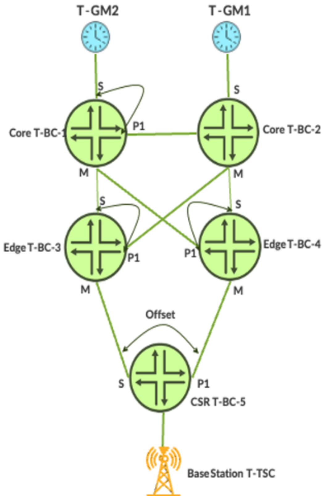
Figure 2: The synchronization network monitoring using PPM feature
