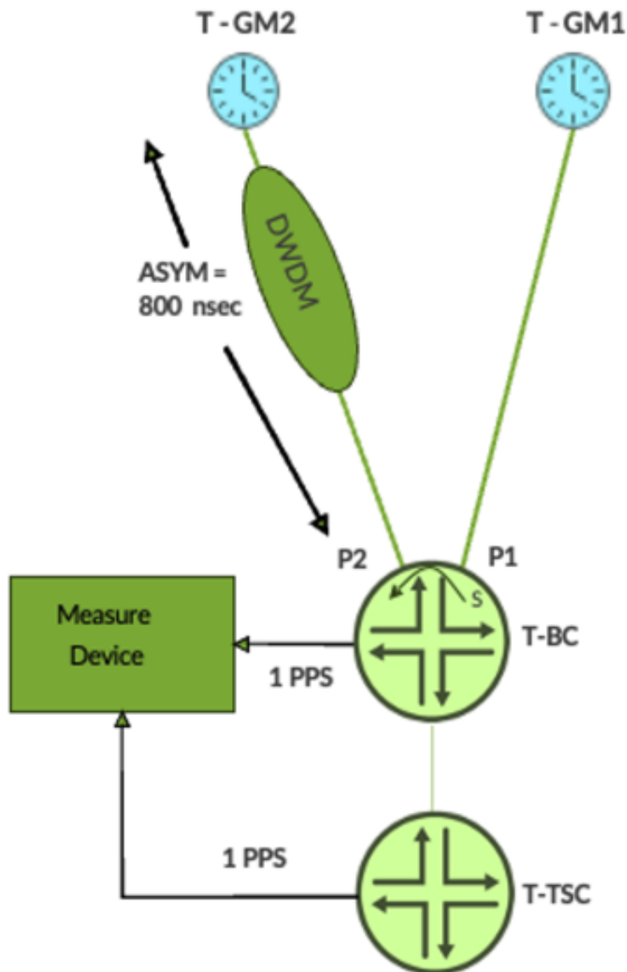
Figure 1: Figure-1: PPM for Provisioning
