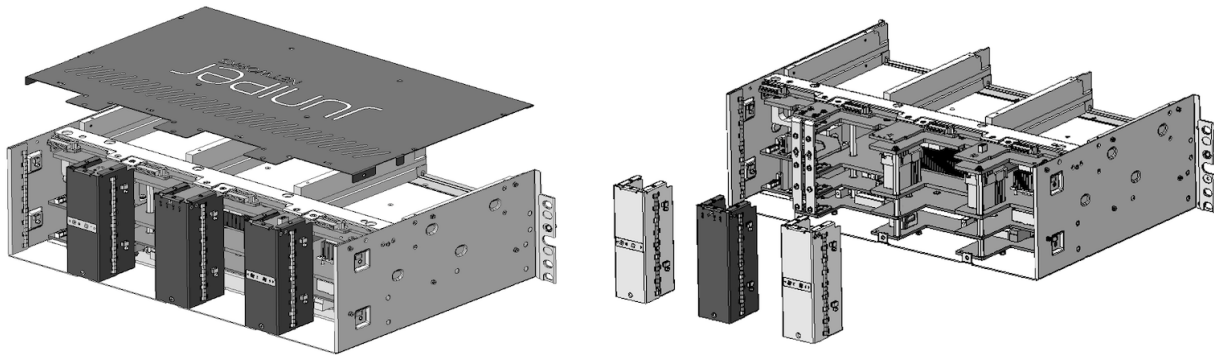
Figure 6: ACX7348 Hardware View
