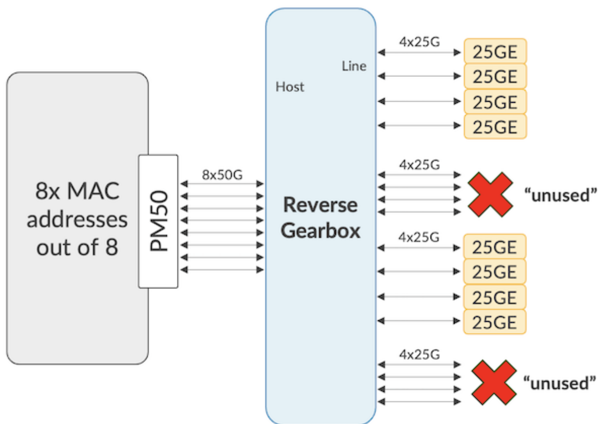
Figure 16: Use of Break-out Cables Behind a RGB
