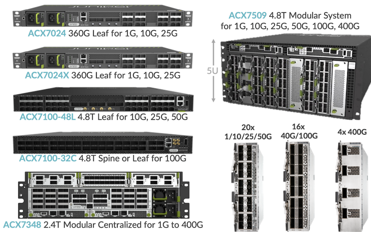
Figure 2: ACX7000 Family in Detail
