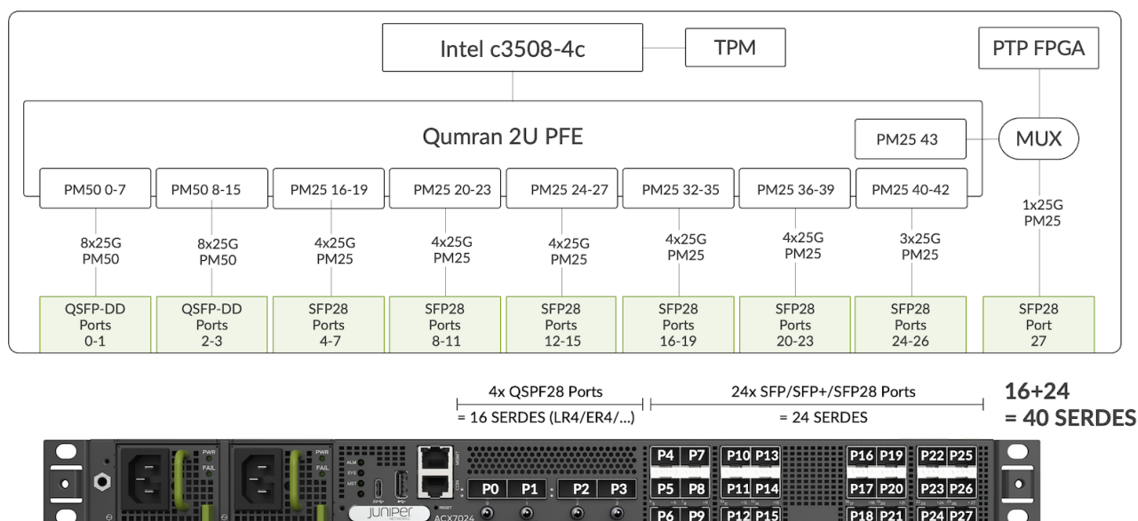
Figure 13: ACX7024 Block Diagram
