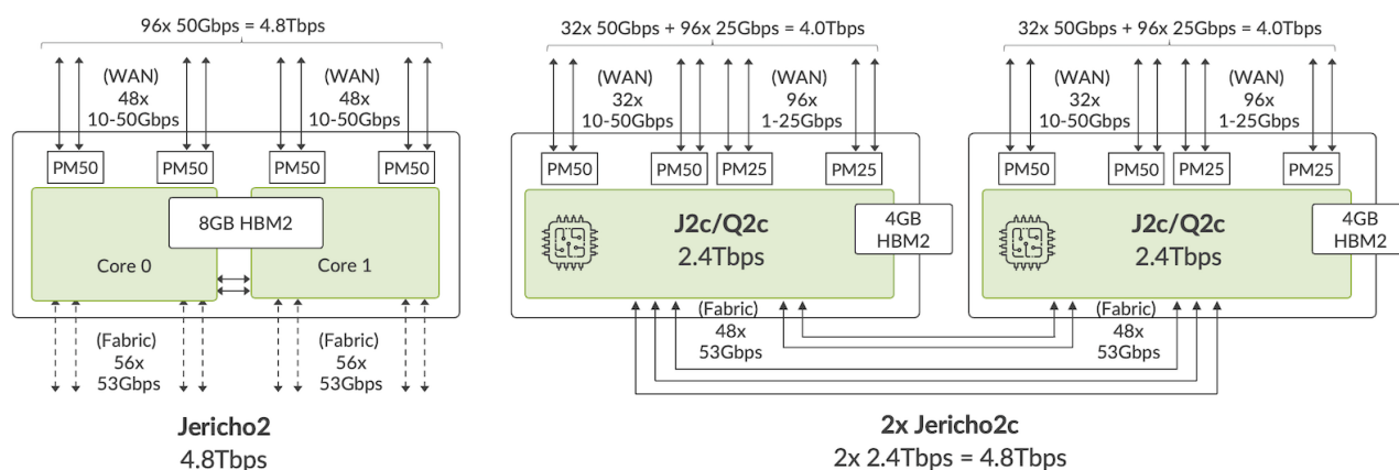
Figure 14: J2 or 2x J2c Back-to-Back
