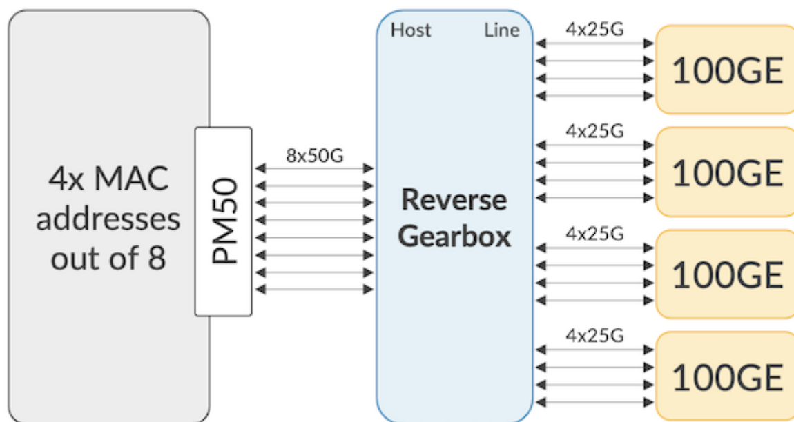
Figure 15: Fanout with a Reverse GearBox
