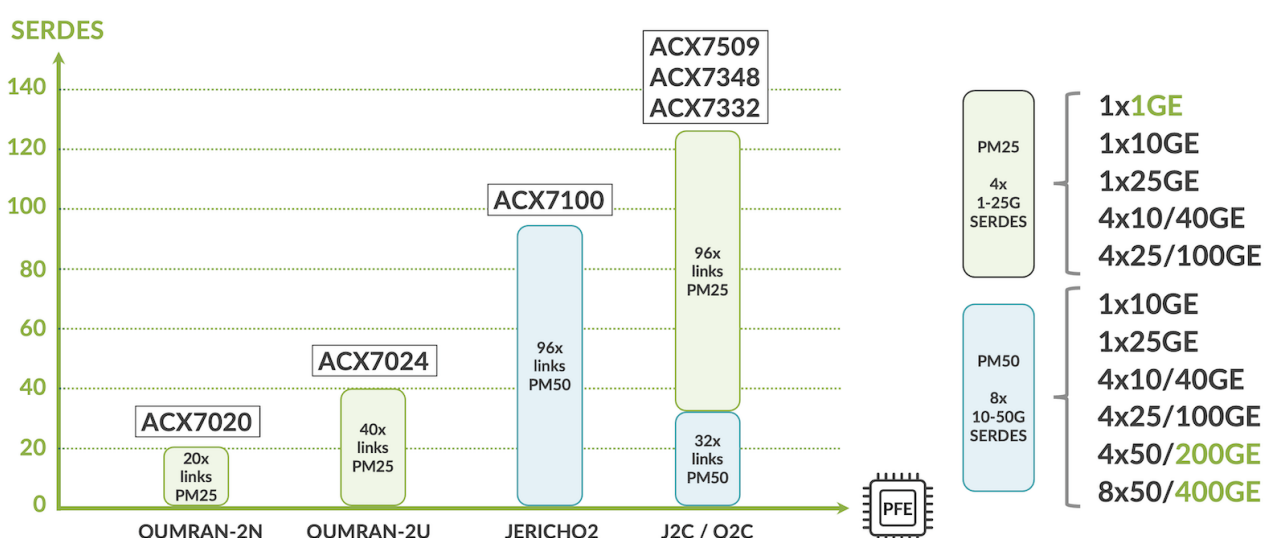
Figure 12: PFEs SerDes and PortMacros
