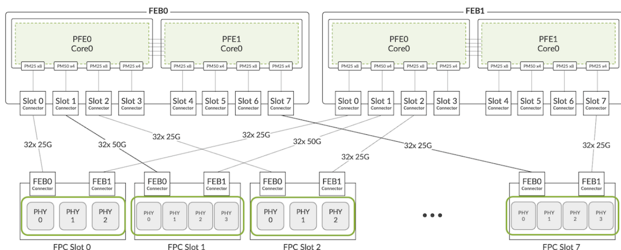
Figure 17: Example of ACX7509 with FPC Connectors and Retimers
