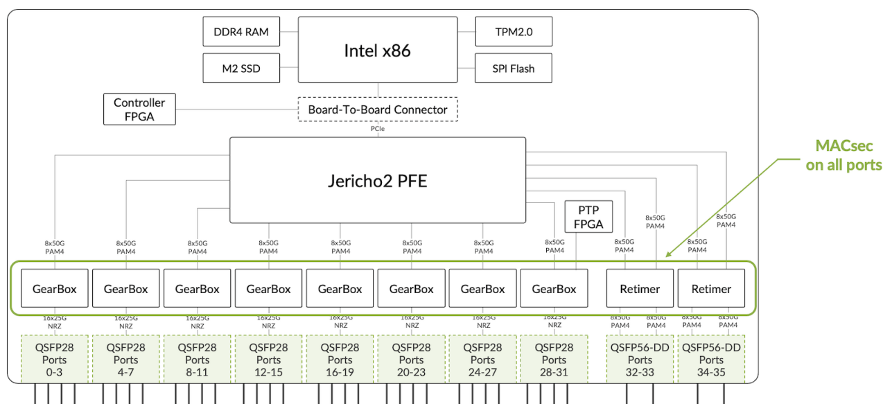
Figure 18: PHY in the ACX7100-32C for MACsec
