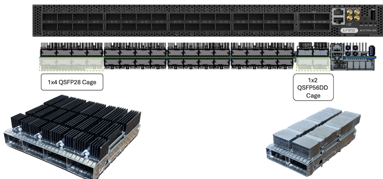
Figure 9: Example of Belly-to-Belly Design on ACX7100
