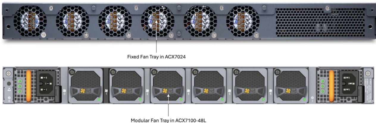
Figure 8: Fixed Fan Blocks in ACX7024 and Field Replaceable Fans in ACX7100
