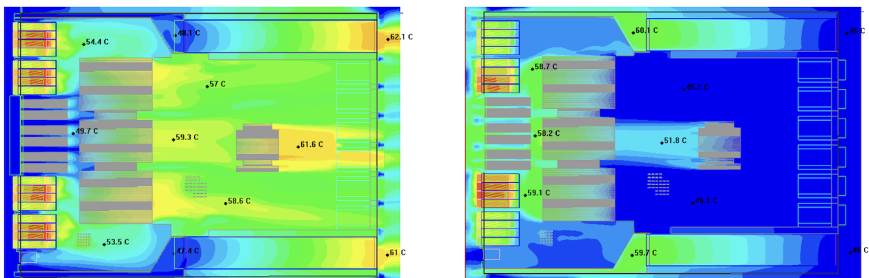
Figure 7: ACX7100-48L Back-to-Front and Front-to-Back Cooling Temperatures
