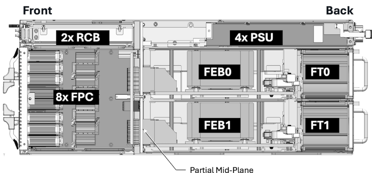
Figure 5: ACX7509 Side View
