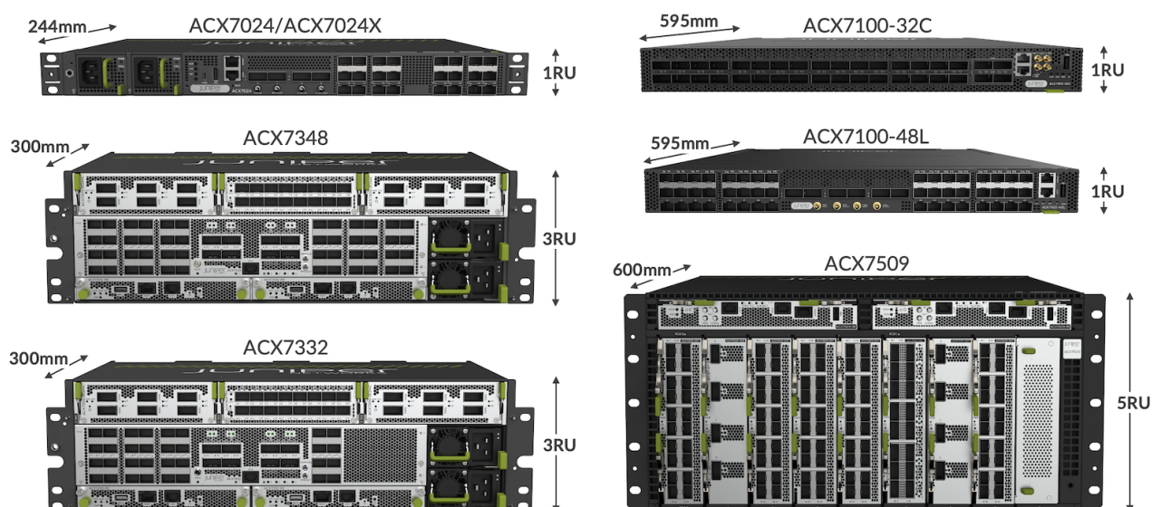
Figure 4: Metal-to-Metal Dimensions of ACX7000 Routers
