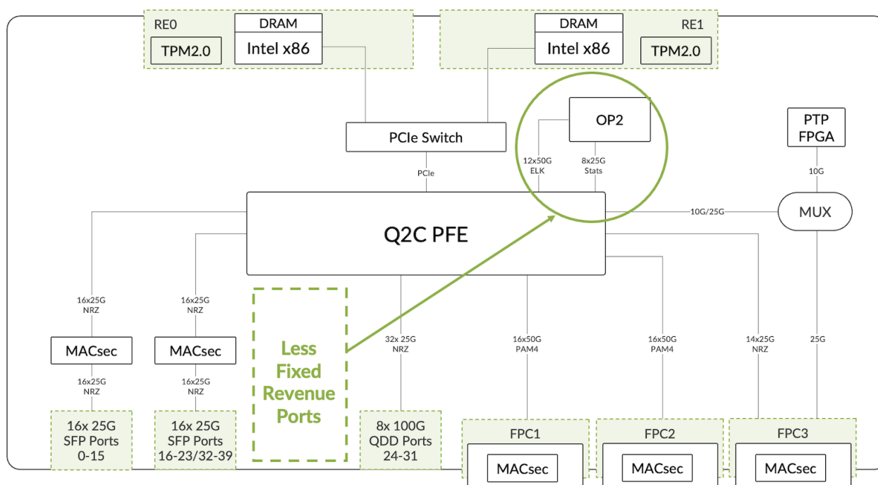
Figure 21: ACX7332 Block Diagram with OP2 eTCAM
