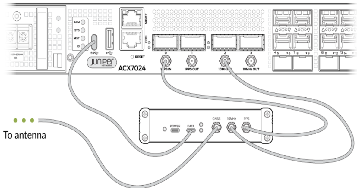
Figure 19: ACX7024 with TB1 Connections
