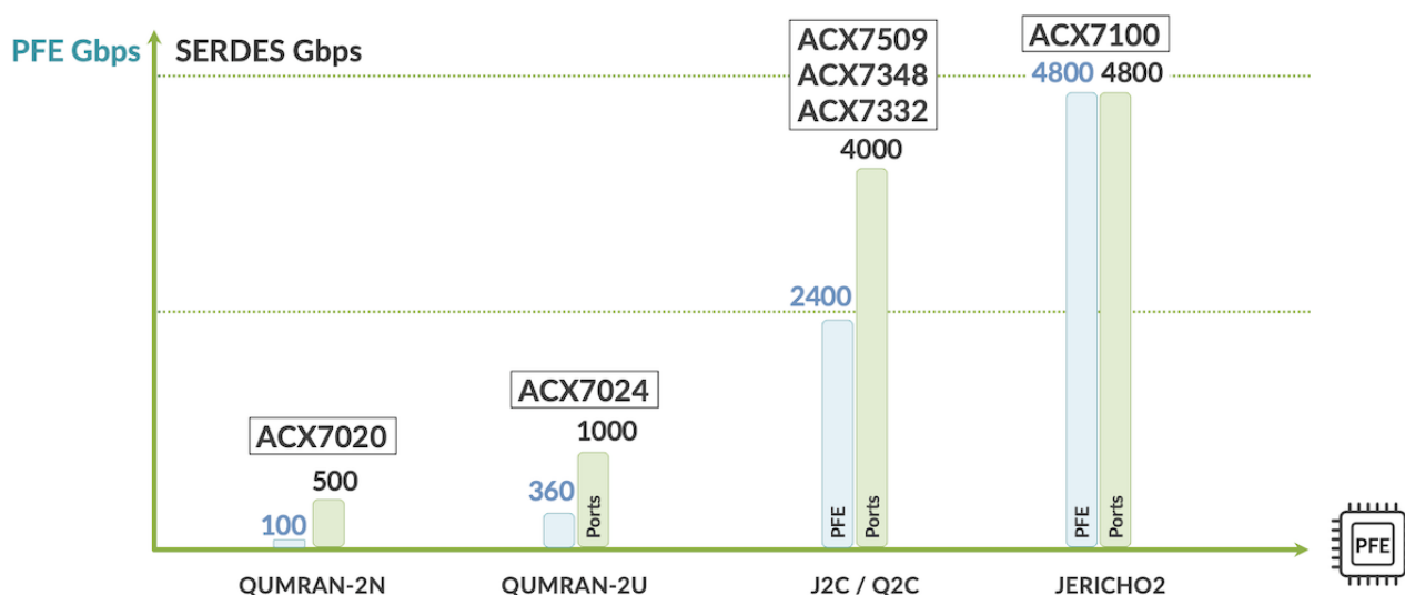
Figure 11: J2 PFEs OverSubscription
