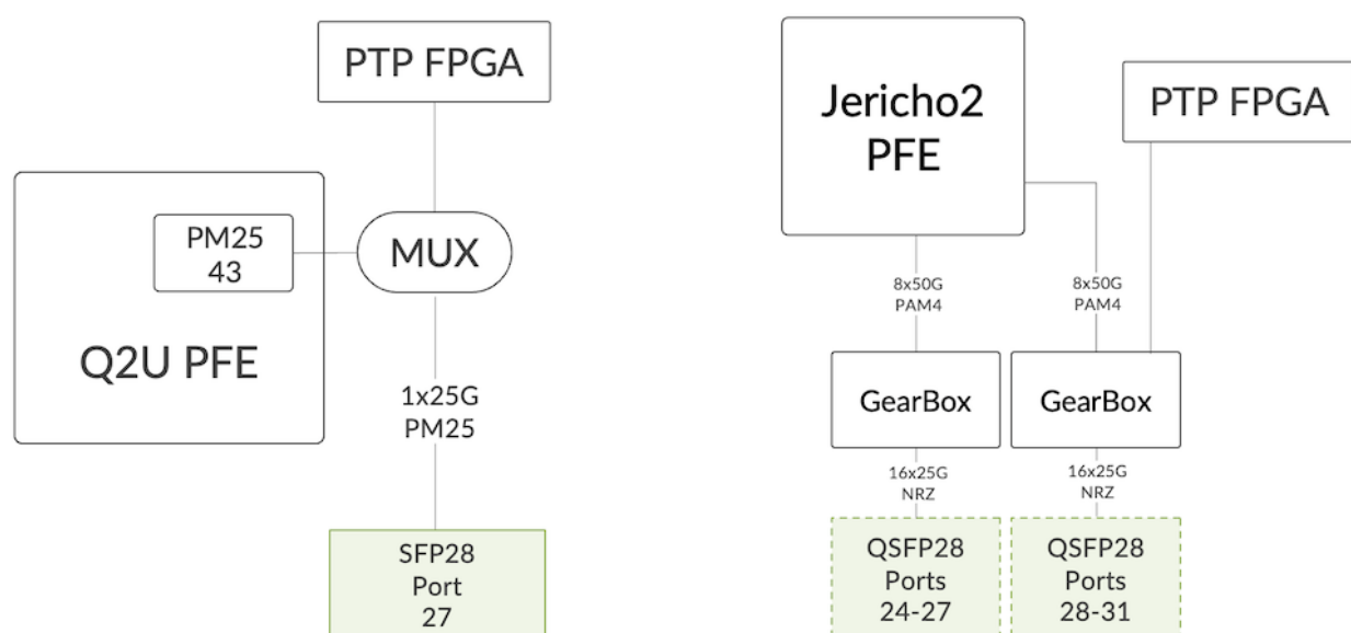
Figure 20: PTP FPGA in ACX7024 and ACX7100
