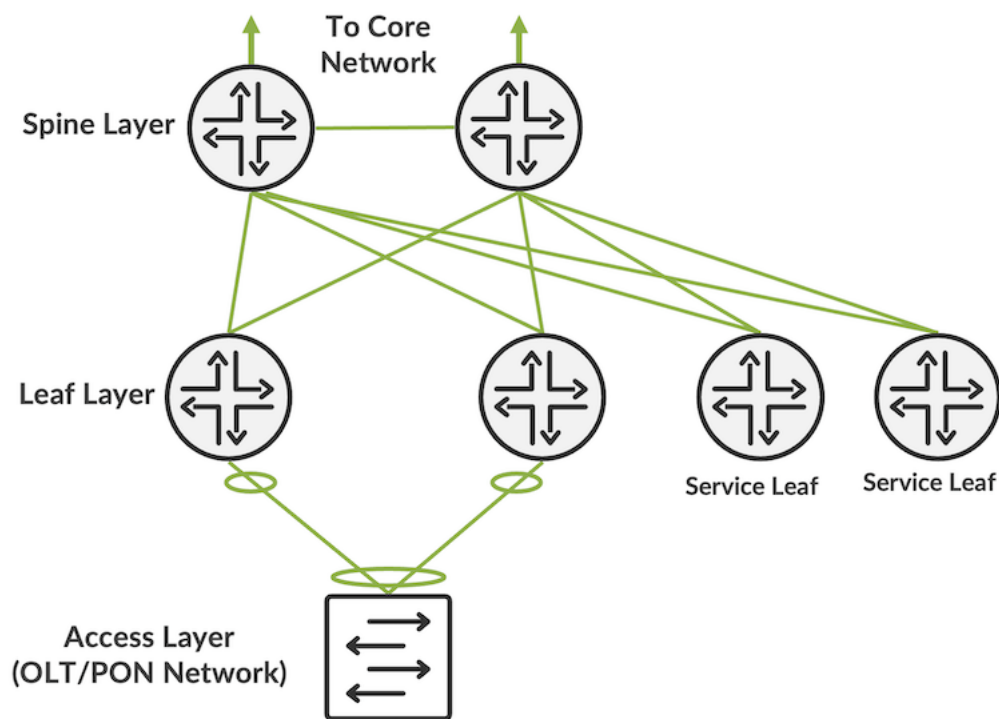
Figure 1: Spine/Leaf Architecture with dedicated Service Leaf
