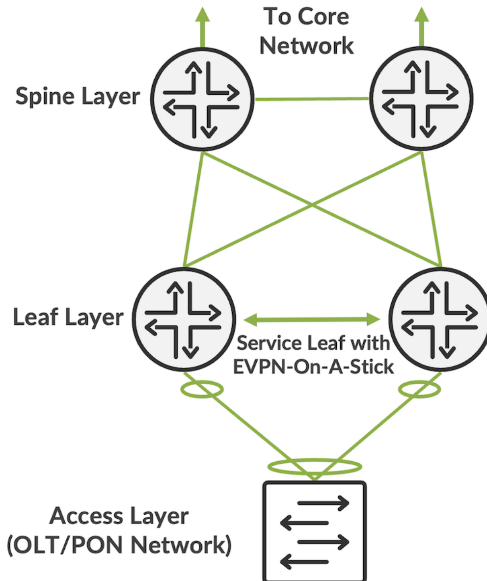
Figure 2: EVPN-On-A-Stick Spine/Leaf Architecture
