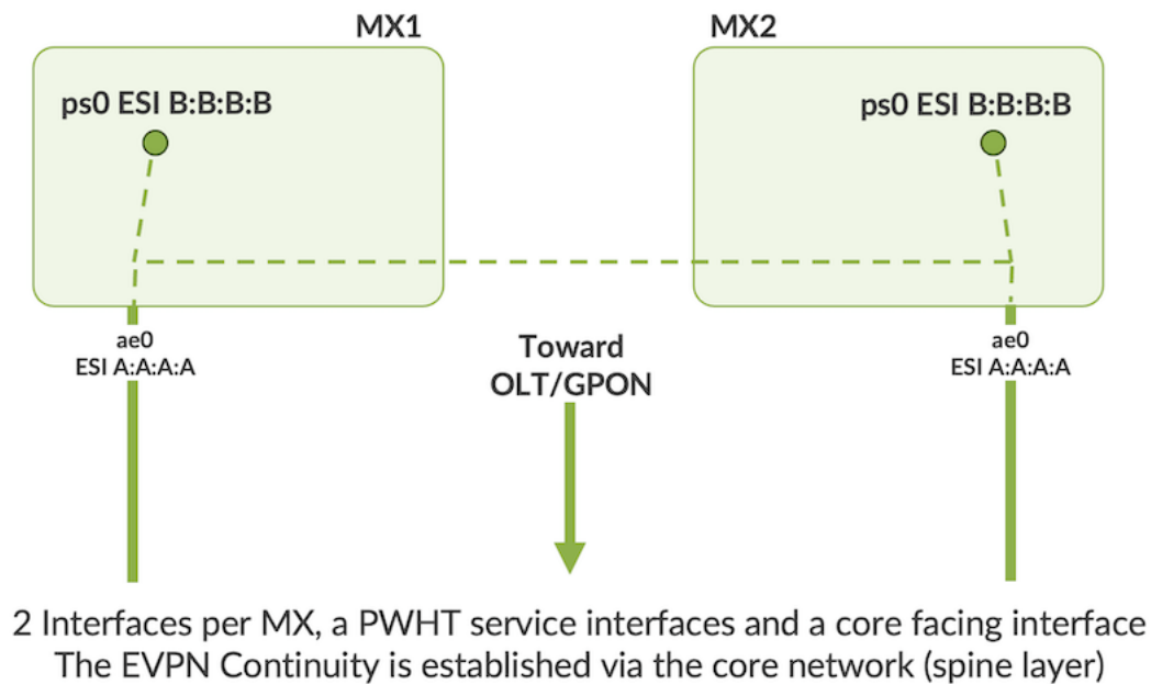
Figure 3: EVPN-On-A-Stick Access and Service interfaces on each MX
